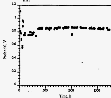
Fig. 4. Cell potential vs time of MCFC test cell containing Material 1 cathode.
