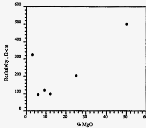
Fig. 2. Effect of MgO concentration on resistivity of \text{LiFeO}_2 at 650^\circ\text{C} in air.
