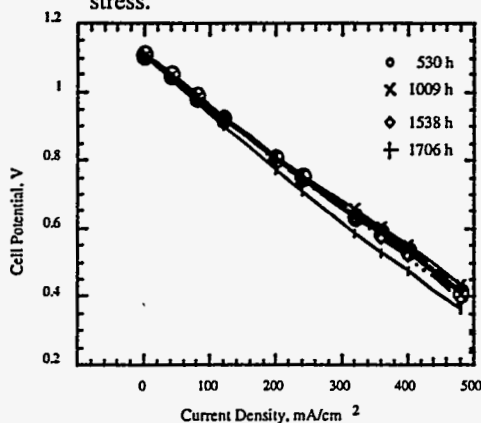
Fig. 5. Changes in polarization curves vs time of MCFC test cell containing Material 1 cathode.
