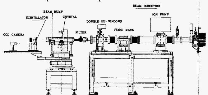
Figure 2: Schematics of the experimental setup for beam divergence measurement.
