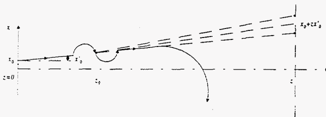
Figure 1: Schematics showing the undulator radiation cone from an off-axis particle: solid line is the particle trajectory and dashed line is the cone of undulator radiation.
