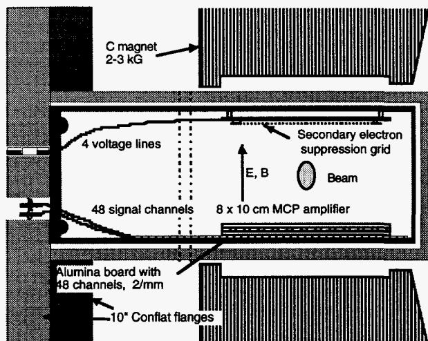
Figure 1. Cross section of IPM. View is looking down the beamline. In this experiment the orientation was rotated 90° CW so the detector mounting flange was horizontal.
