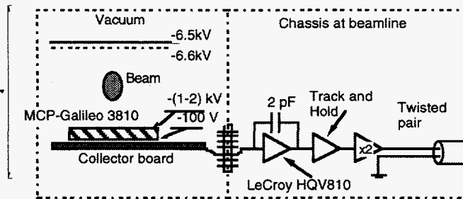
Figure 2. Schematic of the electronics in the tunnel. The trigger signal for the track-and-hold is generated by a digital delay generator in the instrument racks.
