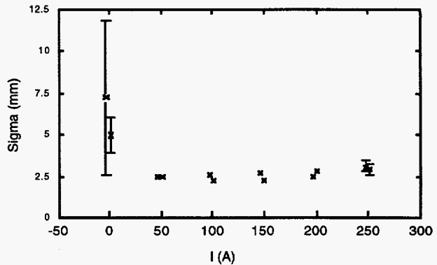
Figure 5. Beam width (sigma) from Gaussian fit to IPM data plotted vs. magnet current. Field is about 0.1T/50A.
