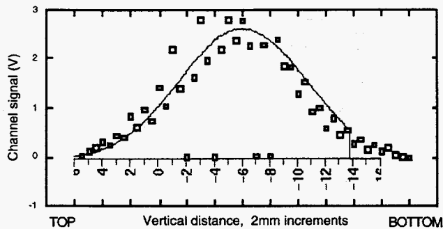
Figure 3. A Gaussian fit to the fluorescent screen profile, solid curve, overlaid the data collected from the IPM. The screen was located 2m downstream and the beam was diverging.
