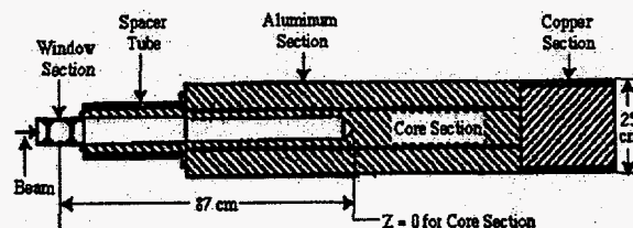
FIGURE 2. Cross sectional view of the commissioning and tune-up dump.
