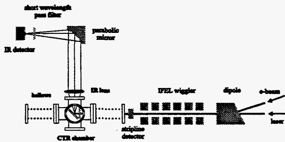
Figure 2: Schematic of the micro-bunching diagnostic setup for the IFEL experiment.
