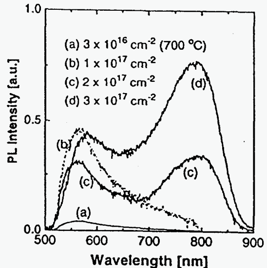
Fig.1. PL intensity for samples implanted at different doses and annealed 30 min. at 1000^\circ\text{C} .
