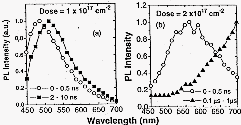
Fig.4 Nanosecond time-resolved gated spectra for samples implanted at 1 \times 10^{17} (a), and 2 \times 10^{17} \text{ cm}^{-2} and annealed at 1000 \text{ }^\circ\text{C} .
