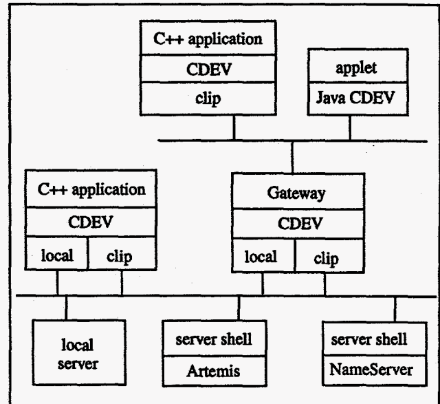
Figure 2: CDEV network components, showing logical network connections for two protocols, with gateway connected applets and applications.
