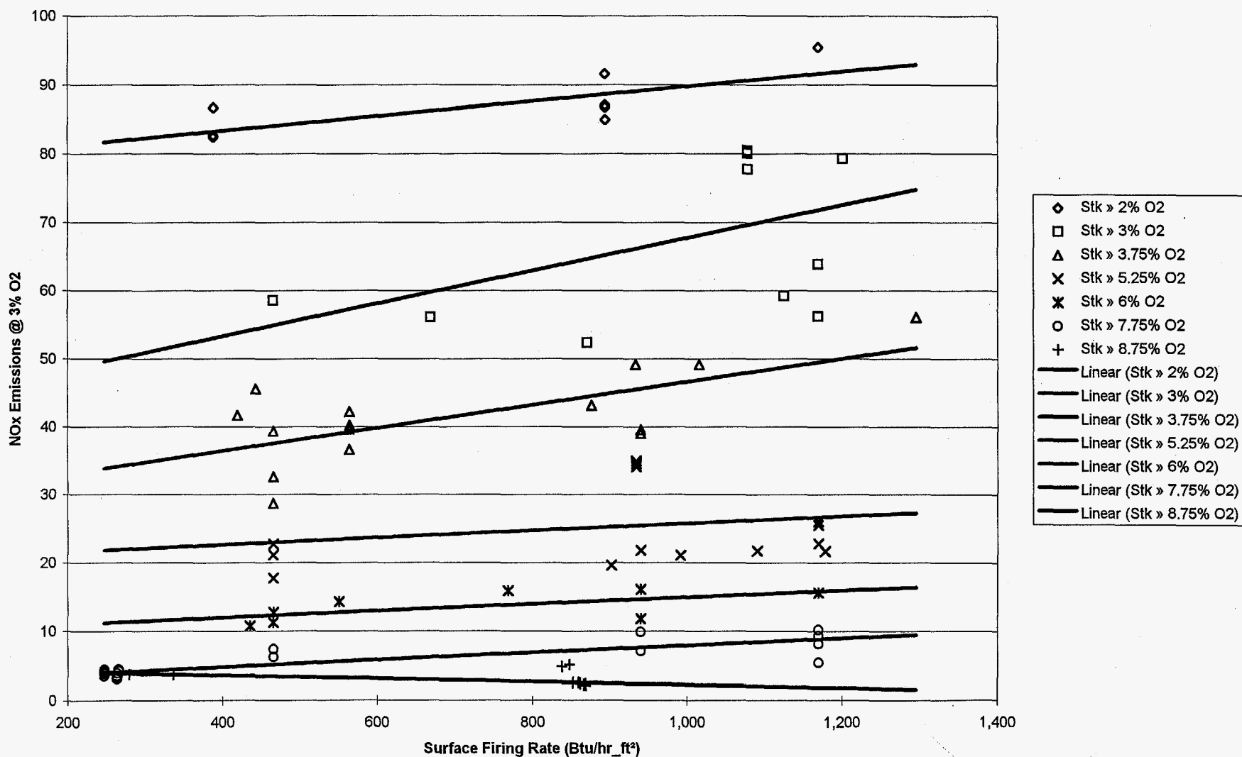
Figure 2-3. Excess Air Curve in Unilux Boiler
