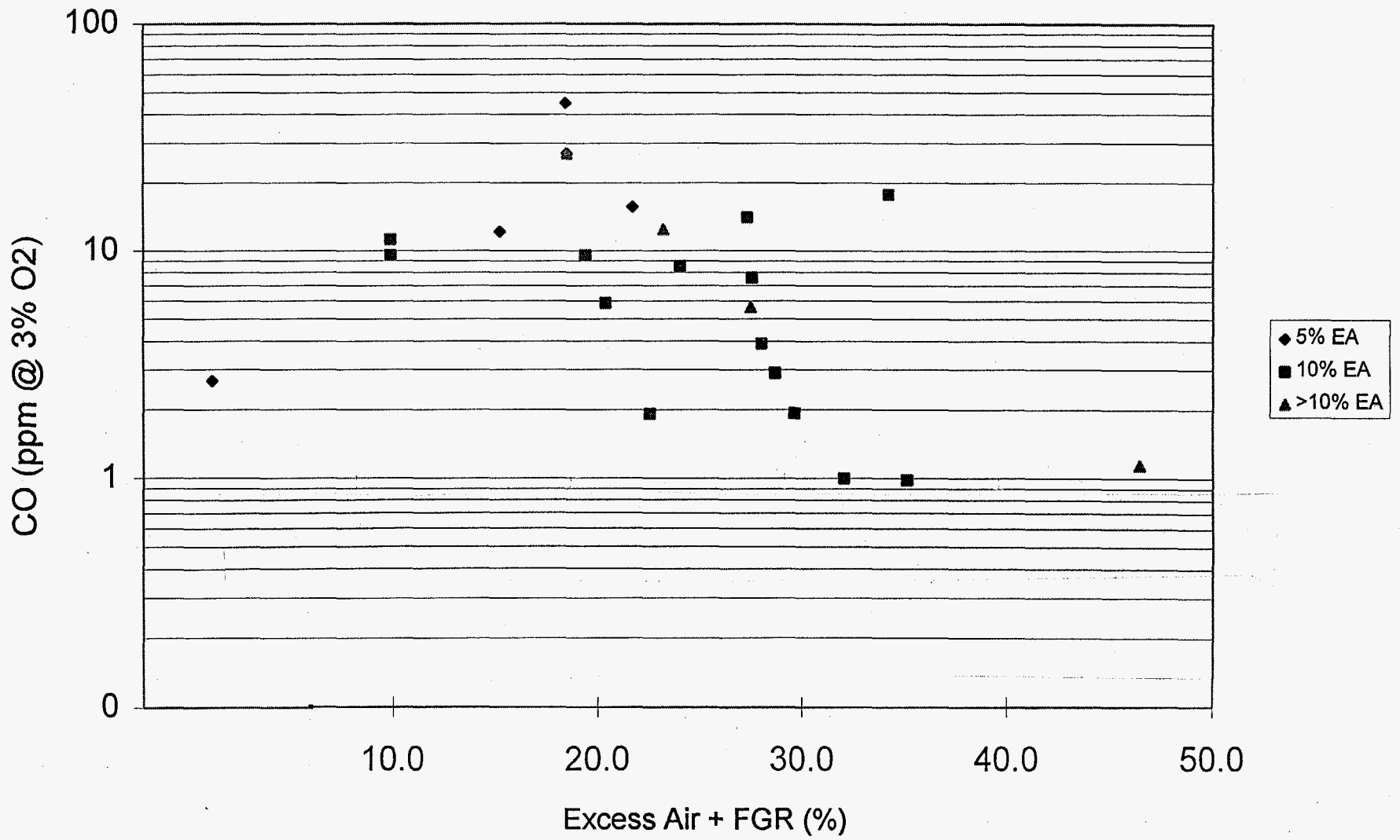
Figure 2-11. CO vs. Excess Air Plus FGR in Unilux Boiler
