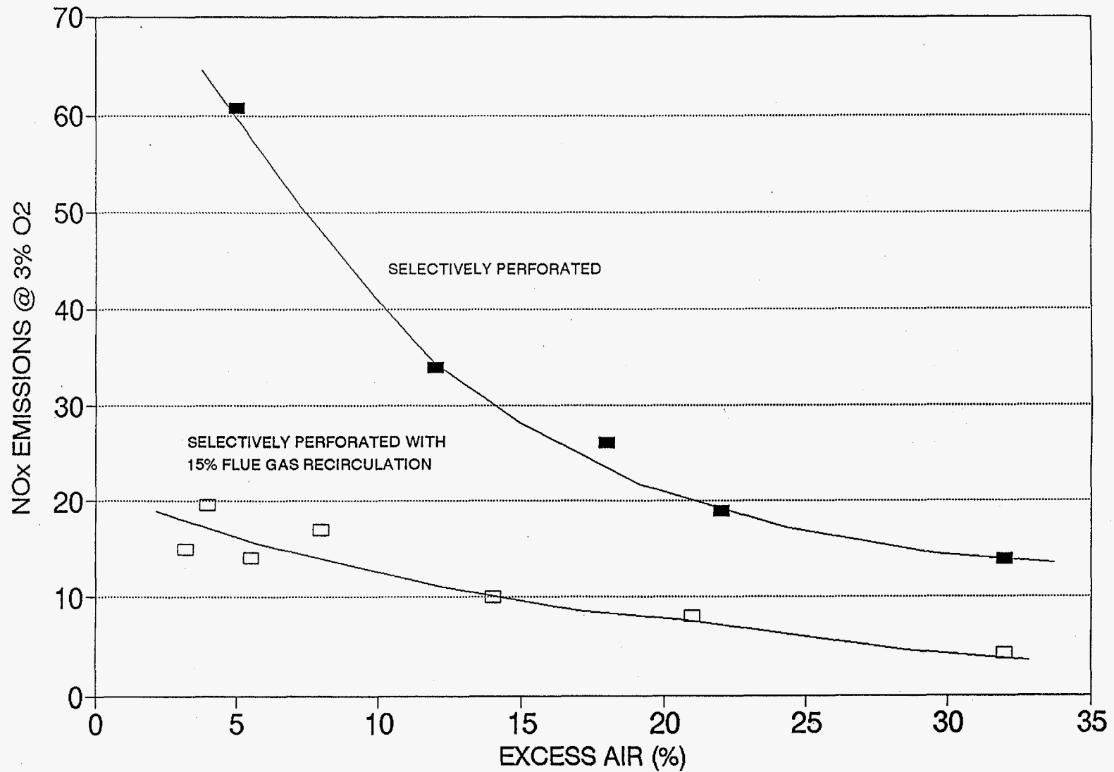
Figure 1-3. Experimental Data Demonstrating the Significant Reduction in NO x Achieved Simultaneously with Low CO Emissions Using the RSB Concept. Fired Duty -- 1 MBtu/hr-ft 2
