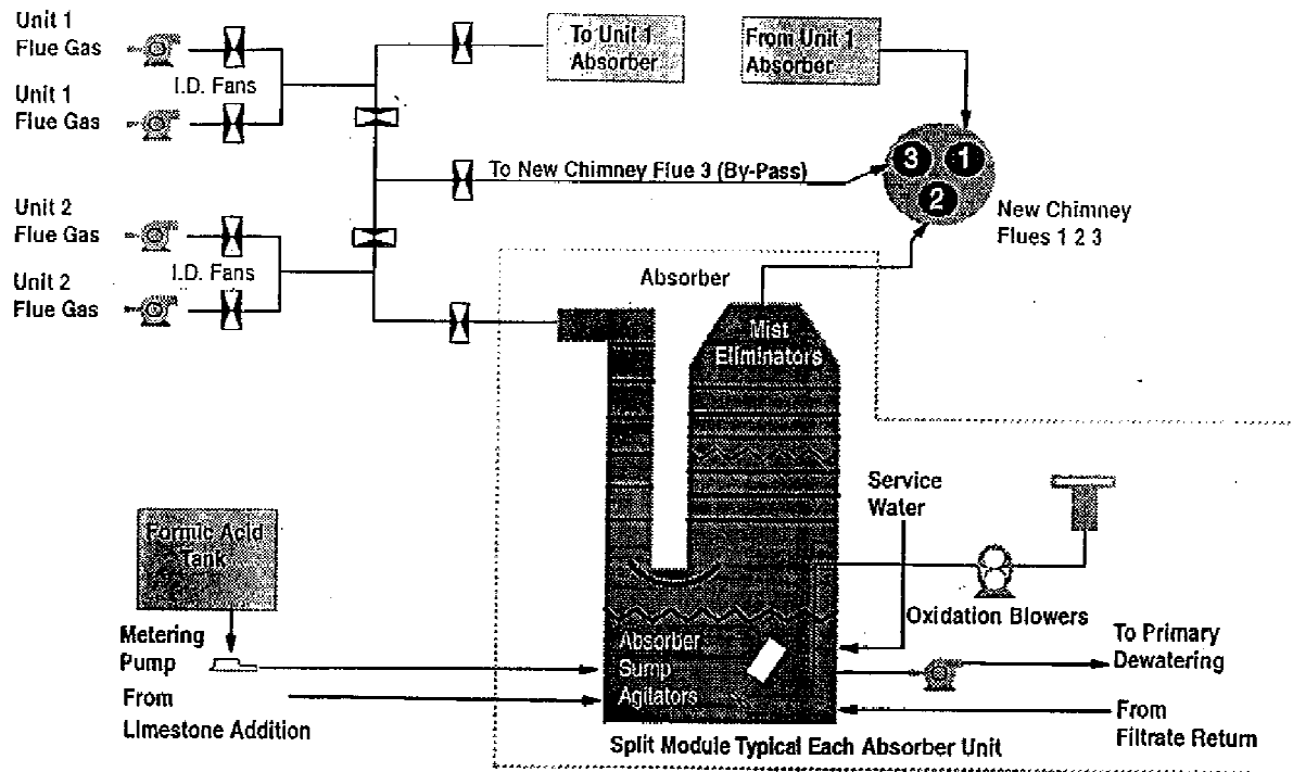
Figure 1 Simplified SHU Flow Diagram
