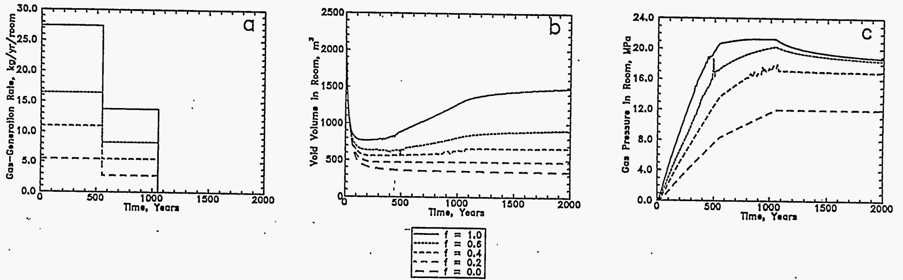
Figure 1. Gas-generation rate histories and SANCHO simulation results from Stone (1992).
