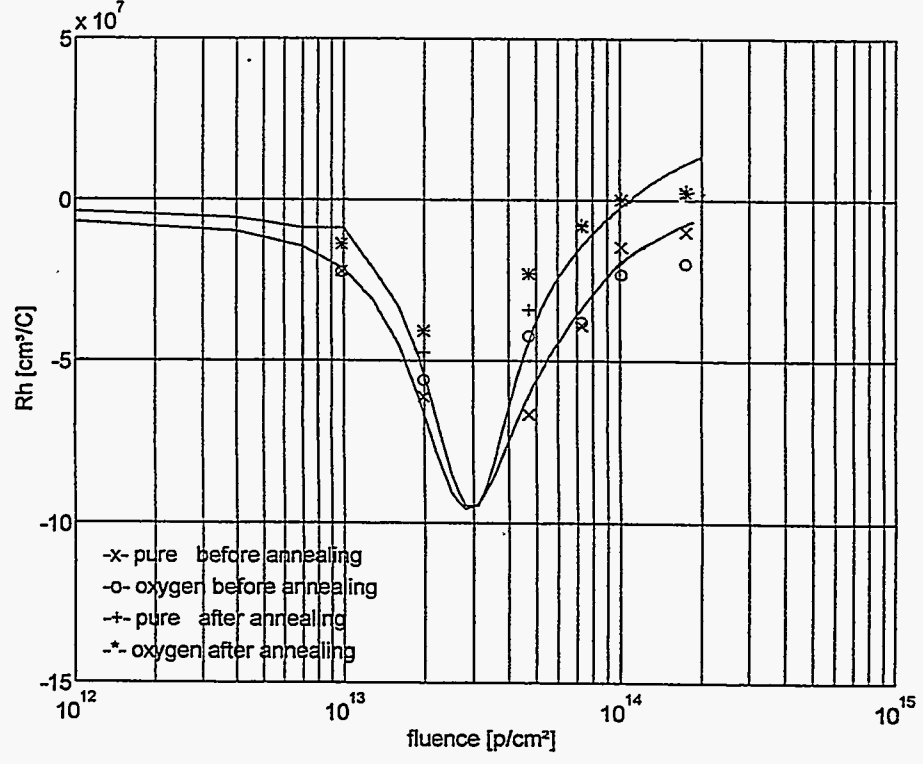
Figure 5b. Hall coefficient (measured at 27°C) versus fluence for pure and oxygenated samples before and after the annealing treatment.
