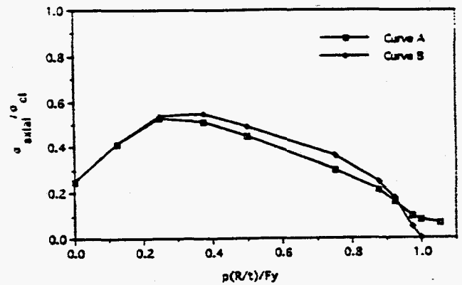
Figure 8 Strain-Hardening Effect on Buckling of Cylindrical Shell, R/t = 900
