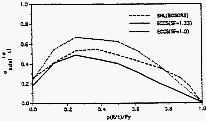
Figure 7 Comparison of Axial Compressive Stresses with ECCS Formulas using SF = 1.00 and 1.33 (Curve B), R/t = 900
