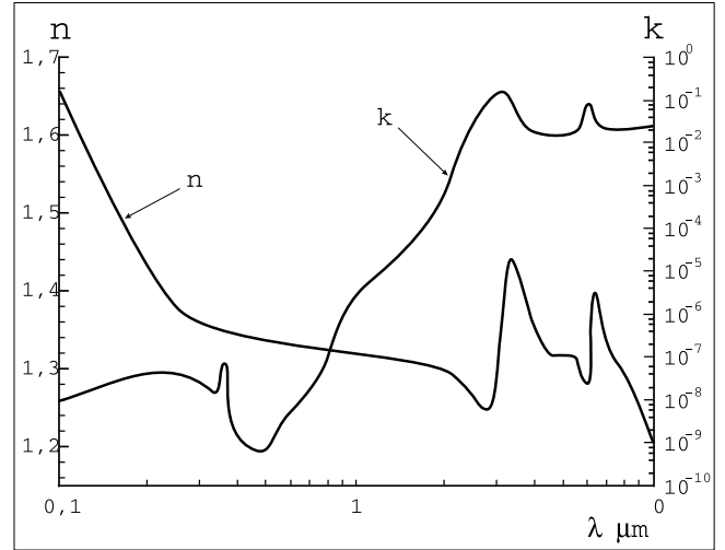
Figure 1. The dependence of the imaginary and real part of the refractive factor of water with wavelength calculated from the data of Bohren and Huffman [1982].
