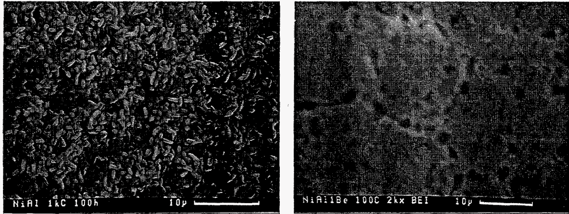
Figure 2: SEM (backscatter mode or secondary mode?) surface micrographs of \beta -NiAl (left) and Ni-49Al-1Be (right) after exposure for 100 h at 1000°C in air saturated with moisture at 20°C.
