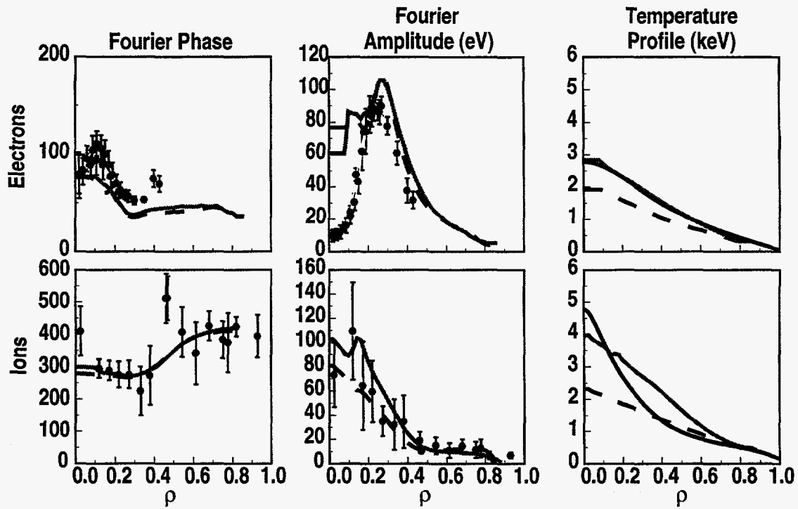
FIG. 6. Comparison of GLF23 model predictions with EXB shear included (solid grey line) and omitted (dashed line) for the case with \rho_{ECH} = 0.3 . Measured data \delta T_e and \delta T_i (circles) and T_e and T_i profiles (black lines) are also shown.
