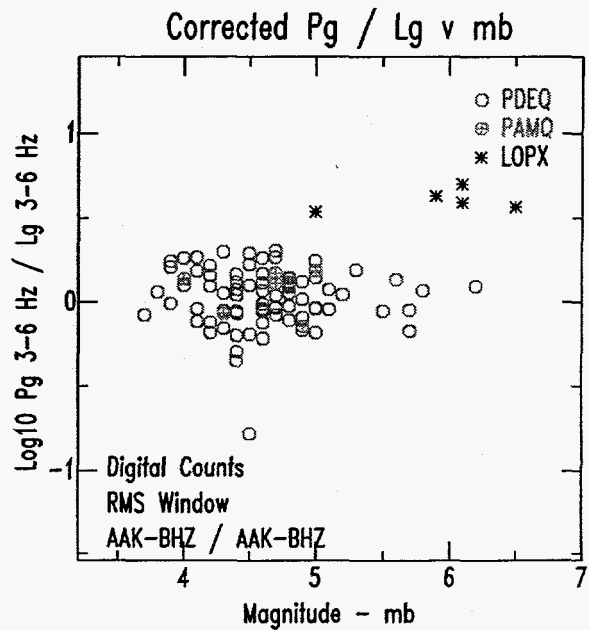
Figure 3. Phase ratio P_g/L_g discrimination plots for stations WMQ (left) and AAK. Center frequencies are 1.125 Hz and 4.5 Hz. As frequency increases, separation between earthquakes and explosions also increases.
