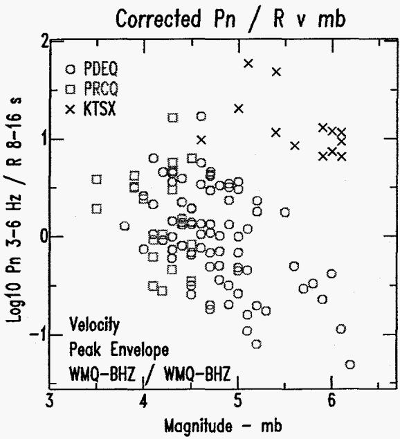
Figure 6. Short-period / long-period discrimination plots for stations WMQ (left) and AAK. Here we show P_n in ratio with R , but P_n in ratio with L also performs well. As P_n frequency increases, separation increases.
