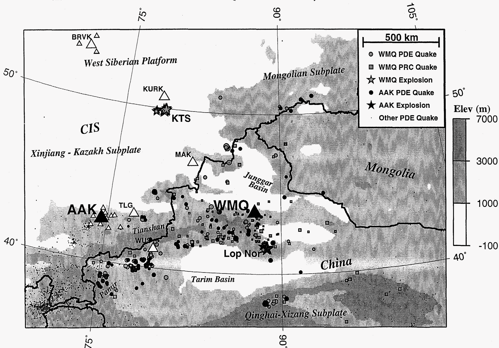
Figure 1. Study area map showing, shaded topography, nuclear explosion and test site locations, natural seismicity, and seismic stations. We used seismic data recorded at stations WMQ and AAK in this study.
