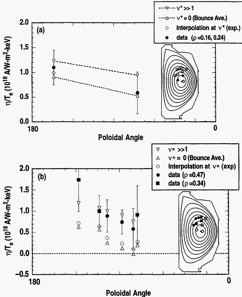
FIGURE 1. Comparison of theoretical and experimental values of normalized ECCD efficiency \eta/T_e as functions of poloidal angle: (a) near the magnetic axis, (b) off-axis. The inset plasma cross-sections show the ECH deposition locations.
