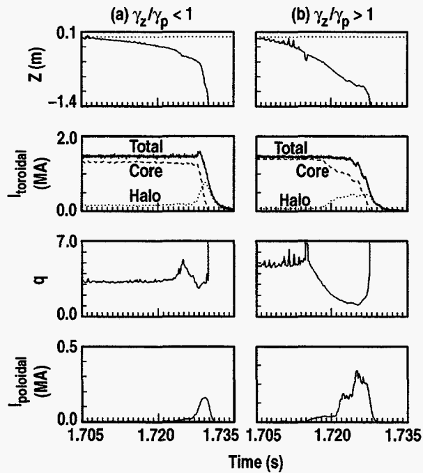
Fig. 4. Comparison of two VDE discharges with a ratio of \gamma_z/\gamma_p < 1 [(a) discharge 90204] and \gamma_z/\gamma_p > 1 [(b) discharge 90219]. Time evolution of vertical position, total toroidal current, core toroidal current (dashed), halo toroidal current (dotted), edge safety factor q , and total poloidal halo current.
