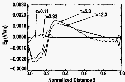
FIGURE 1. Evolution of the parallel electric field. The normalized perpendicular diffusion coefficient is 1.0 and mean free path is equal to the connection length L .
