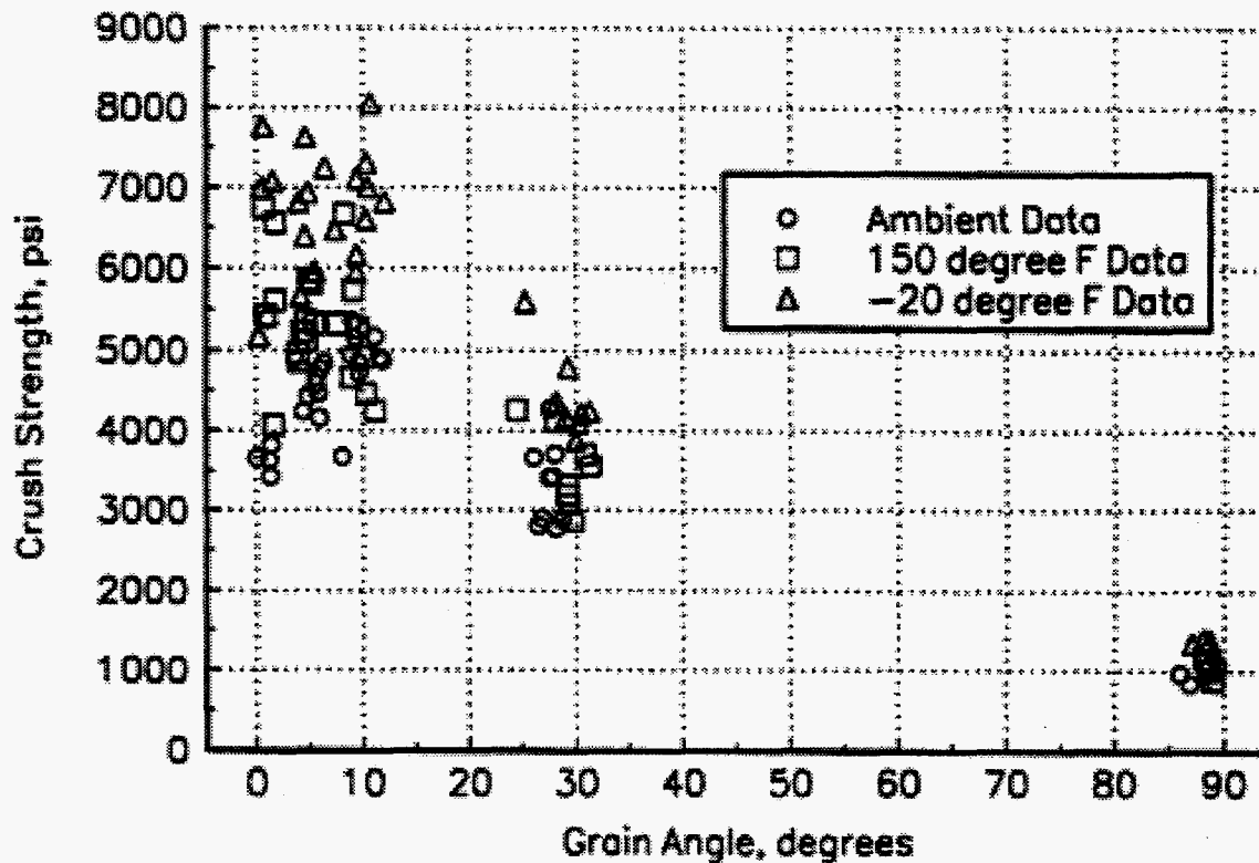
Figure 5. All UW Crush Data Plotted Against Grain Angle (Phi)
