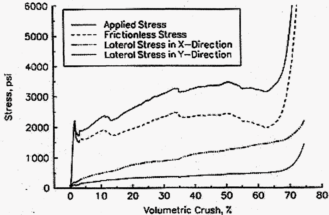
Figure 17. Stress-Volumetric Crush curves for Specimens C533 Showing Increasing Lateral Stresses and Increasing Frictional Effects
