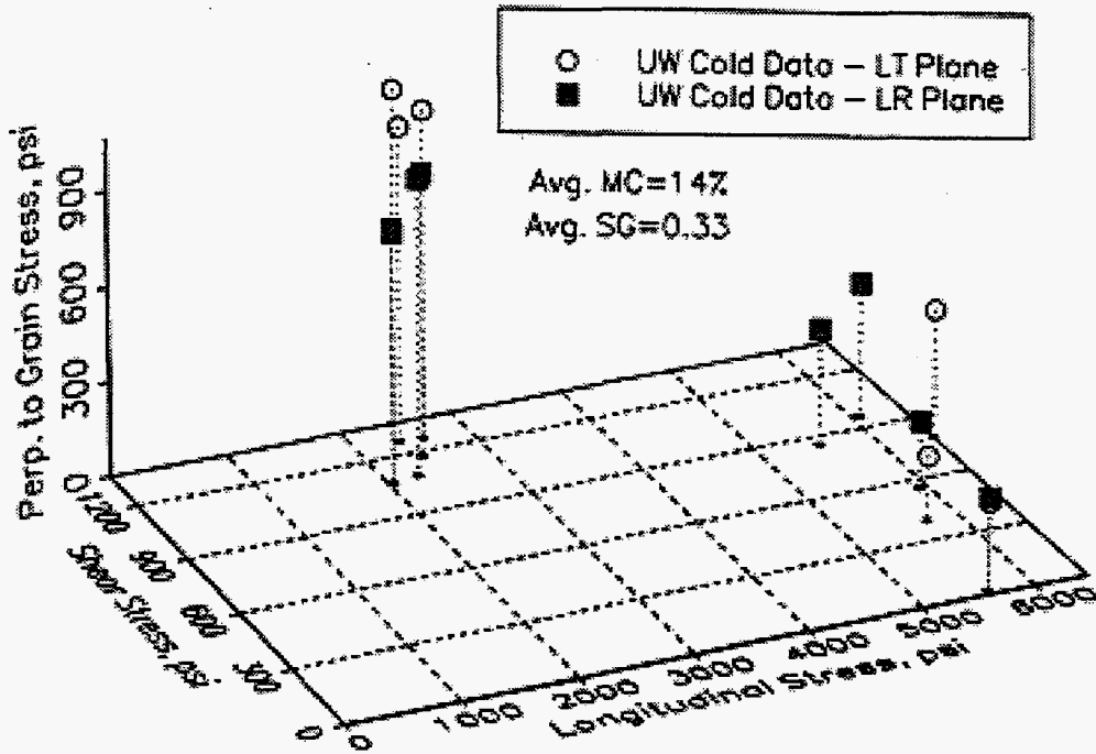
Figure 12. Stresses in the Material Coordinate System at Peak Crush Stress for Cold Data Subset
