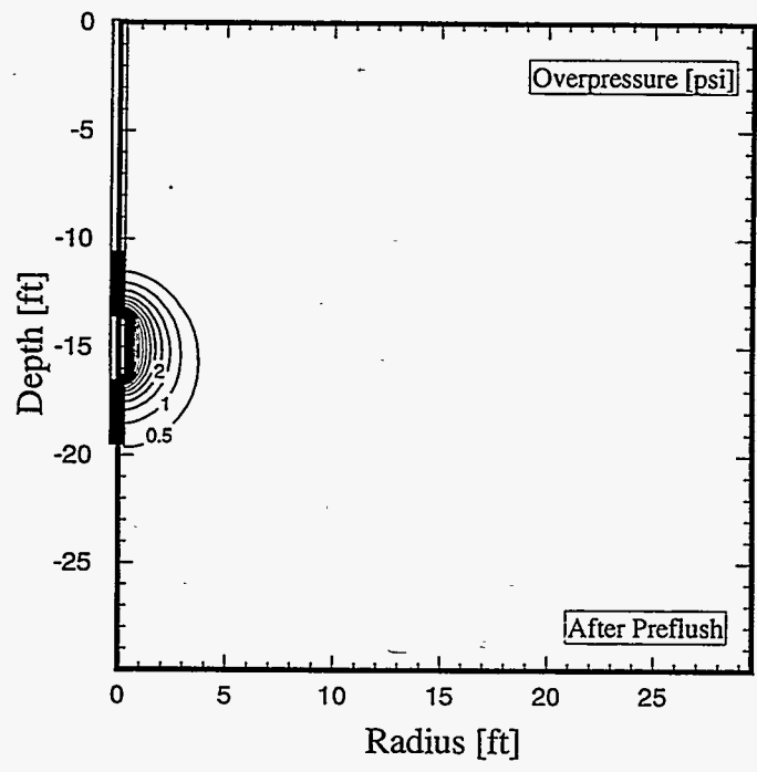
Figure 17: Liquid saturation and pressure distribution after preflushing
