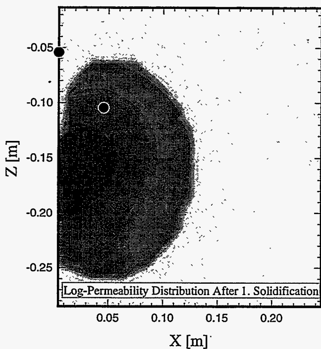
Figure 10: Logarithm of permeability after solidification of primary grout plume
