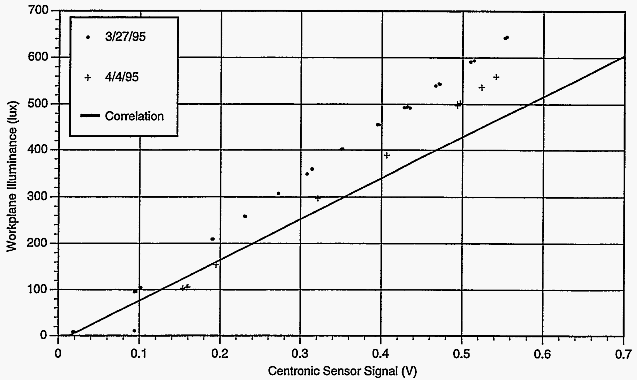
Figure 4. Centronics ceiling-mounted photosensor signal (V) and the resultant average workplane illuminance (lux) as the lighting system is operated over its full dimming range with no daylight. Data points for two days are given, March 27, 1995 and April 4, 1995.
