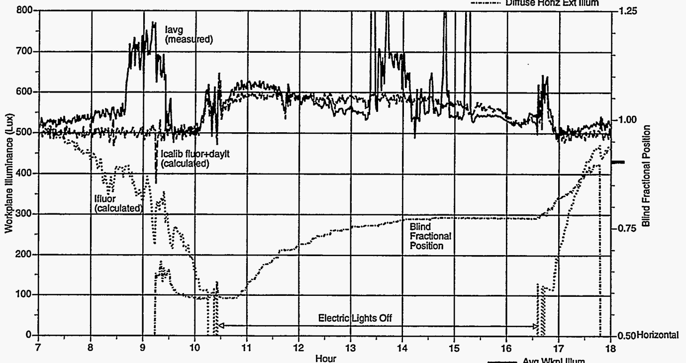
Figure 8b. Average workplane illuminance, calibrated workplane illuminance, workplane illuminance provided by electric lighting, and blind fractional position for a clear sunny day, February 18, and southwest-facing window. The blinds were controlled to block direct sun and meet the design workplane illuminance level using the shielded Li-Cor ceiling mounted photosensor for control. The electric lighting system was dimmed or shut off in response to the available daylight.
