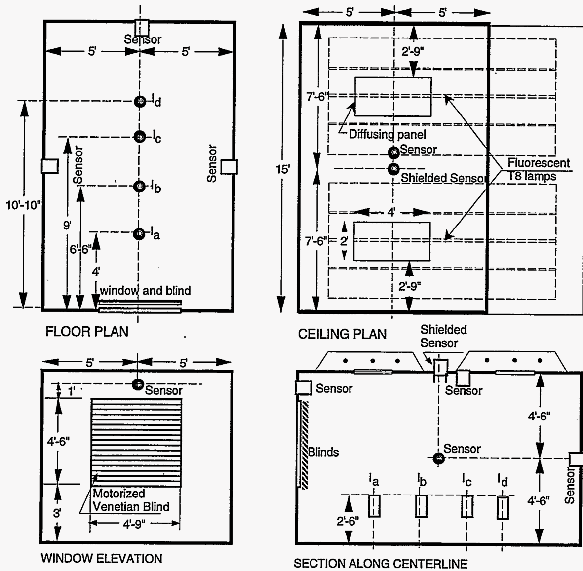
Figure 1. Plan and section of 1:3 reduced-scale model. Dimensions are shown in full-scale.
