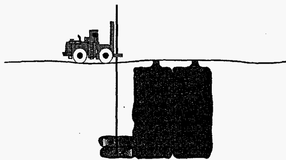
Figure 2. Conventional column jet grouting.
