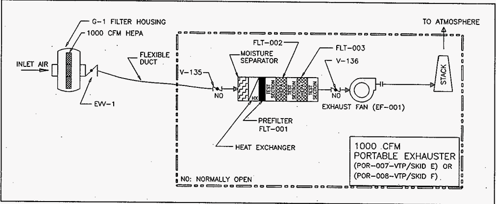
FIGURE 1 FUNCTIONAL TEST HARDWARE CONFIGURATION SCHEMATIC
