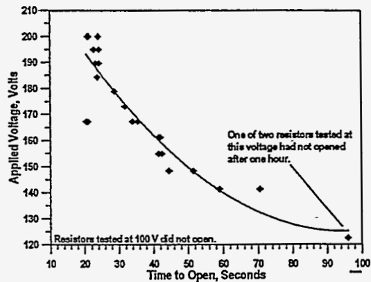
Figure 8, Time, in seconds, until the tin oxide resistor opened.
