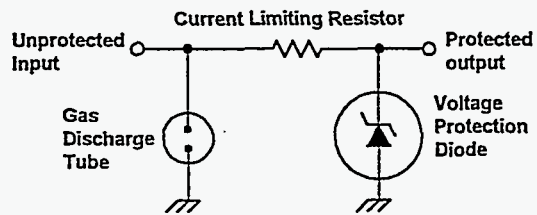
Figure 1. Surge Protector from Reference 1.
