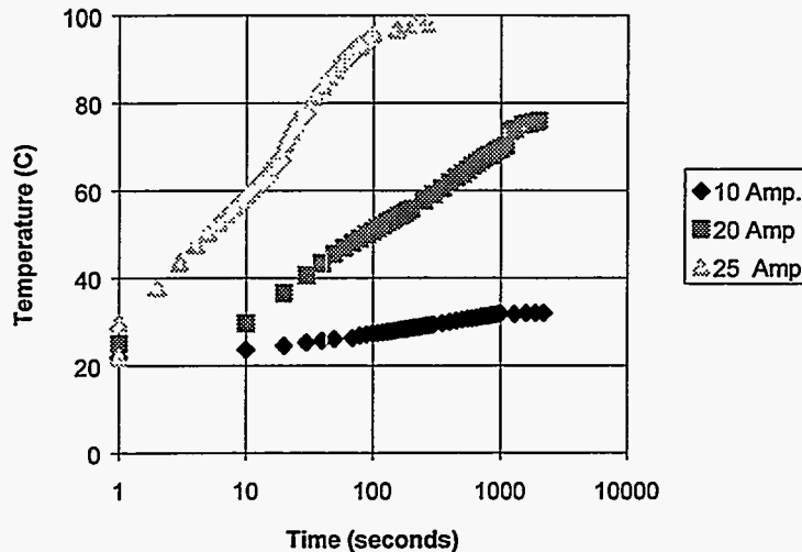
Figure 1. Temperature as a function of time and current for a 20-gauge Teflon-insulated conductor surrounded by a bundle of 80 similar conductors that were not carrying current.
