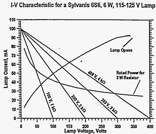
Figure 15, Current-voltage characteristic showing the load lines for various tester voltages and the 3 W maximum power rating line.
