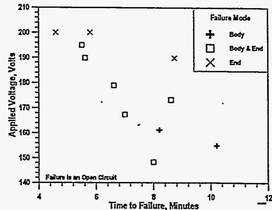
Figure 10, Time until opening for Ceramic/Carbon resistors.
