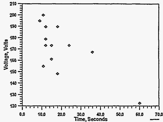
Figure 4, Time until the resistance increase starts to stabilize.
