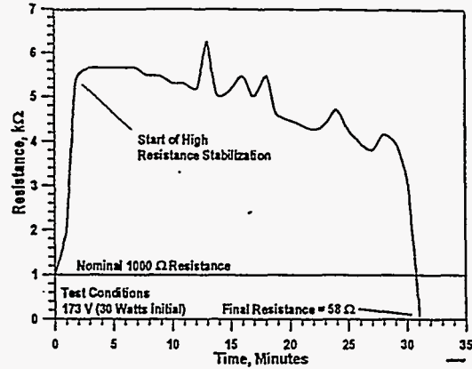
Figure 3, Resistance change characteristic for carbon composition resistors tested at 173 V, 30 W initial power. Shorting occurred in all but one of the resistors tested above 20 W.
