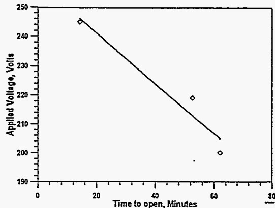
Figure 18, Time to open for 3 W tin oxide and 2 W carbon composition resistors in series.
