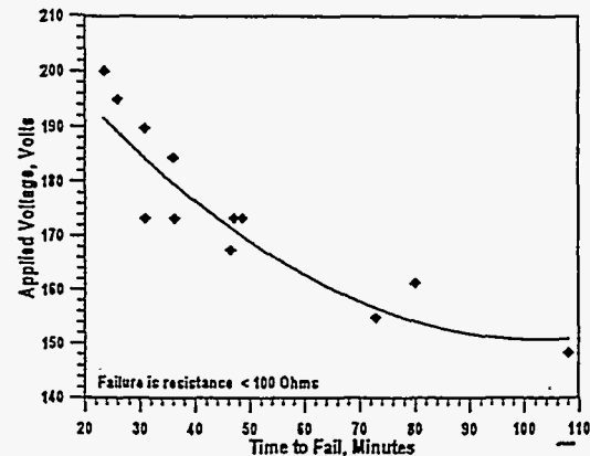
Figure 5, Time until short for Carbon Composition Resistors.
