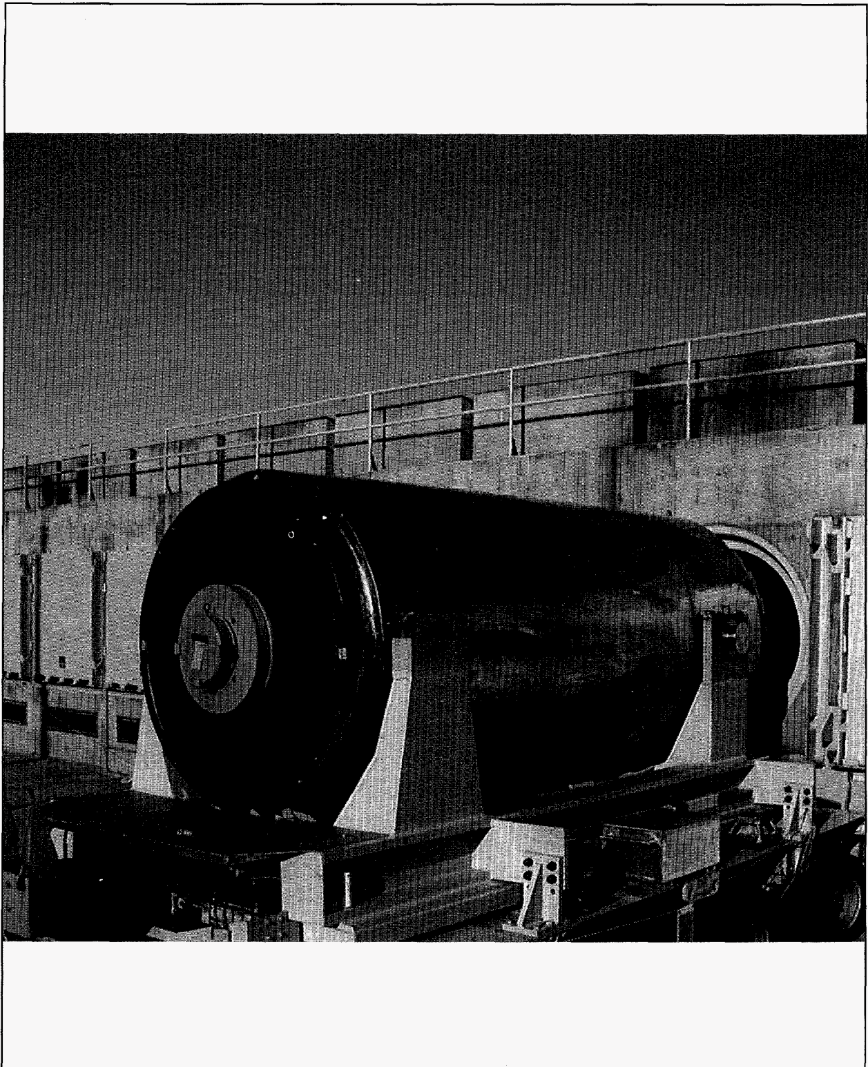
Figure 3.10-4 Photograph of a NUHOMS TC Being Mated with an HSM
