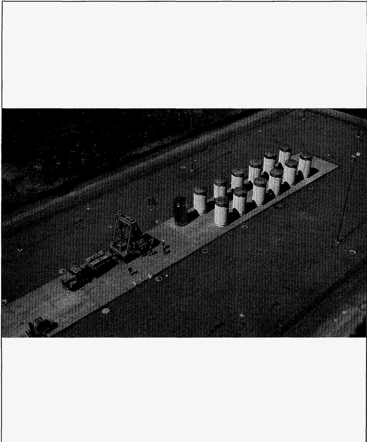
Figure 4.6-3 Photograph of the Surry ISFSI
