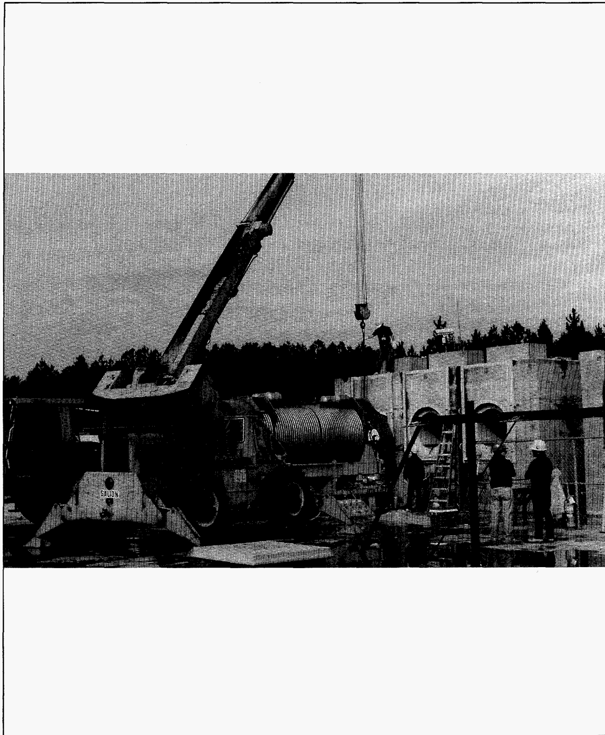
Figure 4.3-3 Photograph of the H.B.Robinson ISFSI During Loading
