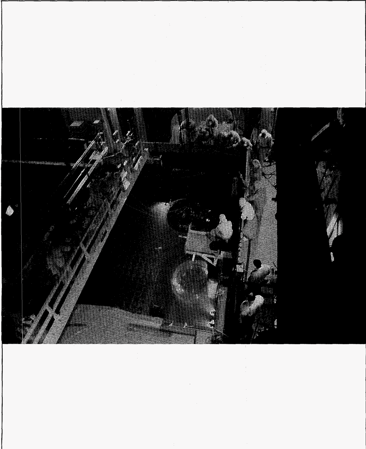
Figure 3.1-4 Photograph of Castor V/21 in the Surry Power Station SFP
