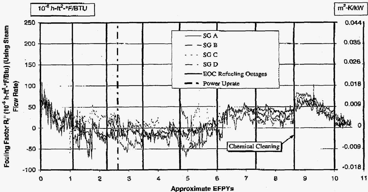
Figure 4. Callaway Historical Global Fouling Factor
