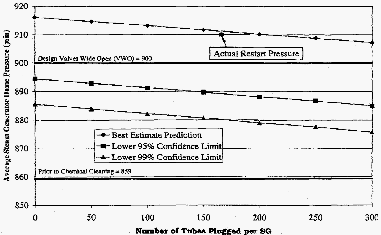
Figure 7. Predicted Steam Pressure After Chemical Cleaning at San Onofre 2
