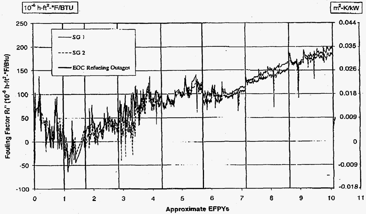
Figure 2. San Onofre 2 Historical Global Fouling Factor
