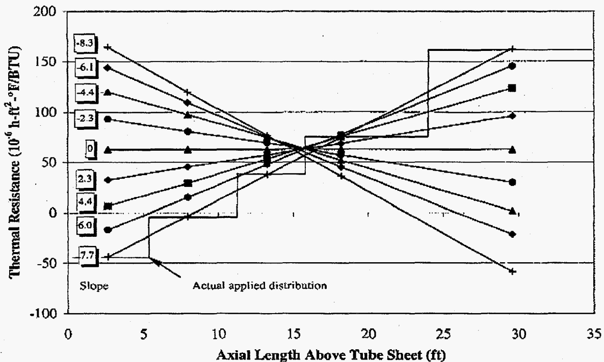
Figure 8. Linear Variations of Fouling Factor Applied to ATHOS Model (60 10 -6 Avg)
