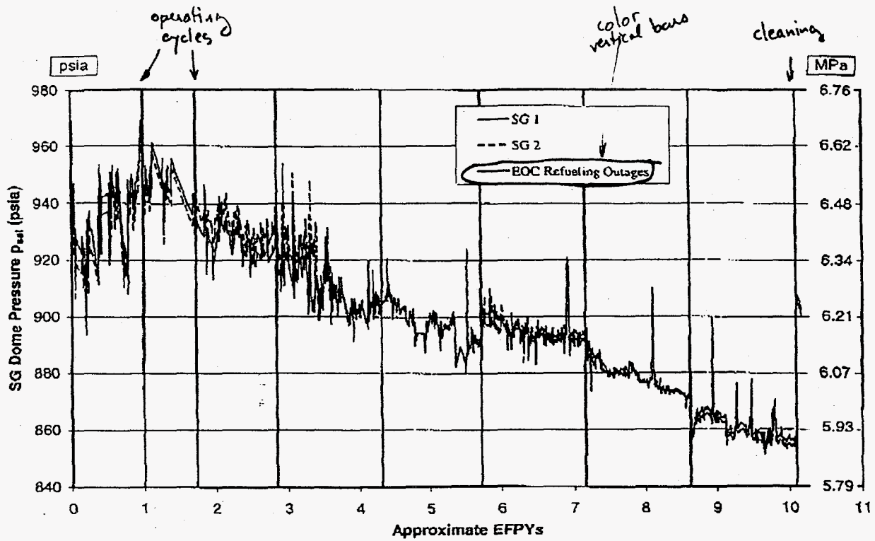
Figure 1. San Onofre 2 Historical Steam Generator Pressure
