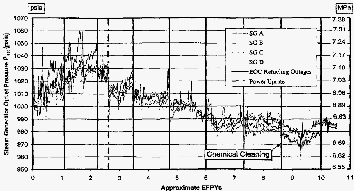
Figure 3. Callaway Historical Steam Generator Pressure
