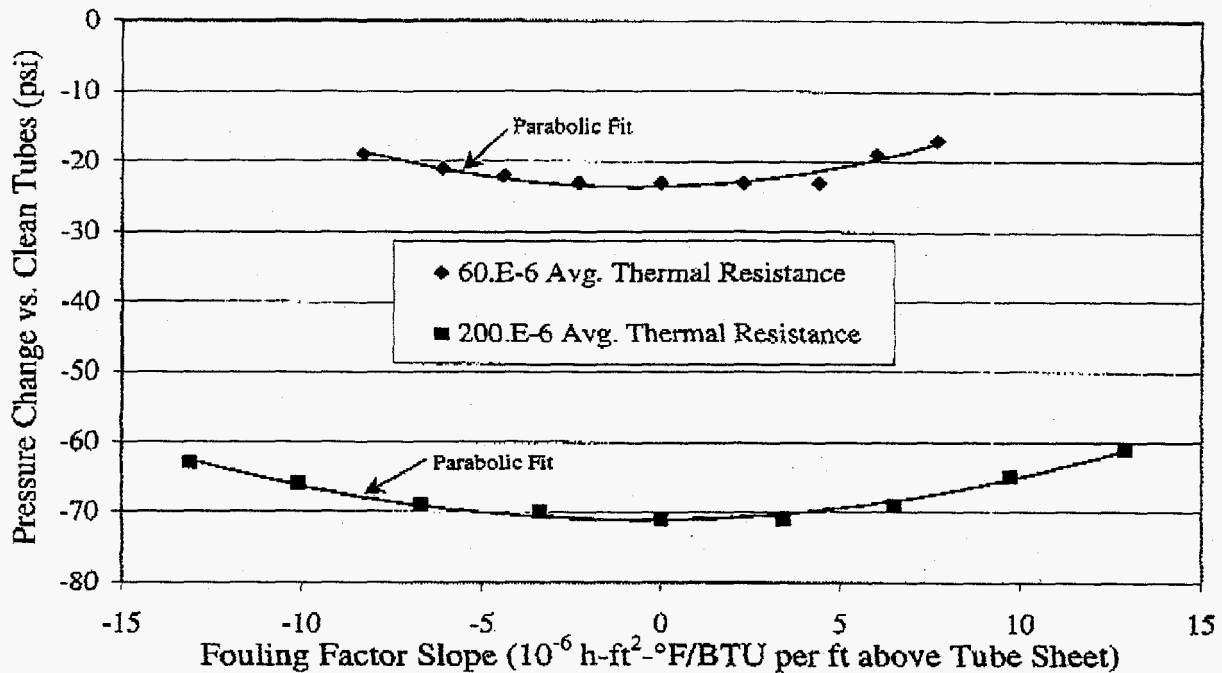
Figure 9. Results of Sensitivity Study
