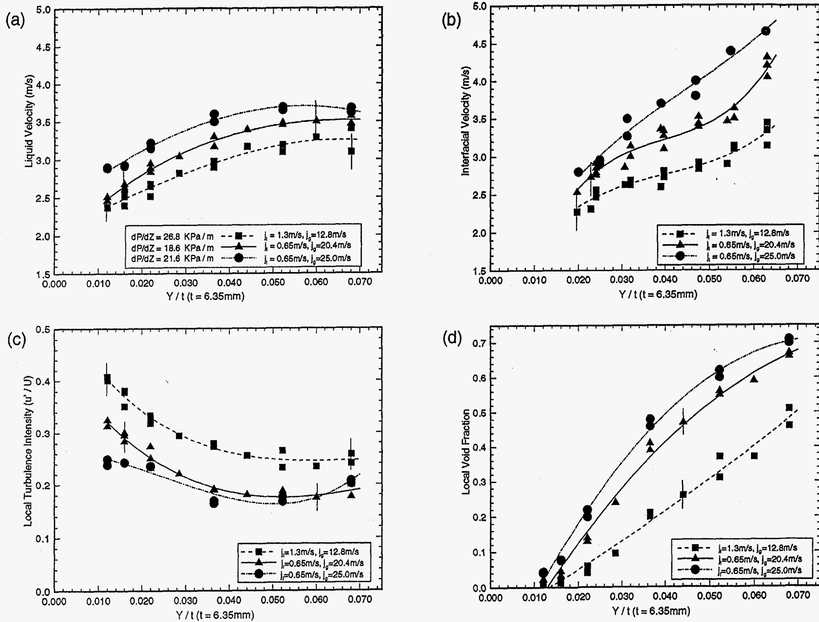
Figure 4. Near-wall HFA data. (a) liquid velocity using calibration (b) interfacial velocity using cross-correlation (c) turbulence intensity (d) void fraction
