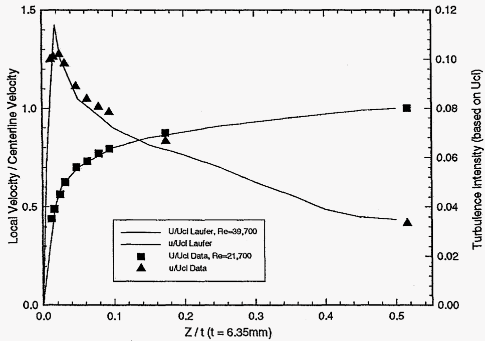
Figure 2. (a) HFA calibration in single-phase liquid flow (b) Single-phase turbulent profiles compared with Laufer's (1951) data
