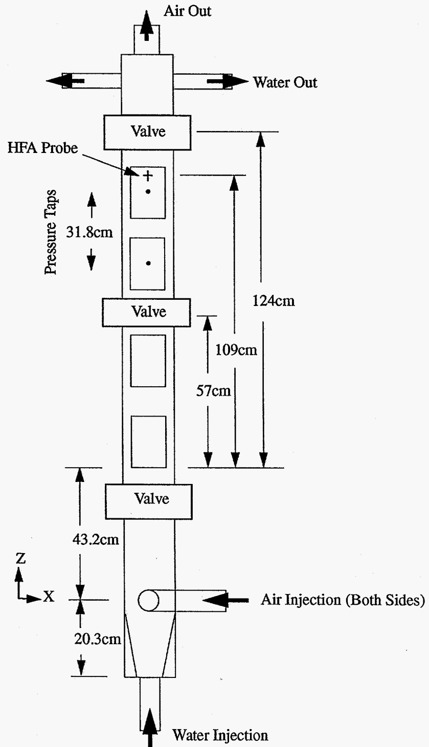
Figure 1. Test Section Schematic
