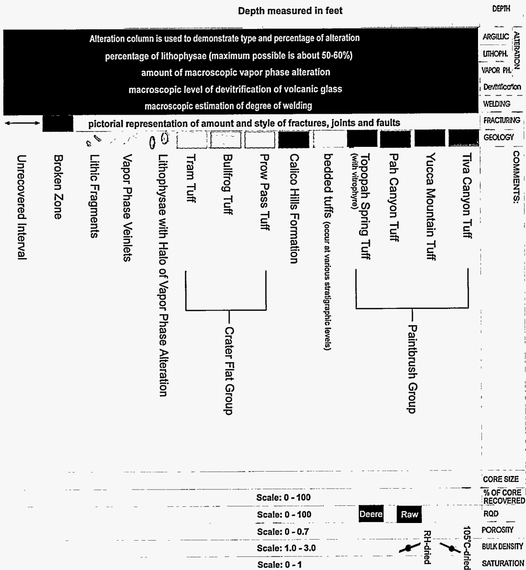
Figure B-1. Example geologic core log form with parallel columns for representing various geologic features and other quantitative and semiquantitative information as a function of depth.
