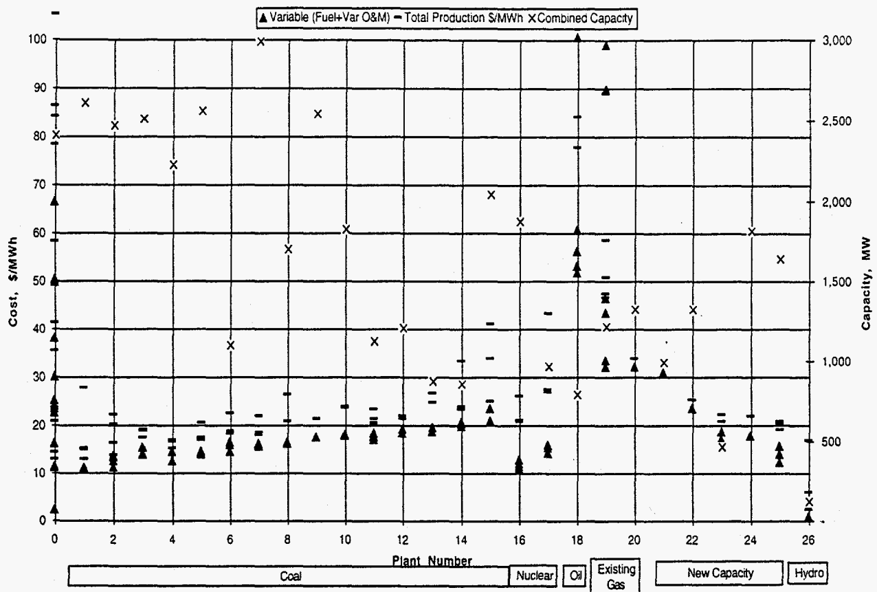
Figure 3. Separation of 131 Ohio power plants into 25 bins by technology and variable cost for use in ORCED.
