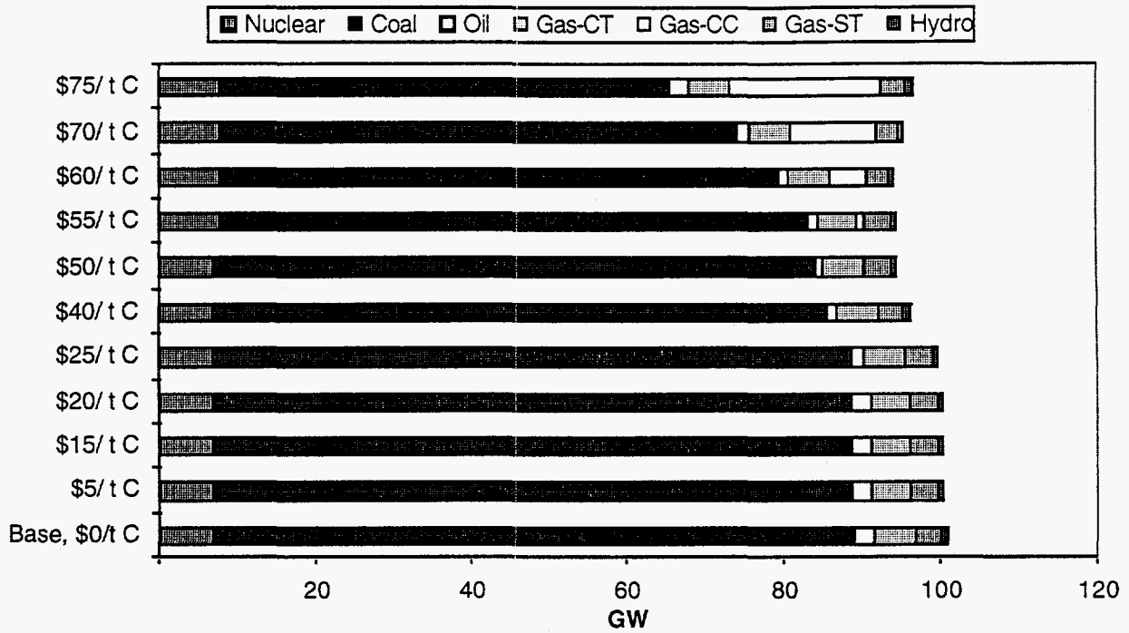
Figure 8. ECAR capacity (GW) with carbon charge and demand reduced due to price elasticity.
