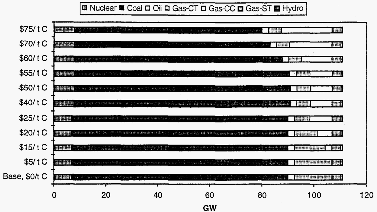
Figure 12. ECAR capacity (GW) with varying carbon charge rates and constant demands.
