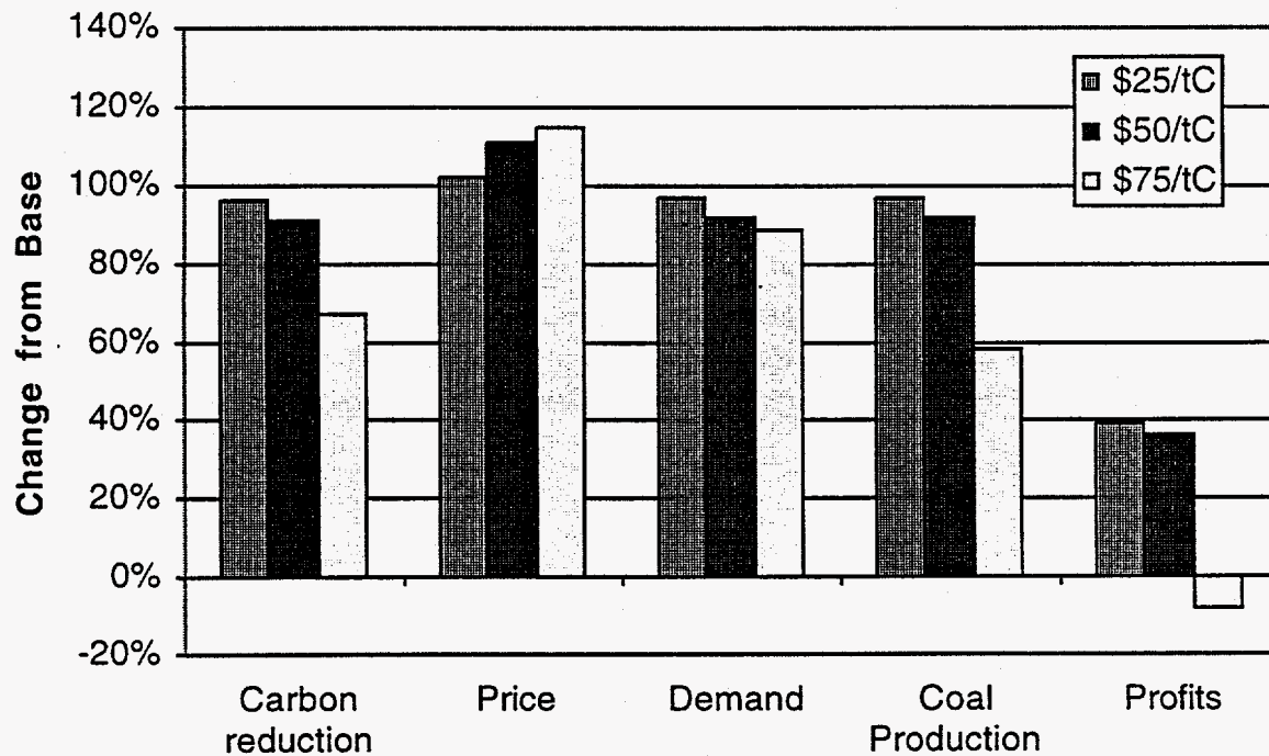
Figure 14. Changes in key parameters with carbon charges of $25/tC, $50/tC, and $75/tC.
