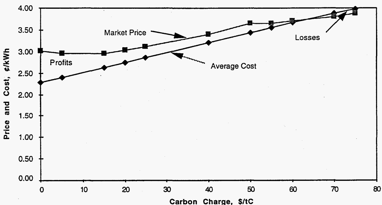
Figure 10. Average total cost and market price at different charge rates. The area between the curves represent extra profits to the generators.
