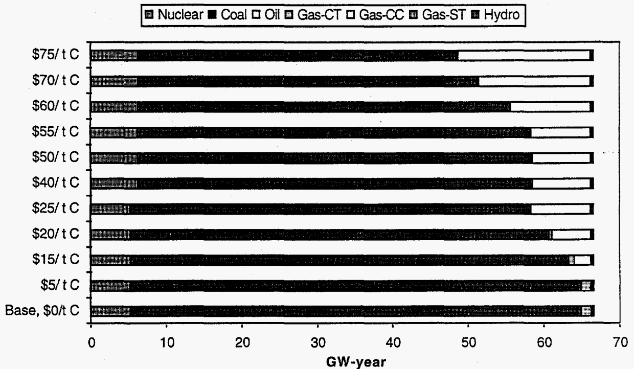
Figure 13. ECAR generation (GW-year) with varying carbon charge rates and constant demands.
