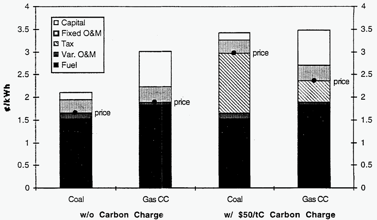
Figure 2. Cost of existing coal plant and new gas combined cycle plant operating at 90% capacity factor with and without a carbon charge. Note that a plant's bid price is based on its variable cost.
