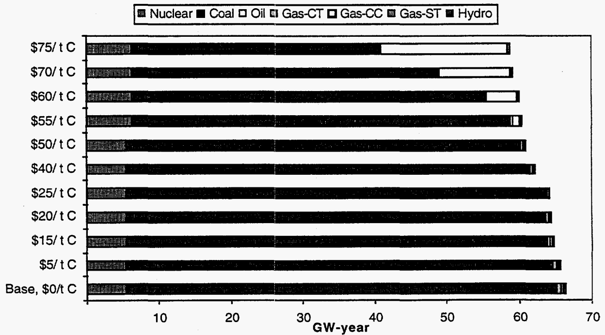
Figure 9. ECAR generation (GW-year) with carbon charge and demand reduced due to price elasticity.
