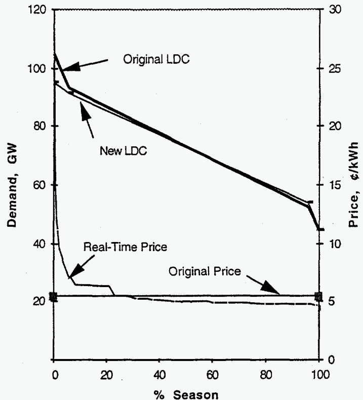
Figure 4. Peak period load duration curves and prices before and after elasticity.
