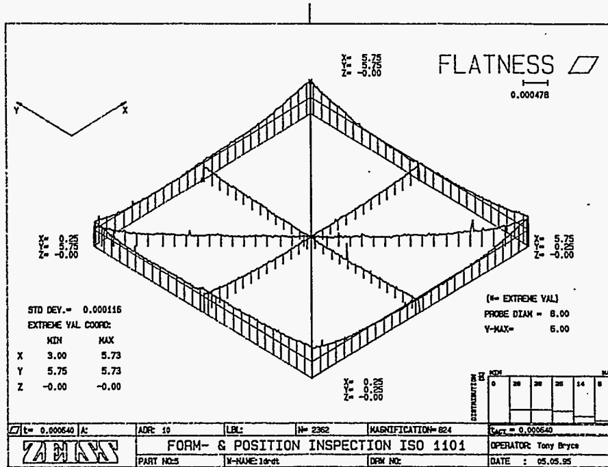
Figure 10. Platen Flatness After Thermal Cycling
