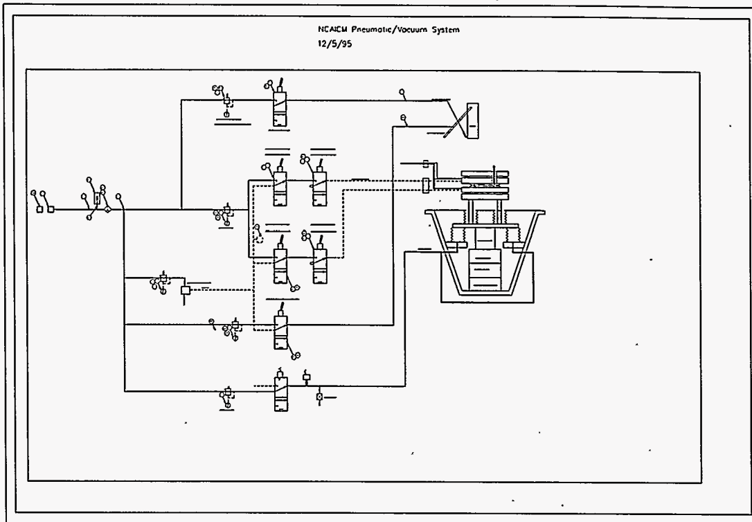
Figure 11. Pneumatic Schematic
