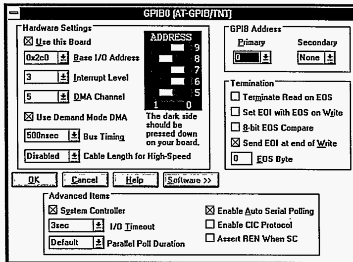
Figure 15. GPIB Configuration.
