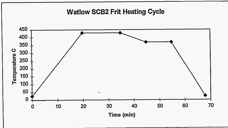
Figure 17. Typical SCB-2 Frit Thermal Cycle
