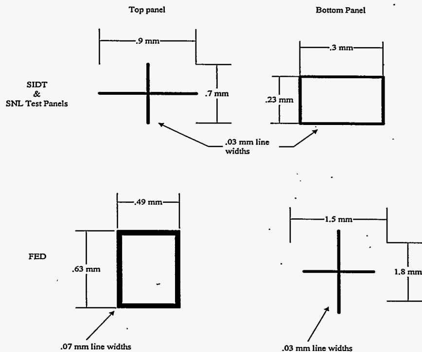
Figure 22. Alignment Marks (not to scale)
