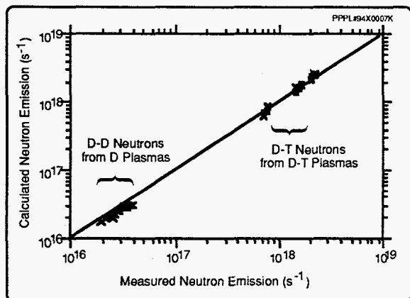
Figure 5. Comparison of neutron emission calculated from plasma parameters with measured fusion power.
