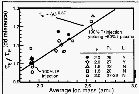
Figure 3. Variation of global energy confinement as a function of average ion mass.
