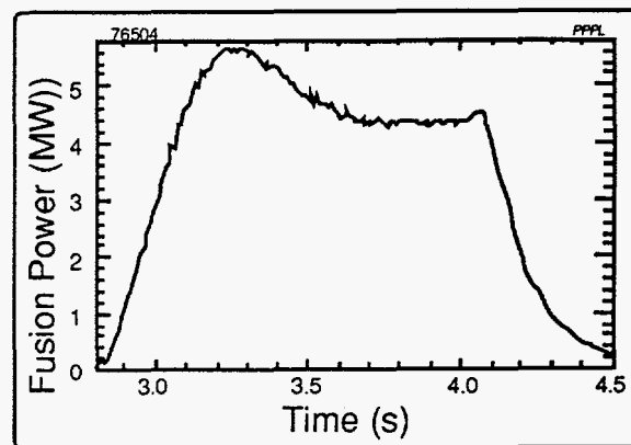
Figure 6. Fusion power profile used for alpha physics studies. This pulse produced 6 MJ.
