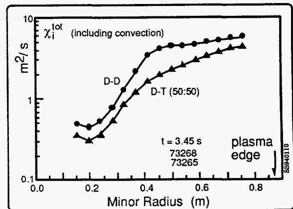
Figure 4. Comparison of ion energy radial transport in D-D and D-T plasmas.
