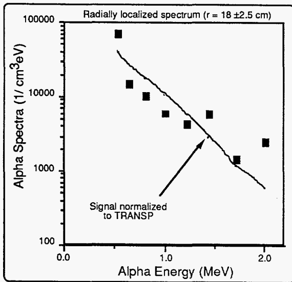
Figure 12. Distribution function for energetic alpha particles measured by alpha charge exchange from preliminary measurements by General Atomics, Ioffe Institute and MIT collaboration. The solid line is the distribution calculated by TRANSP.
