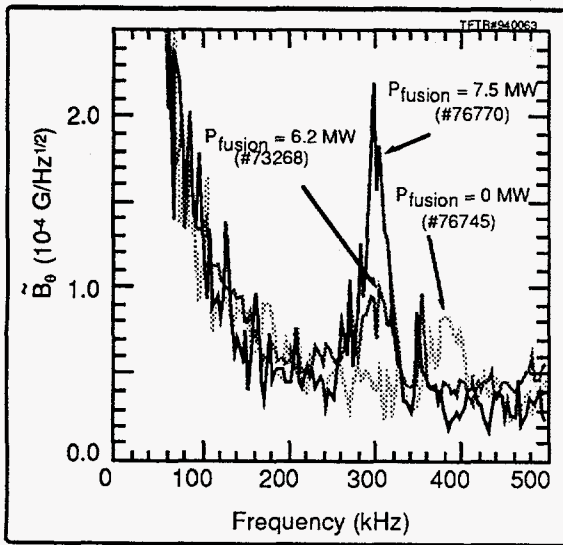
Figure 16. Possible alpha driven TAE mode.
