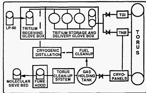
Figure 2. TFTR tritium system schematic. The low inventory cryogenic distillation system has been constructed but is not installed.
