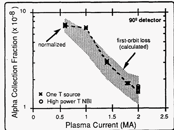
Figure 11. Measured loss of alpha particles.
