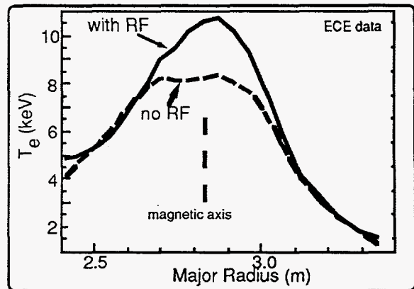
Figure 17b. Electron heating by ICRF in a D-T plasma.
