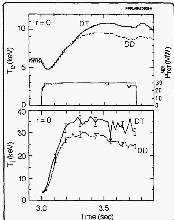
Figure 15. Tests for alpha heating.
