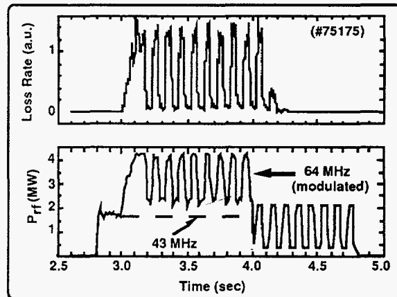
Figure 14. Demonstration of a possible ICRF burn control or ash removal technique on TFTR.
