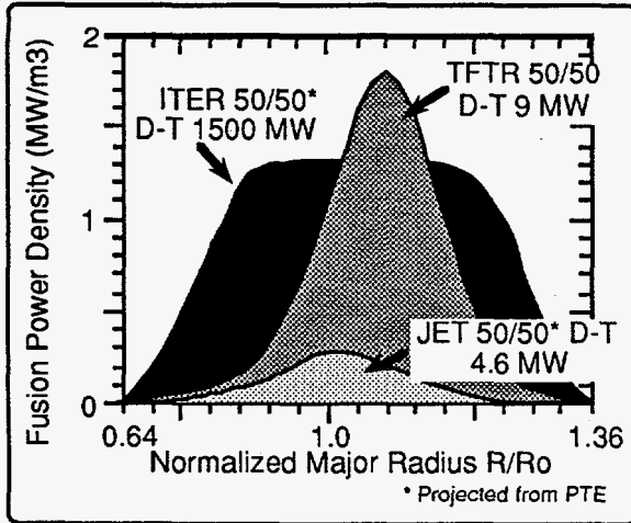
Figure 9. Comparison of fusion power density in TFTR, JET and ITER versus normalized major radius. The JET value is obtained by increasing the D/T mix in the PTE experiment to 50/50 as described in Reference 3.
