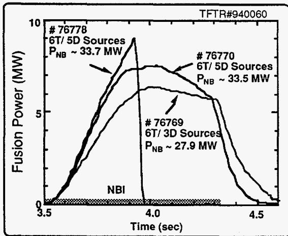
Figure 7. Time evolution of fusion power for the highest power pulses.
