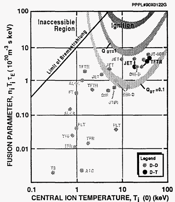
Figure 8. Lawson diagram for steady-state D-T plasmas.
