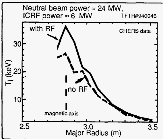
Figure 17a. Ion heating by ICRF in a D-T plasma.
