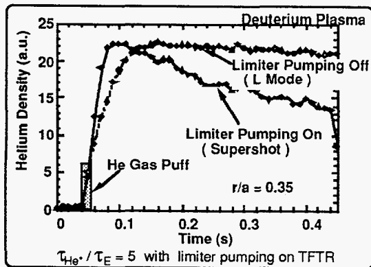
Figure 13. Helium pumping in TFTR
