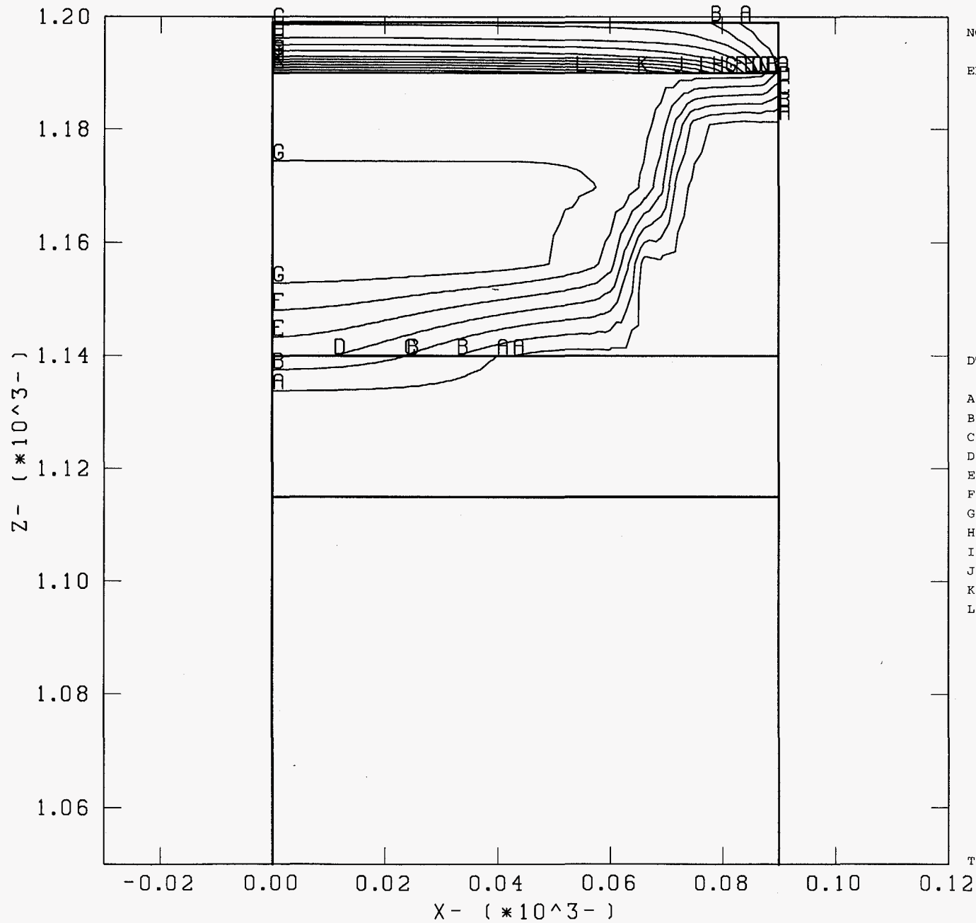
Change in Saturation from In Situ Conditions Ptn Modeled as Tpc-TN Time=25 Years
