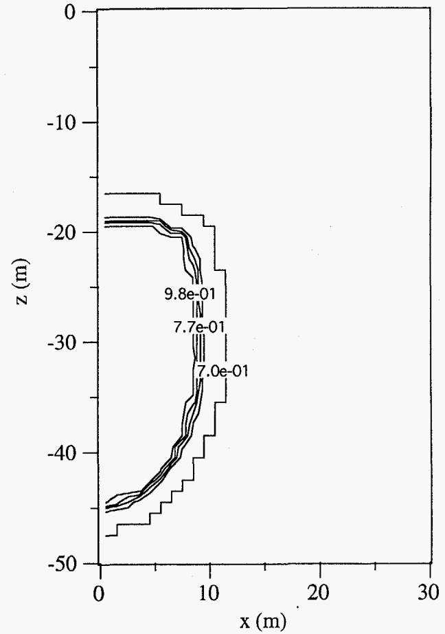
Matrix Water Saturation
