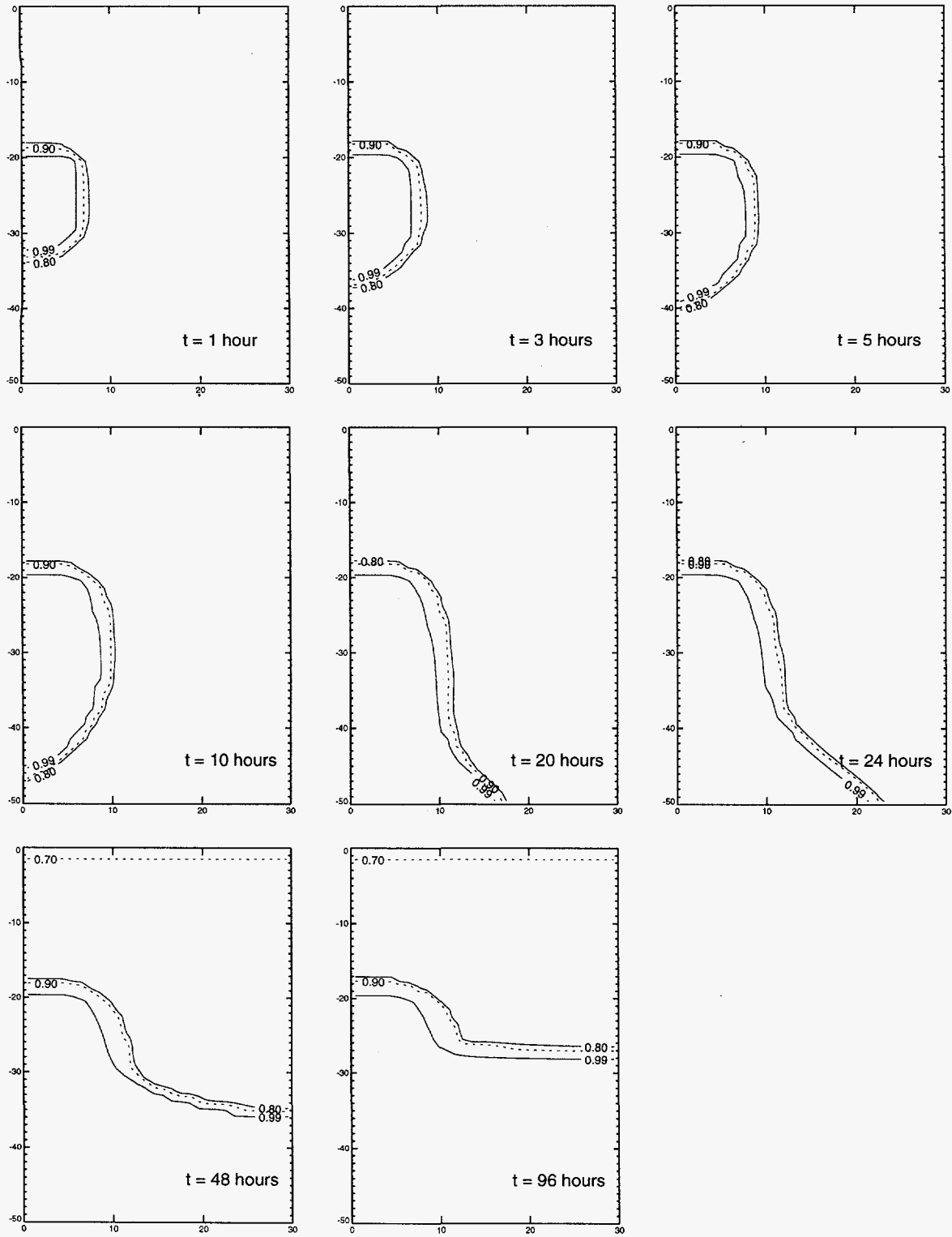
Figure 5.3-8 Equivalent continuum model prediction of saturation front movement over 4 days for 50 μm aperture fractures in TSw2 tuff.
