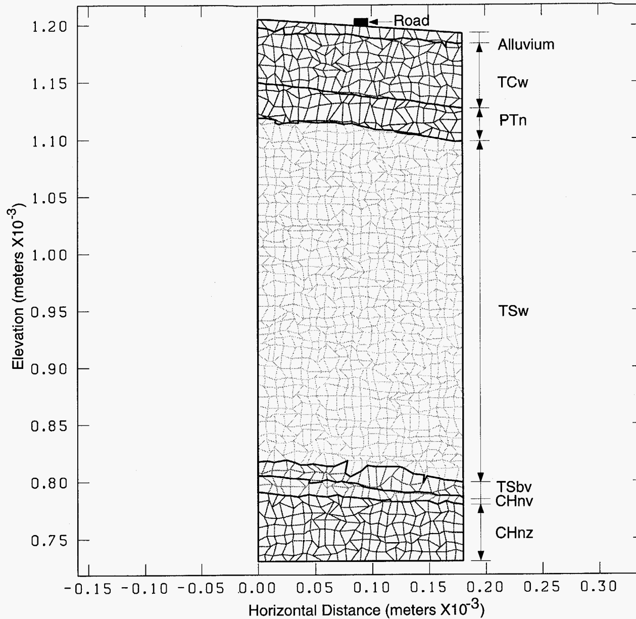
Saturation Near UE25 a#1 Resulting from Road Watering E-W Transect, Seed #2, Alluvium Conductivity per ESF Analyses Computational Grid
