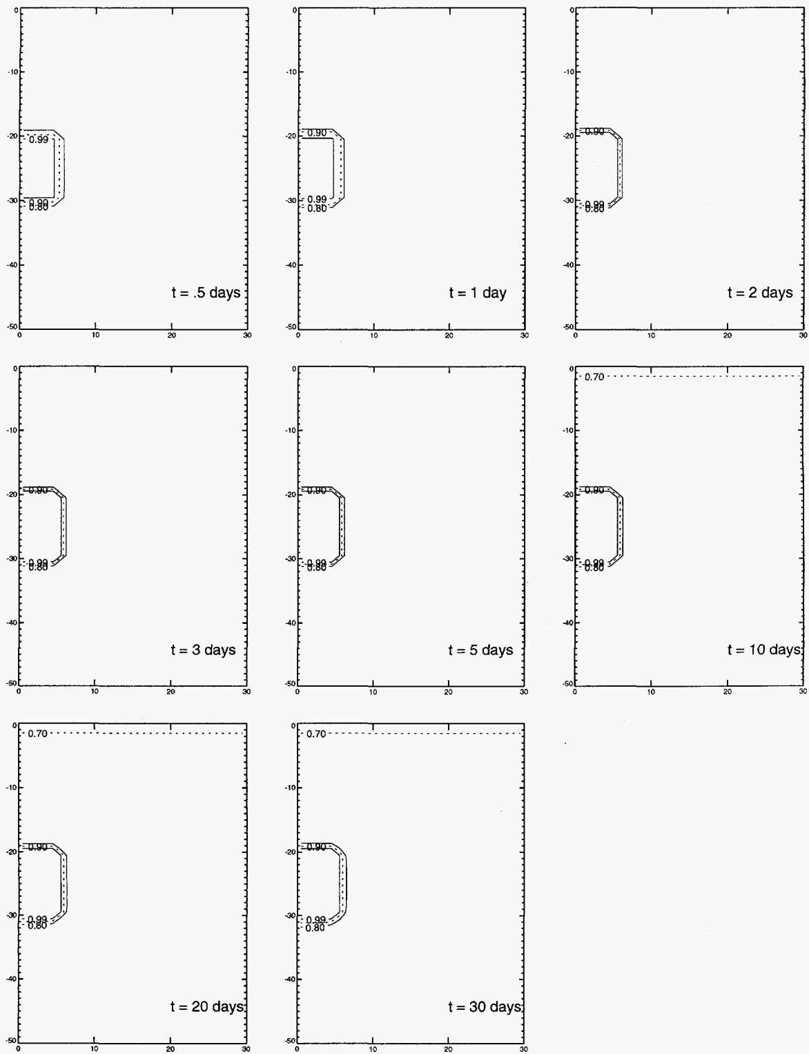
Figure 5.3-2 Equivalent continuum model prediction of saturation front movement over 30 days for 4.55 μm aperture fractures in TSw2 tuff.
