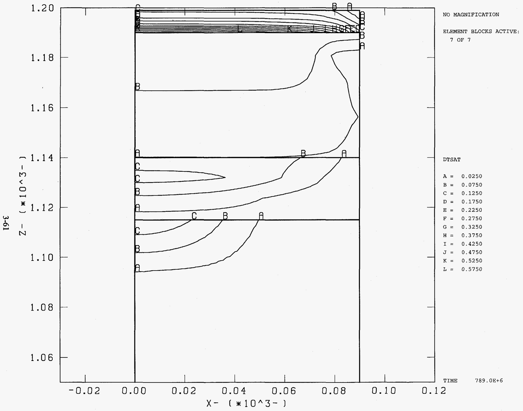
Change in Saturation from In Situ Conditions Ptn Modeled as Pah Canyon Member Time=25 Years
