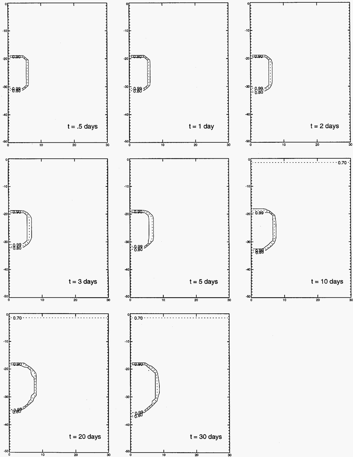
Figure 5.3-3 Equivalent continuum model prediction of saturation front movement over 30 days for 12.5 μm aperture fractures in TSw2 tuff.
