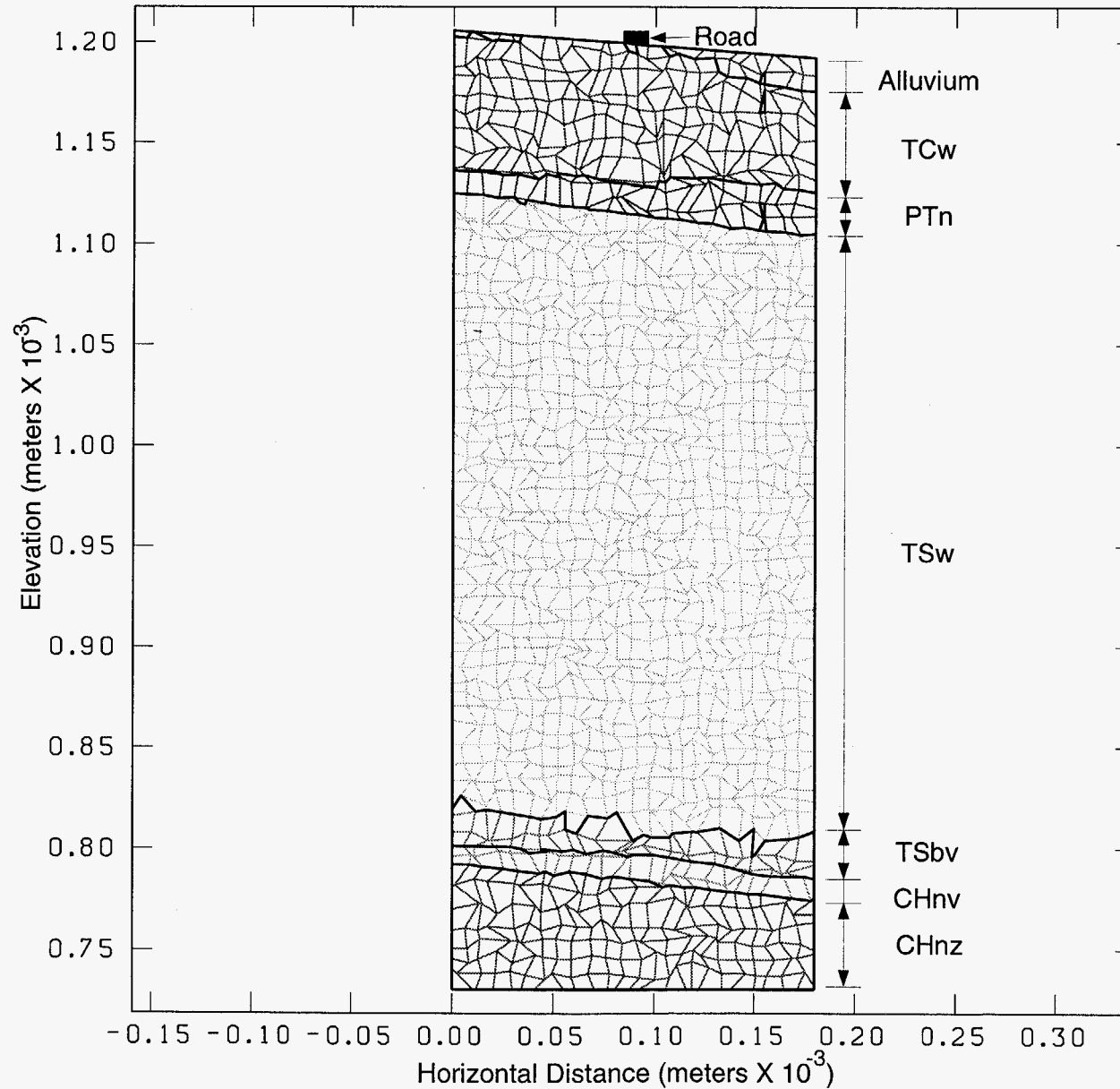
Saturation Near UE25 a#1 Resulting from Road Watering E-W Transect, Seed #1, Alluvium Conductivity per ESF Analyses Computational Grid
