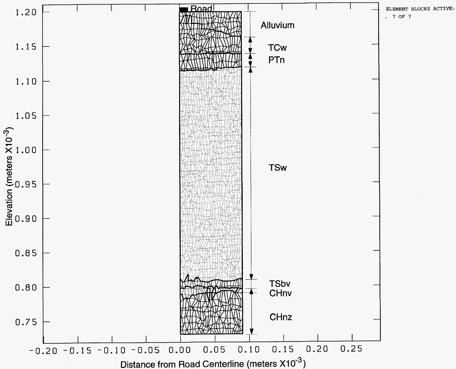
Saturation Near UE25 a#1 Resulting from Road Watering N-S Transect, Seed #3, Alluvium Conductivity per ESF Analyses Computational Grid
