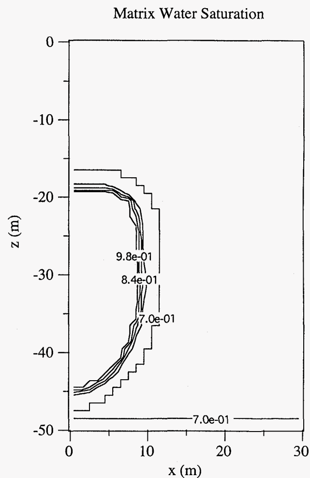
Figure 5.4-4. Water saturation contours in the fracture and matrix elements of TSw2 during flooding of the ESF tunnel using the dual-permeability model. The fracture aperture is 25 \mu\text{m} and the time is 30 days.
