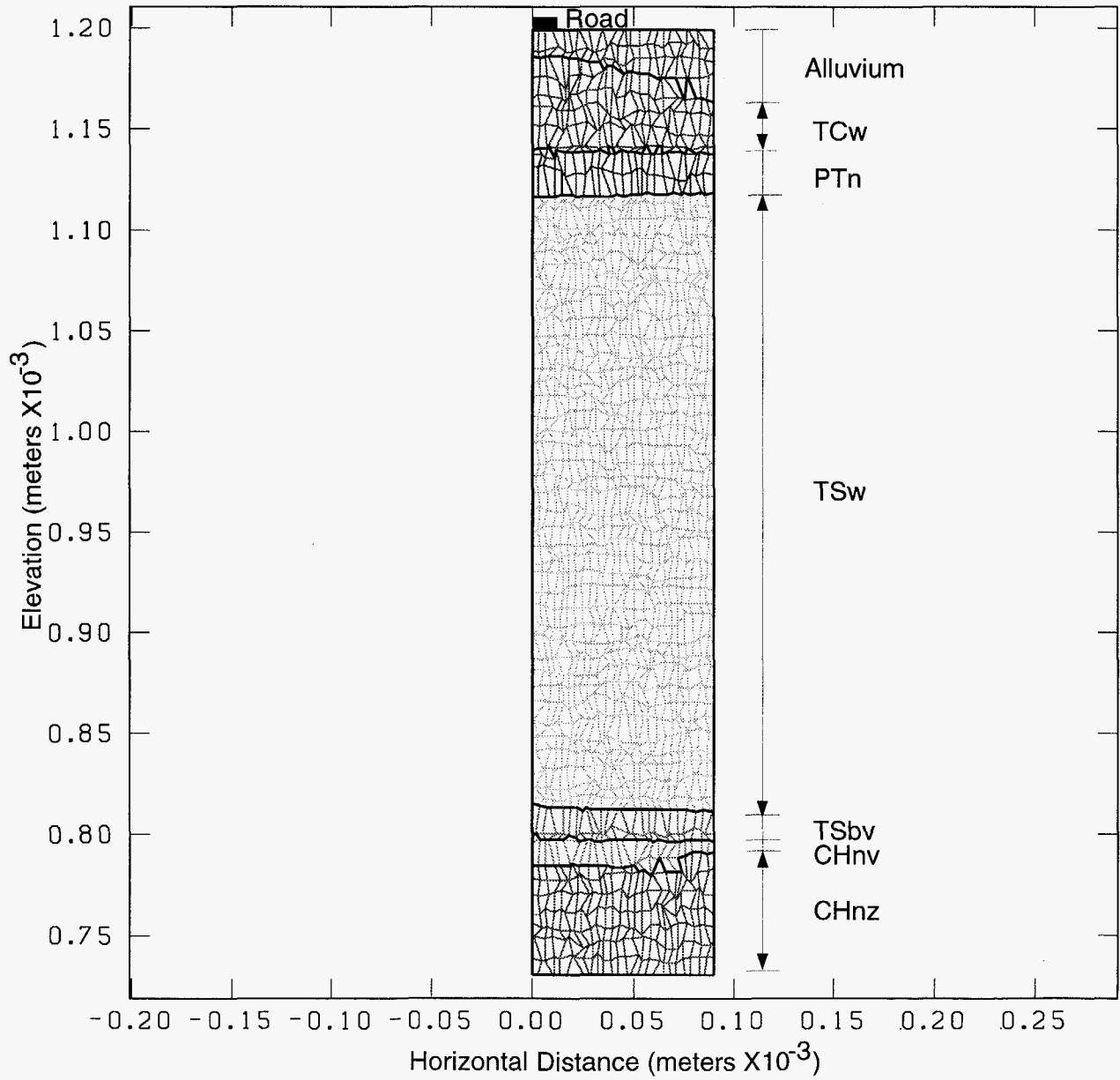
Saturation Near UE25 #1 Resulting from Road Watering N-S Transect, Seed #2, Alluvium Conductivity per ESF Analyses Computational Grid
