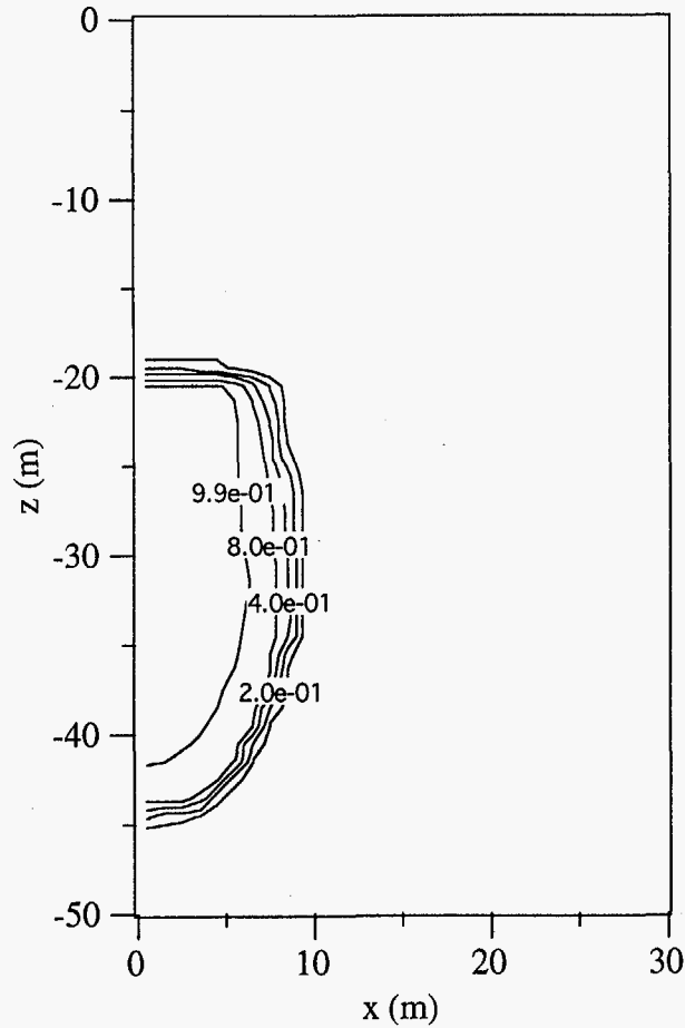
Fracture Water Saturation
