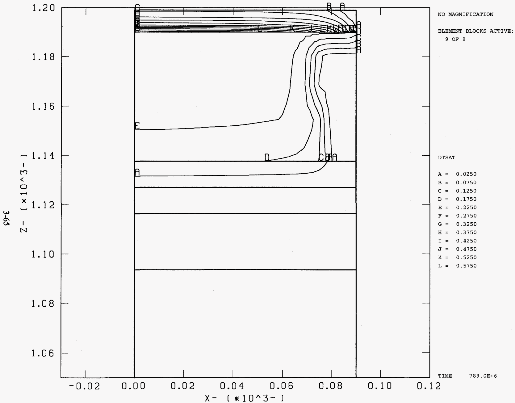
Change in Saturation from In Situ Conditions Ptn Modeled as per PACE-90 Studies Time=25 Years
