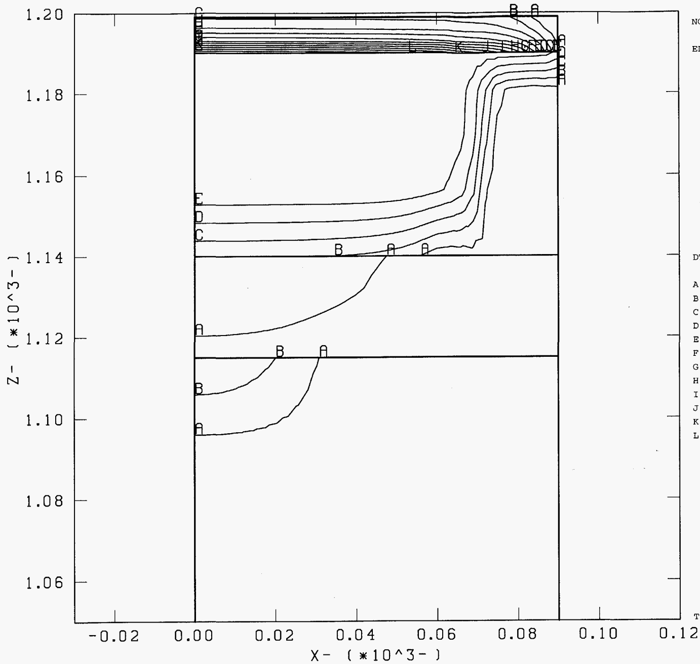
Change in Saturation from In Situ Conditions Ptn as in ESF Analysis #12 Calculations Time=25 Years
