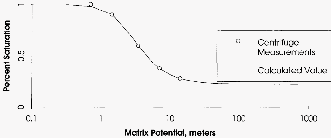
Figure 3.1-1: Moisture Retention Curve for Pah Canyon Member (Sample 4-5H, Flint and Flint, 1990)
