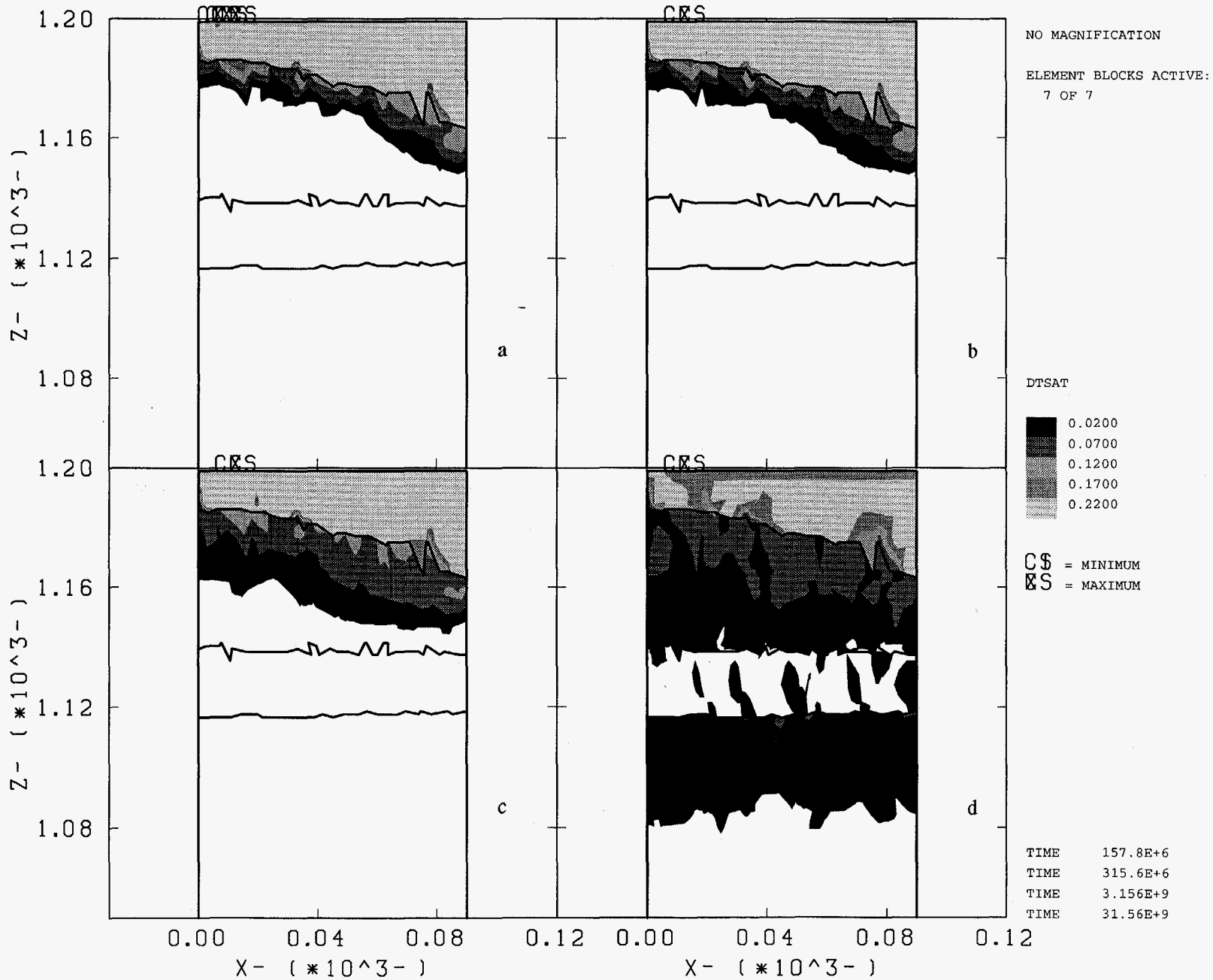
Delta Saturation Near UE25 a#1 N-S Transect, Seed #2, Alluvium Conductivity per ESF Analyses Times=(a) 5 Years (b) 10 Years (c) 100 Years (d) 1000 Years
