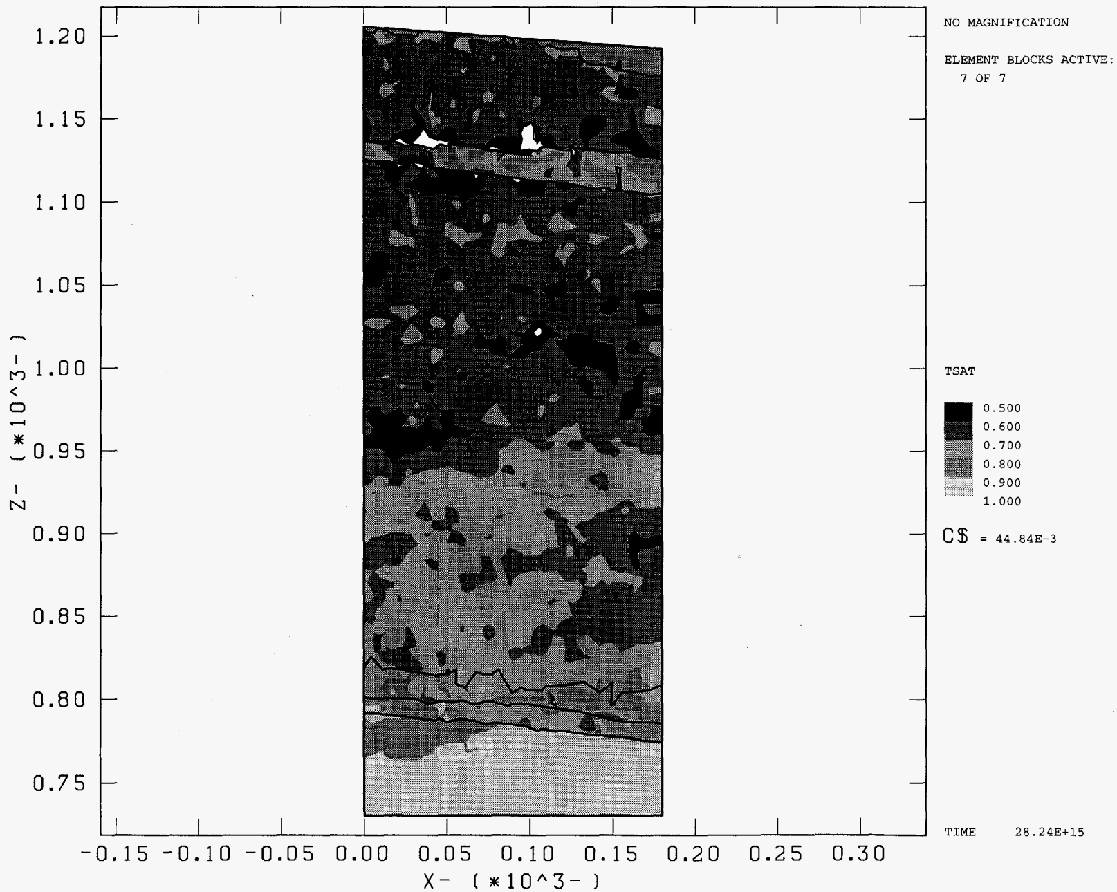
Saturation Near UE25 a#1 Resulting from Road Watering E-W Transect, Seed #1, Alluvium Conductivity per 92% Sand In Situ Conditions
