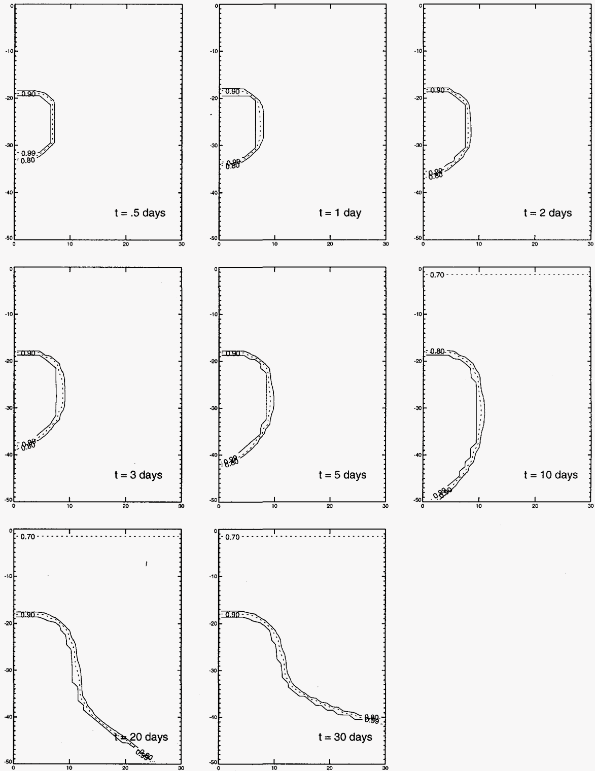
Figure 5.3-6 Equivalent continuum model prediction of saturation front movement over 30 days for 30 μm aperture fractures in TSw2 tuff.
