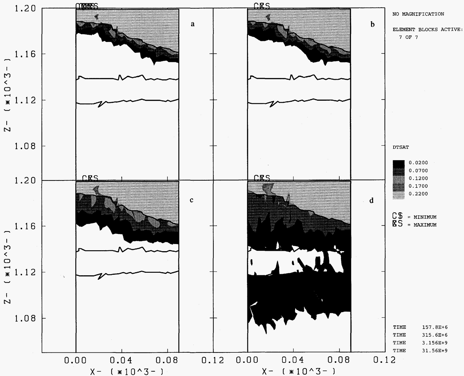
Delta Saturation Near UE25 a#1 N-S Transect, Seed #1, Alluvium Conductivity per ESF Analyses Times=(a) 5 Years (b) 10 Years (c) 100 Years (d) 1000 Years
