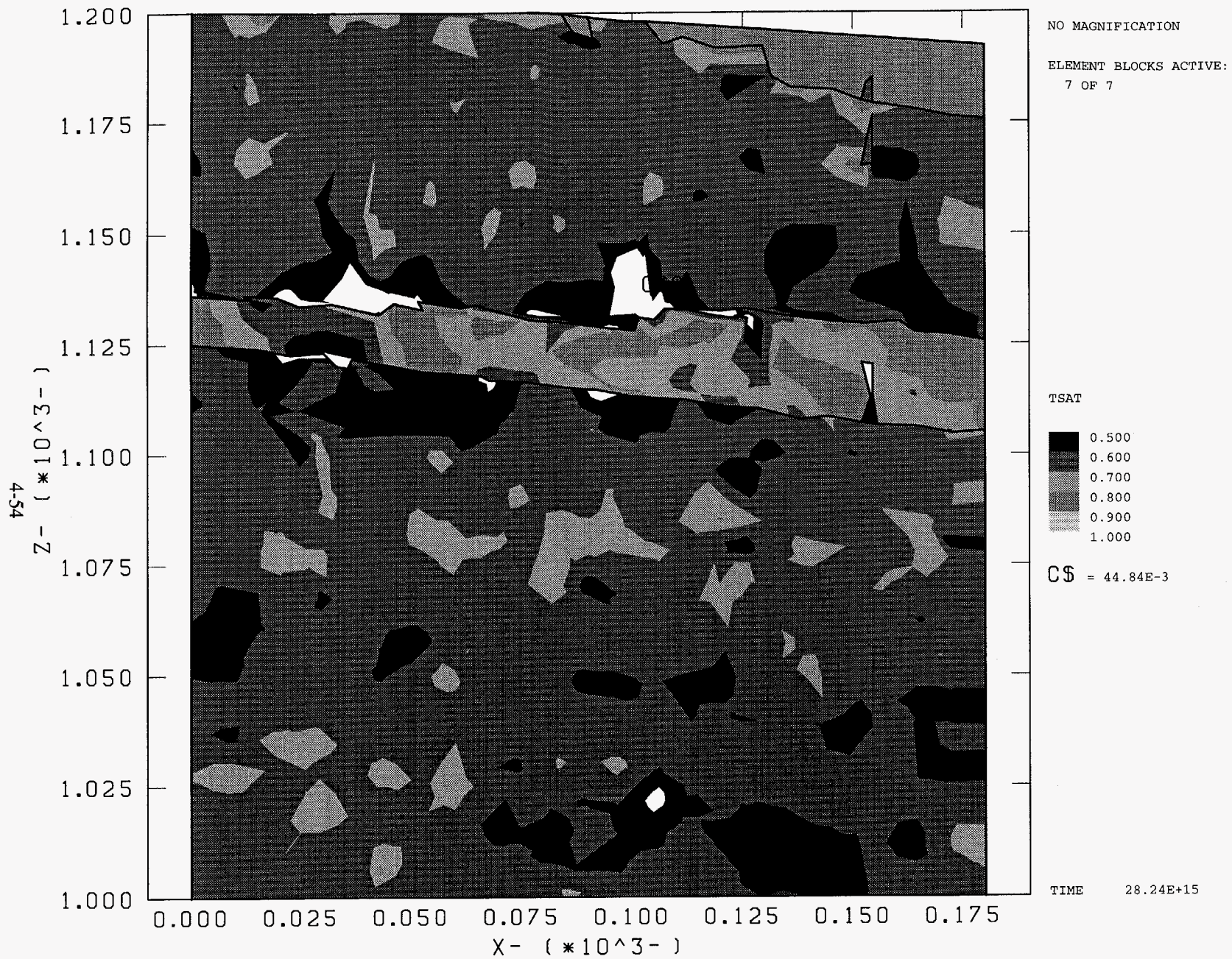
Saturation Near UE25 a#1 Resulting from Road Watering E-W Transect, Seed #1, Alluvium Conductivity per 92% Sand In Situ Conditions
