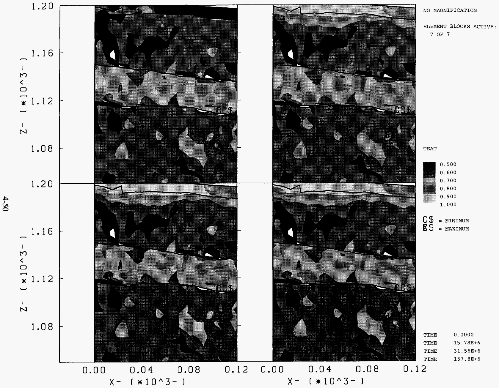
Saturation Near UE25 a#1 Resulting from Road Watering E-W Transect, Seed #2, Alluvium Conductivity per ESF Analyses Times=(a) In Situ (b) 6 Months (c) 1 Year (d) 5 Years
