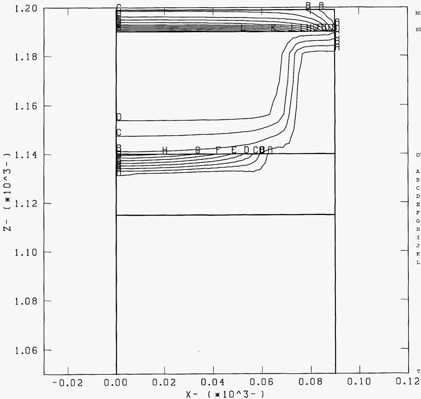
Change in Saturation from In Situ Conditions Ptn Modeled as USW G-4 Time=25 Years
