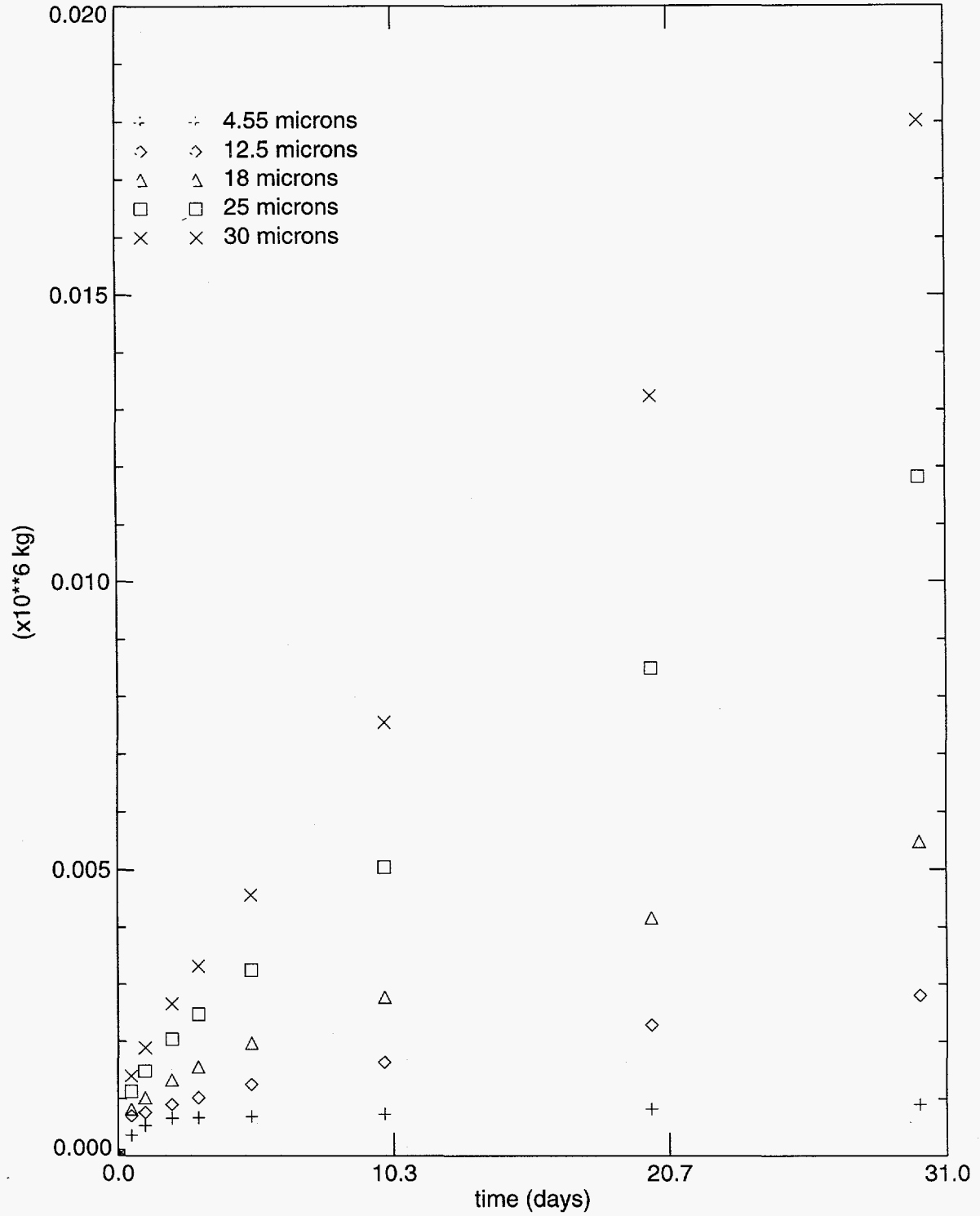
Figure 5.3-7 Equivalent continuum model prediction of the mass of water entering half of the tunnel wall rock for each of five fracture aperture calculations using TOUGH2.
