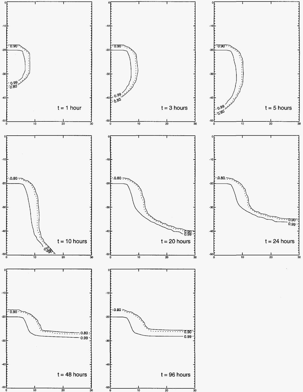
Figure 5.3-9 Equivalent continuum model prediction of saturation front movement over 4 days for 100 μm aperture fractures in TSw2 tuff.
