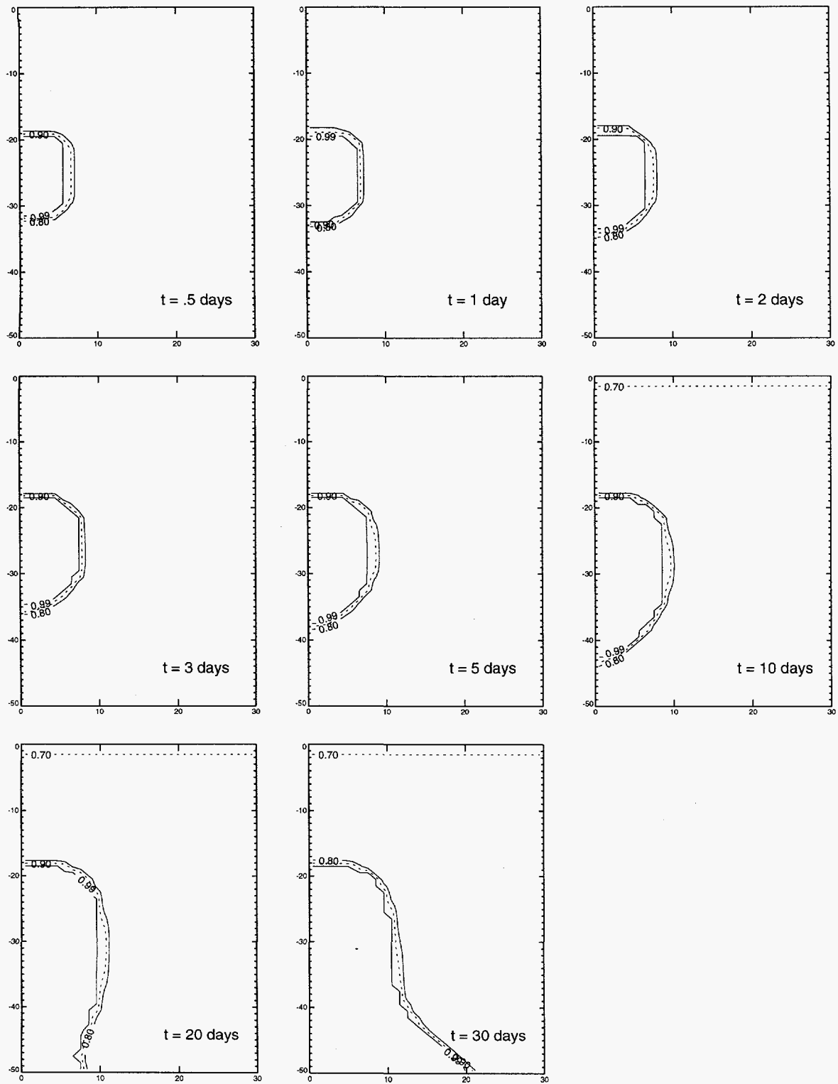
Figure 5.3-5 Equivalent continuum model prediction of saturation front movement over 30 days for 25 \mu\text{m} aperture fractures in TSw2 tuff. Ponding at 30 days is a result of the imposed no flow lower boundary condition.
