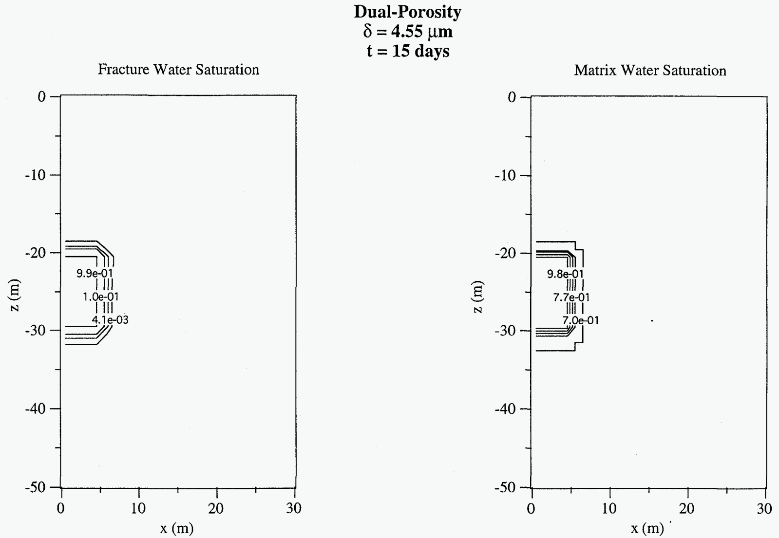
Figure 5.4-1. Water saturation contours in the fracture and matrix elements of TSw2 during flooding of the ESF tunnel using the dual-porosity model. The fracture aperture is 4.55 \mu\text{m} and the time is 15 days.
