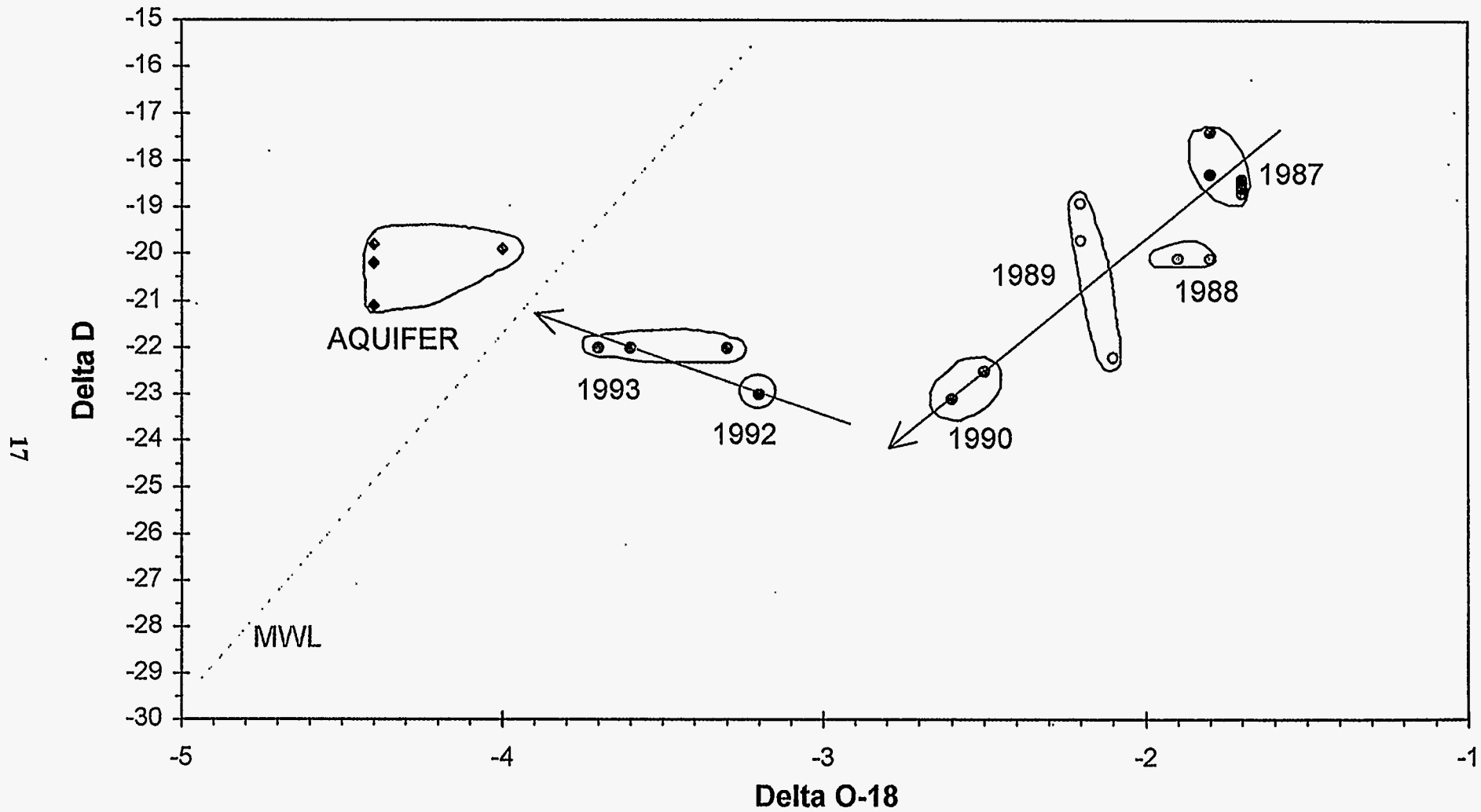
Figure 6 Isotopic evolution of brine taken from fill holes, 1987-1993, showing trend from connate to meteoric, with a significant change occurring in about 1991, approximately the same time of formation of the first sinkhole. The analyses plotted here show the rate of change in hydrogen (D, deuterium) vs ^{18}\text{O} (oxygen) stable isotopes.
