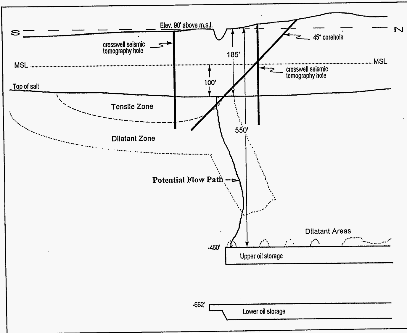
Figure 8 Geomechanical modeling by Ehgartner (1993) and Hoffman (1994) showed mechanism for crack development in tension that would develop over mined openings after a number of years, and progressing through weakened dilatant zones. Based largely on the results of this modeling, crosswell seismic tomography was conducted and angled boreholes were planned to intersect such features.
