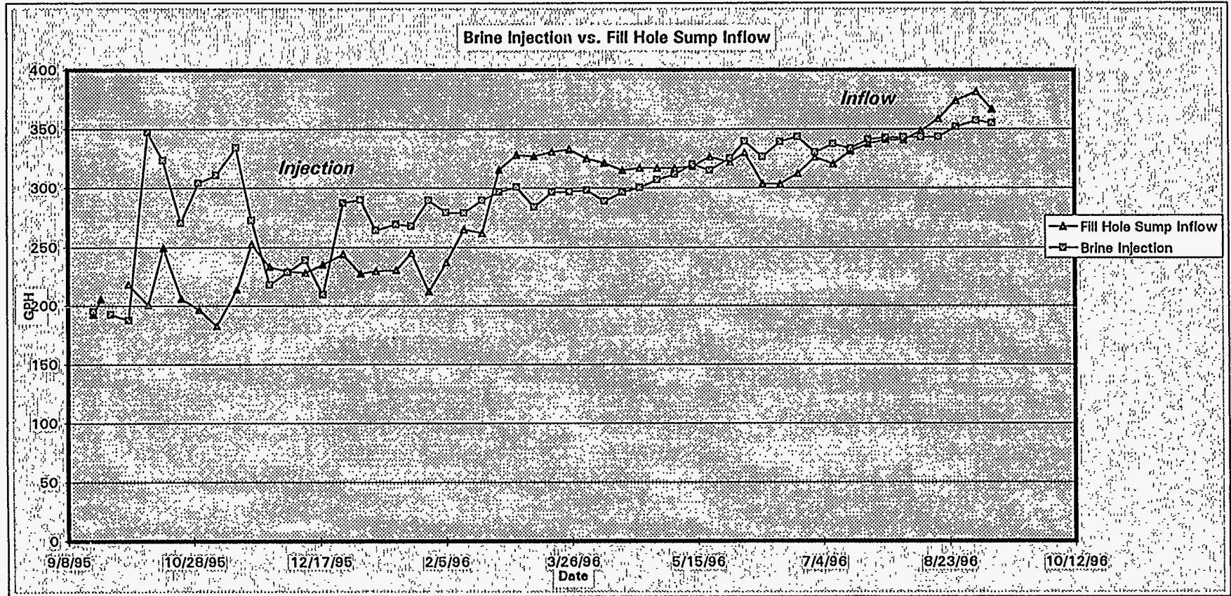
Figure 11 Comparison of brine inflow rates into fill hole sump with brine injected into sinkhole throat. Respective values and generally increasing trend are similar, suggesting possible correlation with regard to origin.
