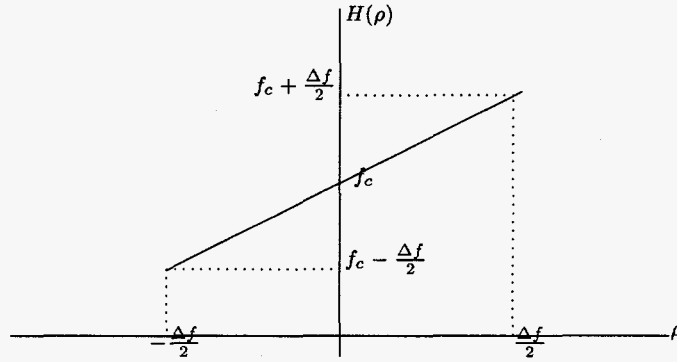
Figure 5: Frequency domain specifications of filter for SAR data.
