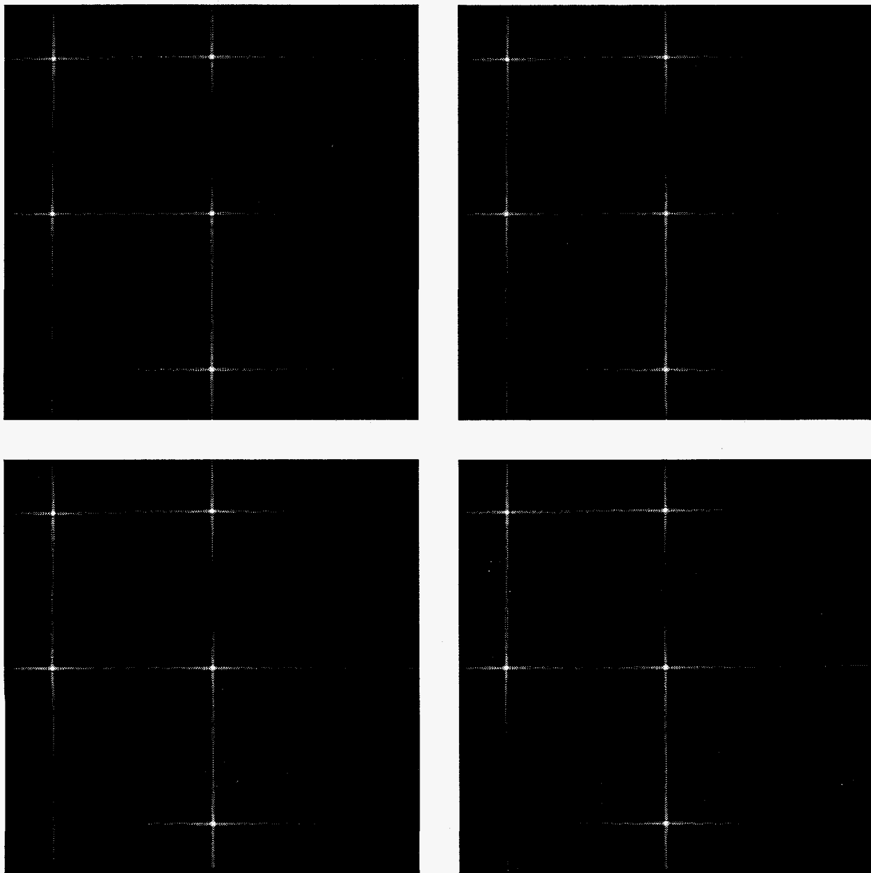
Figure 9: Images formed from "A" parameters. (a) IW. (b) XW. (c) CBP. (d) WX. (labeled clockwise from upper left)
