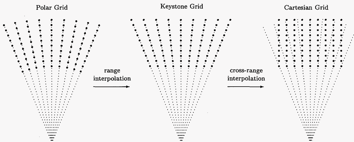
Figure 2: Two steps in interpolation process first yields a keystone grid, then a cartesian grid.
