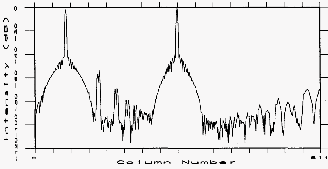
Figure 15: Center row from CBP "D" image, N_s = 332 , M = 1024 .
