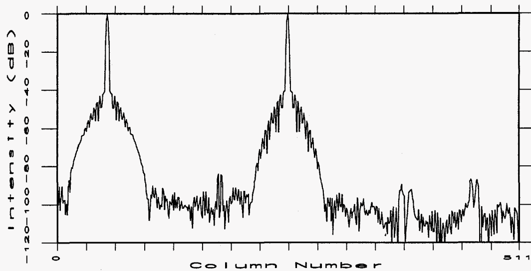
Figure 17: Center row from CBP "D" image, N_s = 332 , M = 4096 .
