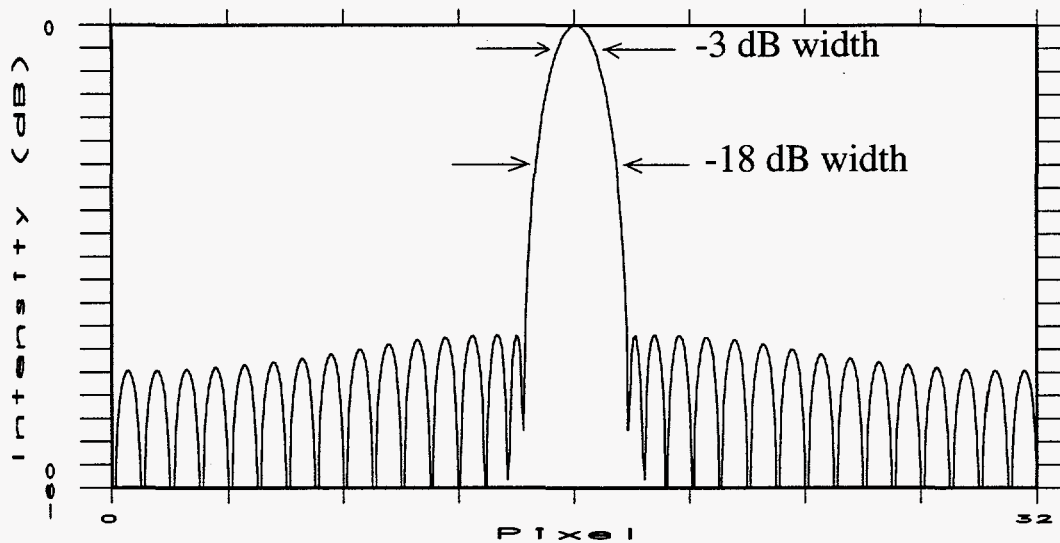
Figure 7: Taylor window IPR showing quality measures.
