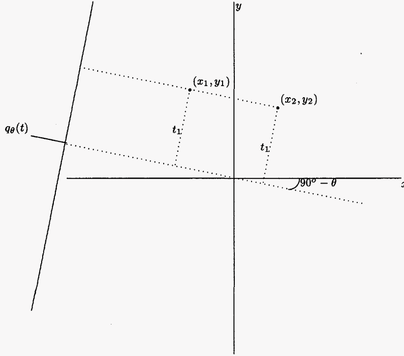
Figure 4: Image and filtered projection arrangement for backprojection step.
