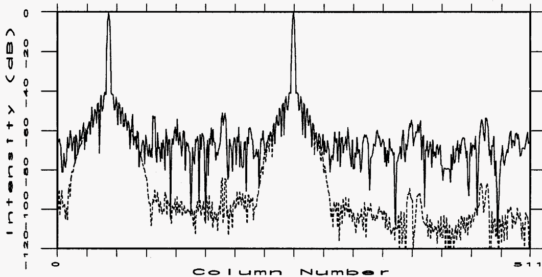
Figure 20: Center row from CBP "D" image, N_s = 332 , M = 4096 . Solid line=nearest neighbor interpolation; dashed line=linear interpolation.
