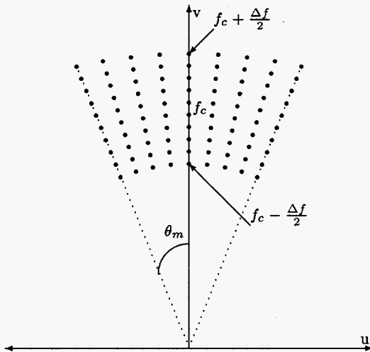
Figure 1: Fourier-domain annulus region where SAR collects data.
