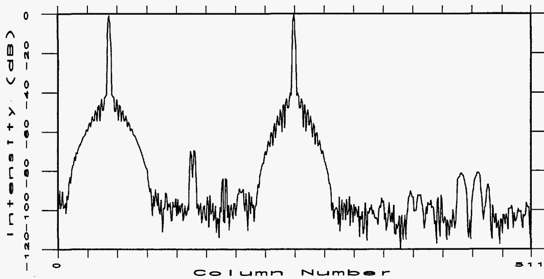
Figure 16: Center row from CBP "D" image, N_s = 332 , M = 2048 .
