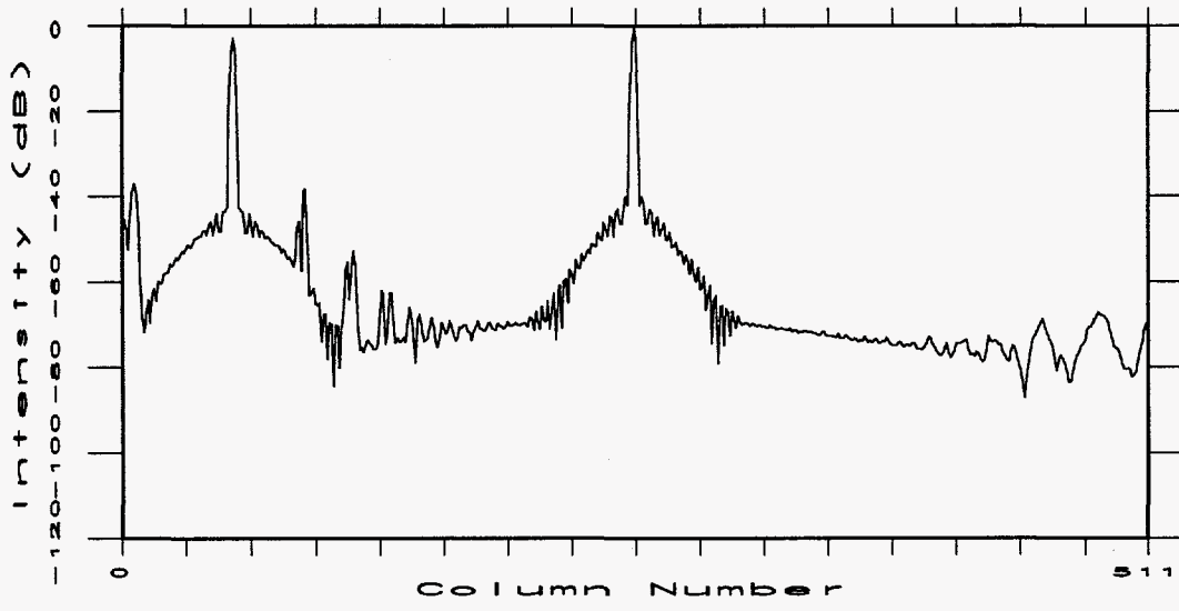
Figure 14: Center row from CBP "D" image, N_s = 332 , M = 512 .
