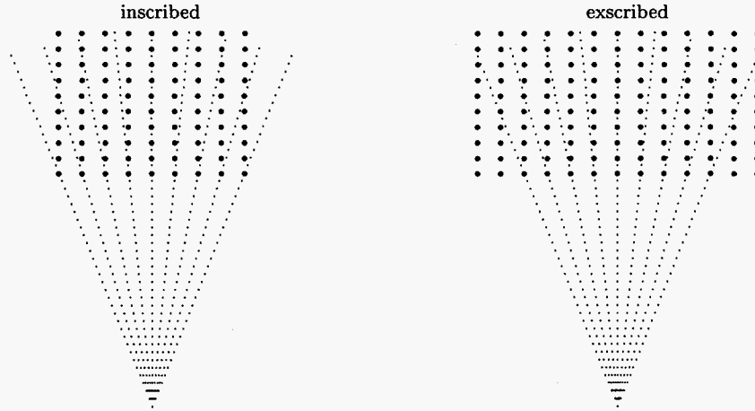
Figure 3: Grid point locations for inscribed and exscribed rectangles.
