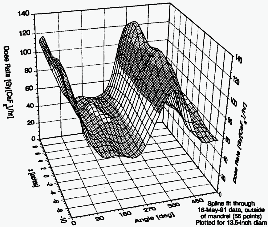
Figure A.7: Aging radiation dose rate for complete cable specimens—outside of cable wraps ( 0^\circ corresponds to x = 6.75 inches, y = 0 inches).
