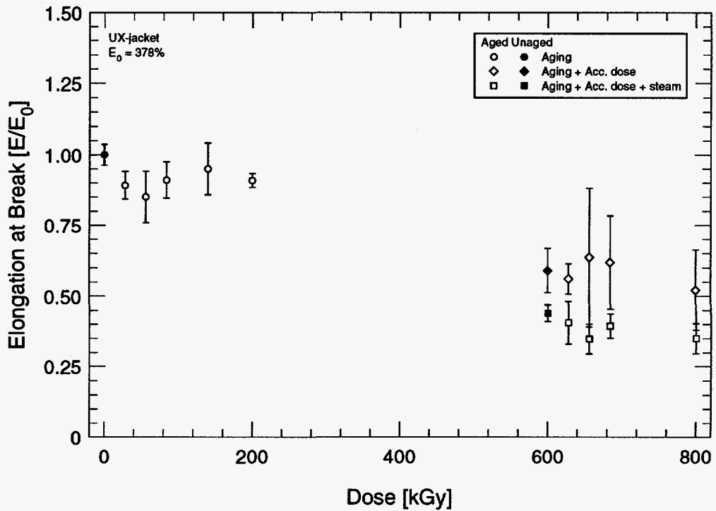
Figure 3.7: Elongation for U.S. XLPO cable—Hypalon jacket.
