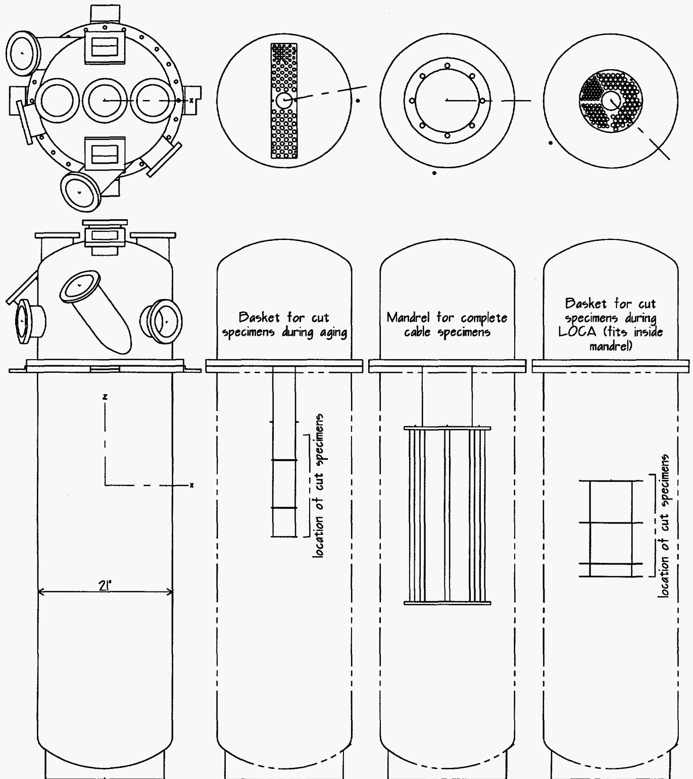
Figure 2.4: Detail of the test chamber and sketches of the two baskets used to hold cut specimens and the mandrel on which the complete specimens were mounted—drawn to scale.
