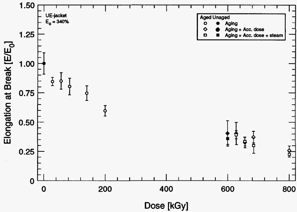
Figure 3.6: Elongation for U.S. EPR cable—Hypalon jacket.
