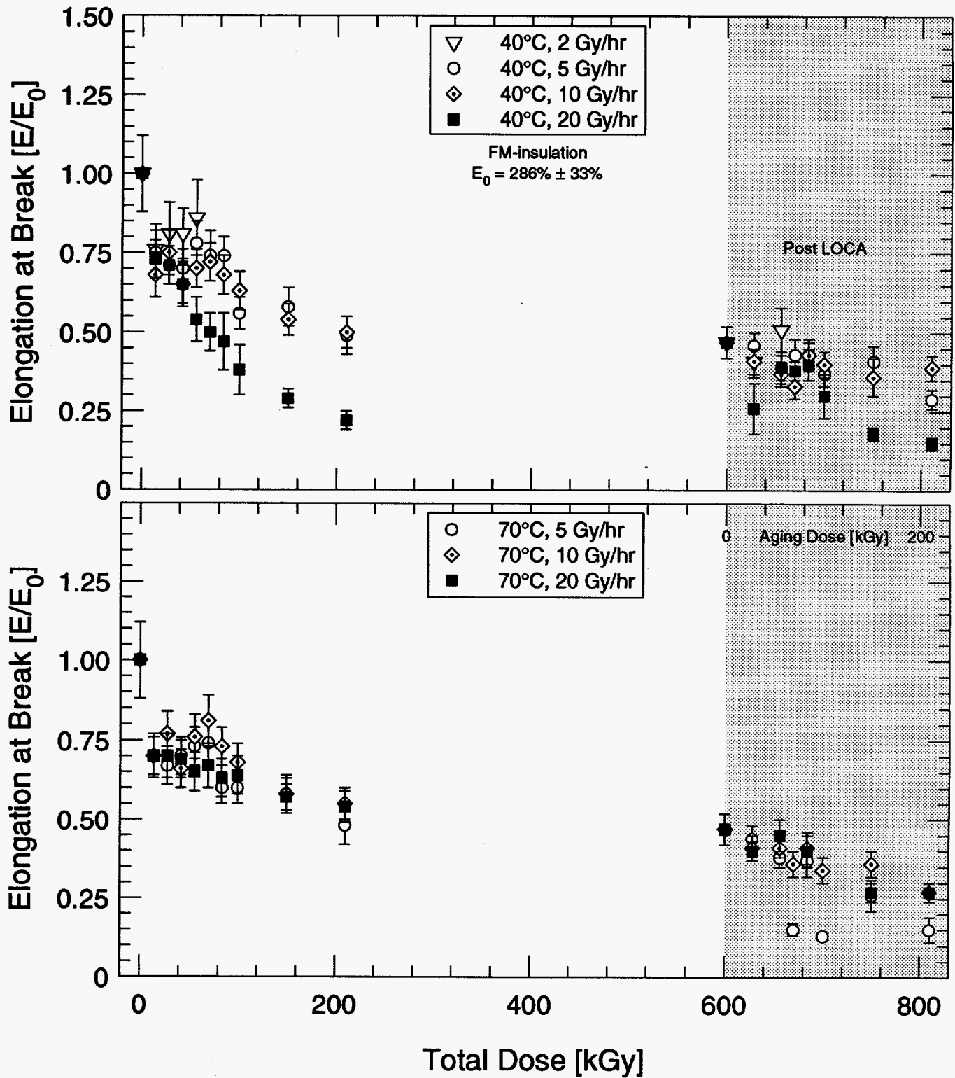
Figure 5.13: Elongation at break during aging and after LOCA simulation versus total dose for French EPR cable—EPR insulation.
