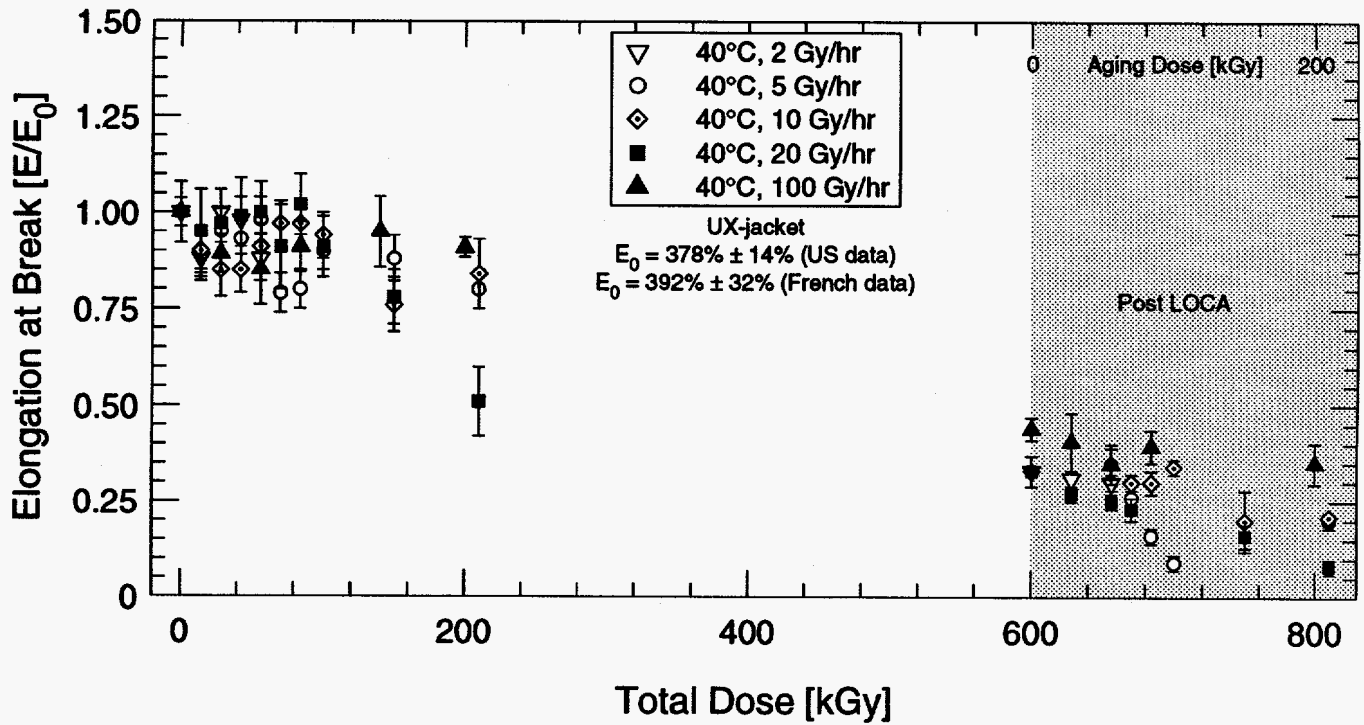
Figure 6.1: Comparison of U.S. and French elongation at break data versus total dose for U.S. XLPO cable—Hypalon jacket.
