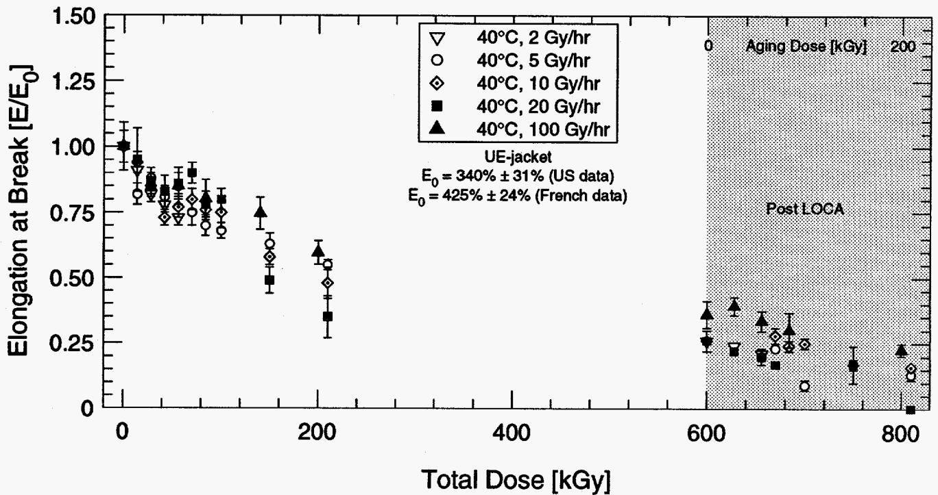
Figure 6.2: Comparison of U.S. and French elongation at break data versus total dose for U.S. EPR cable—Hypalon jacket.
