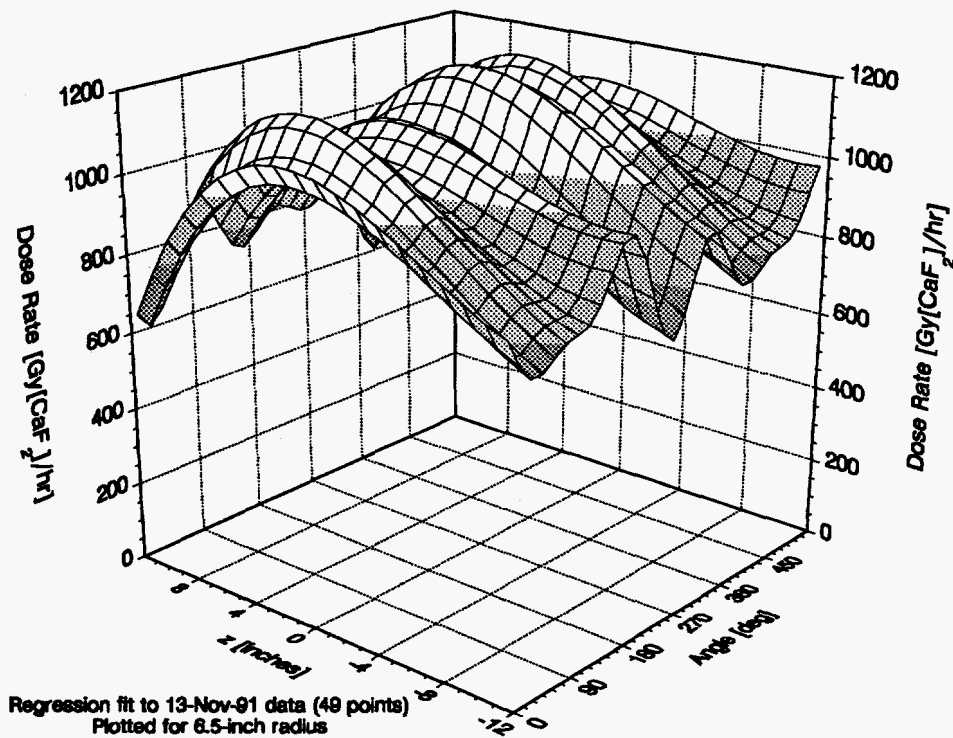
Figure A.10: Accident radiation dose rate—regression fit to data ( 0^\circ corresponds to x = 6.5 inches, y = 0 inches).
