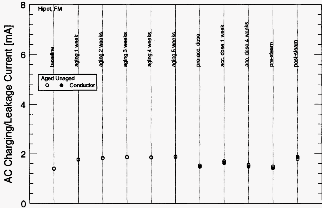
Figure 3.17: AC leakage current for French EPR cable.
