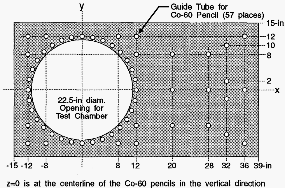
Figure A.2: Plan view of large chamber cobalt fixture showing the fixture coordinate system and possible cobalt source locations.
