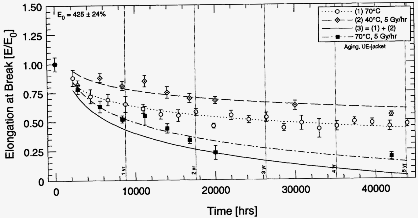
Figure 5.4: Elongation at break versus time for U.S. EPR cable—Hypalon jacket.
