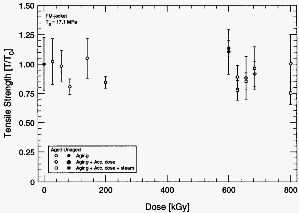
Figure 3.11: Tensile strength for French EPR cable—Hypalon jacket.
