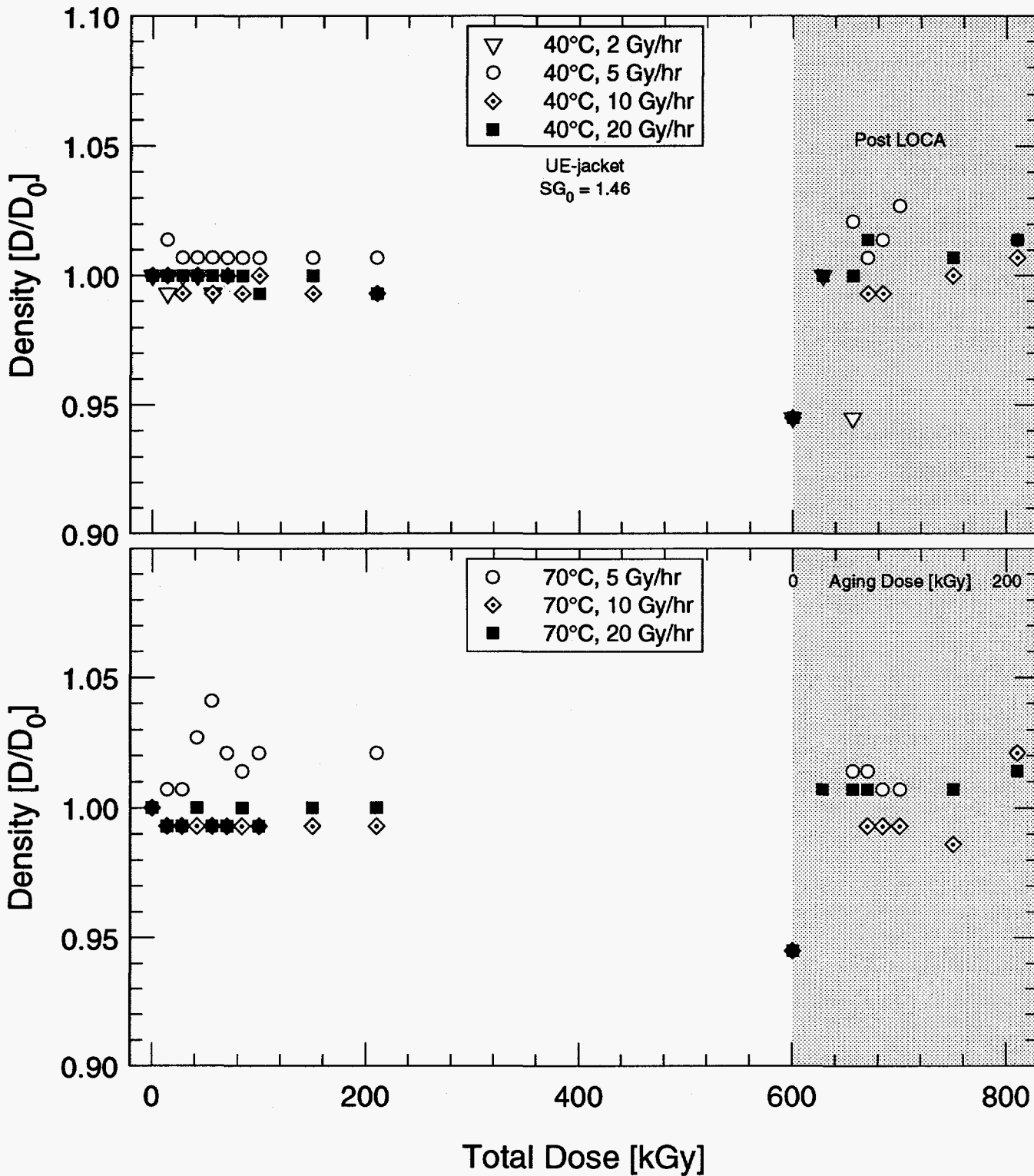
Figure 5.17: Density during aging and after LOCA exposure versus total dose for U.S. EPR cable—Hypalon jacket.
