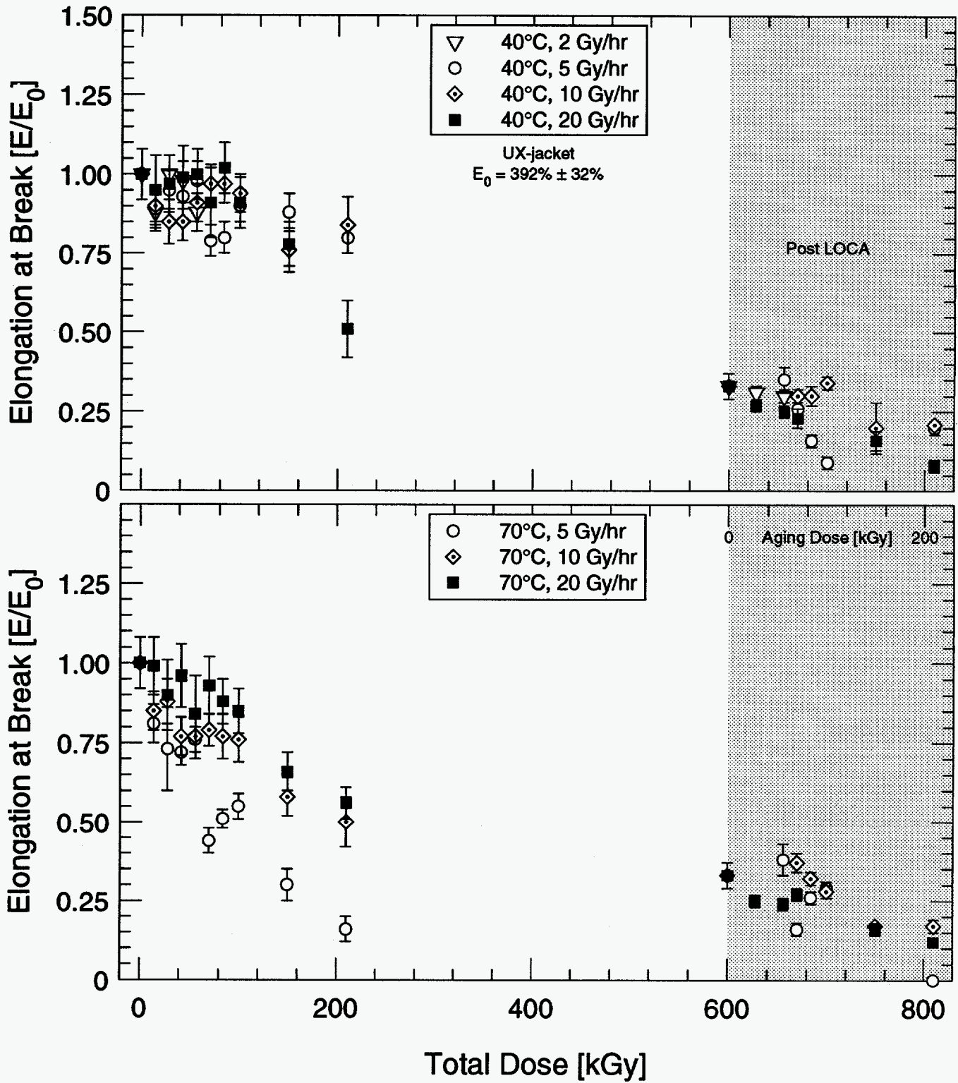
Figure 5.1: Elongation at break during aging and after LOCA simulation versus total dose for U.S. XLPO cable—Hypalon jacket.
