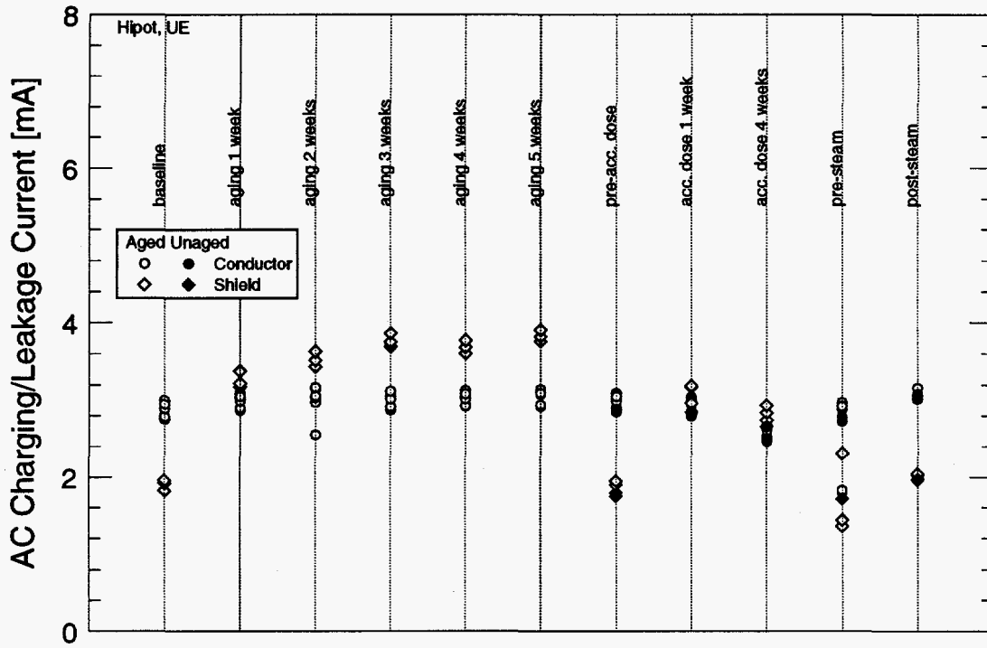
Figure 3.19: AC leakage current for U.S. EPR cable.
