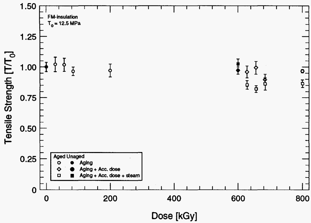
Figure 3.14: Tensile strength for French EPR cable—EPR insulation.
