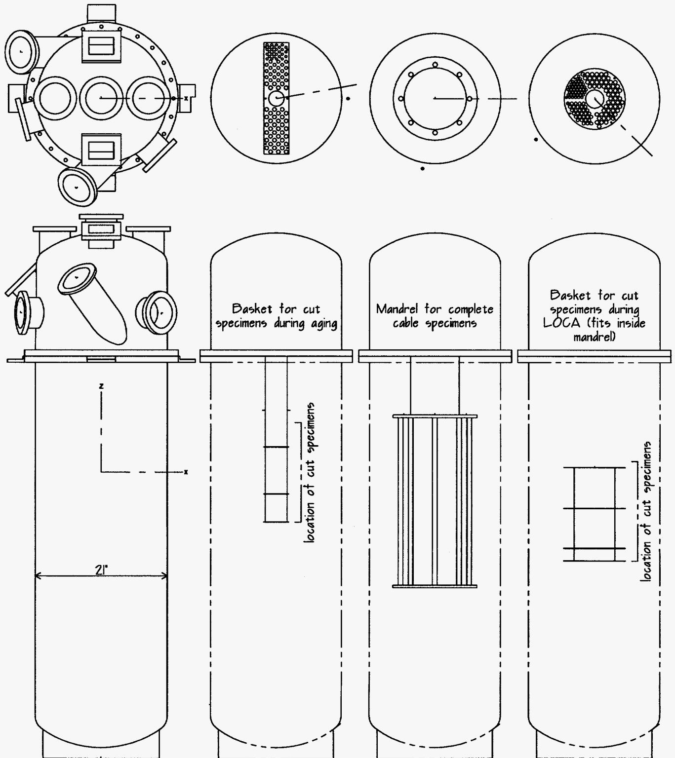
Figure A.4: Detail of the test chamber and sketches of the two baskets used to hold cut specimens and the mandrel on which the complete specimens were mounted—drawn to scale.
