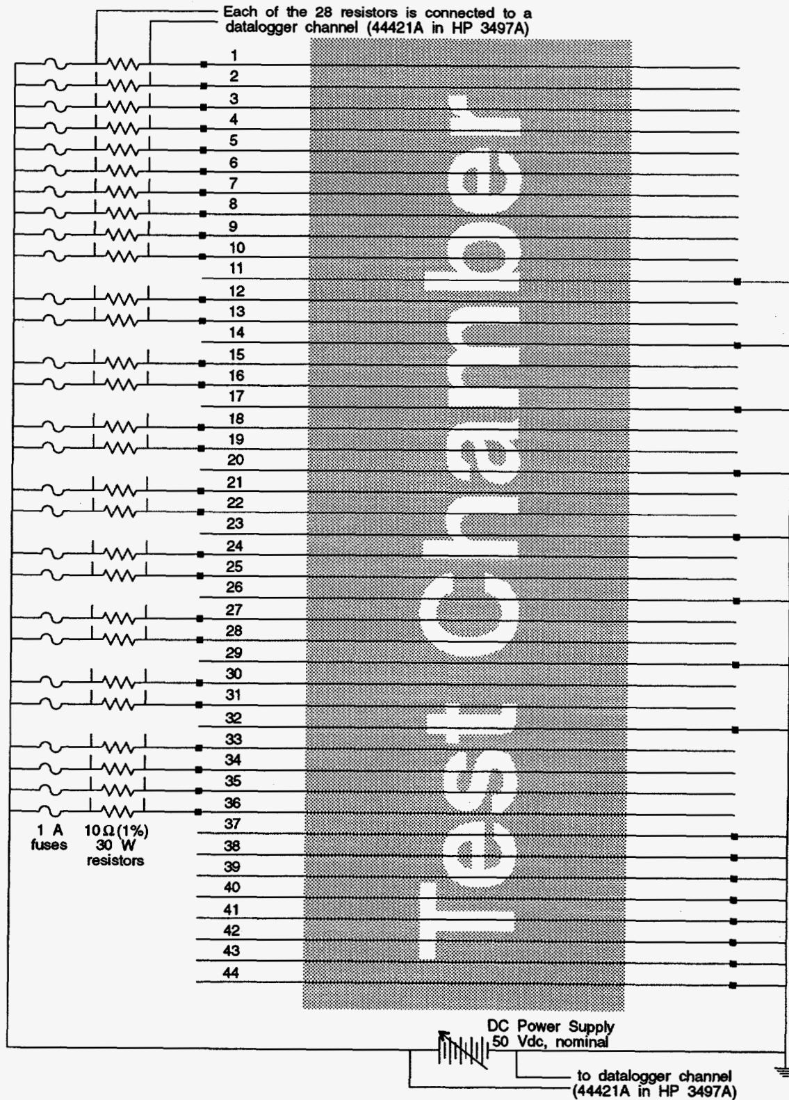
Figure 2.12: Circuitry used to measure continuous insulation resistance during the accident steam exposure.
