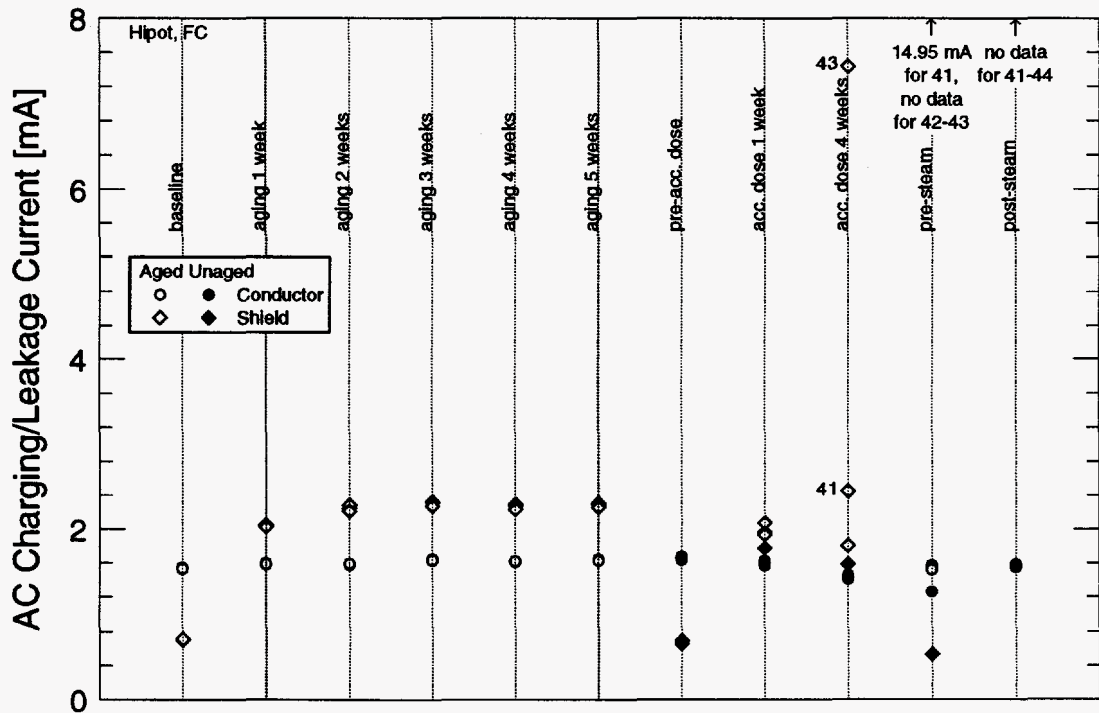
Figure 3.18: AC leakage current for French PE cable.
