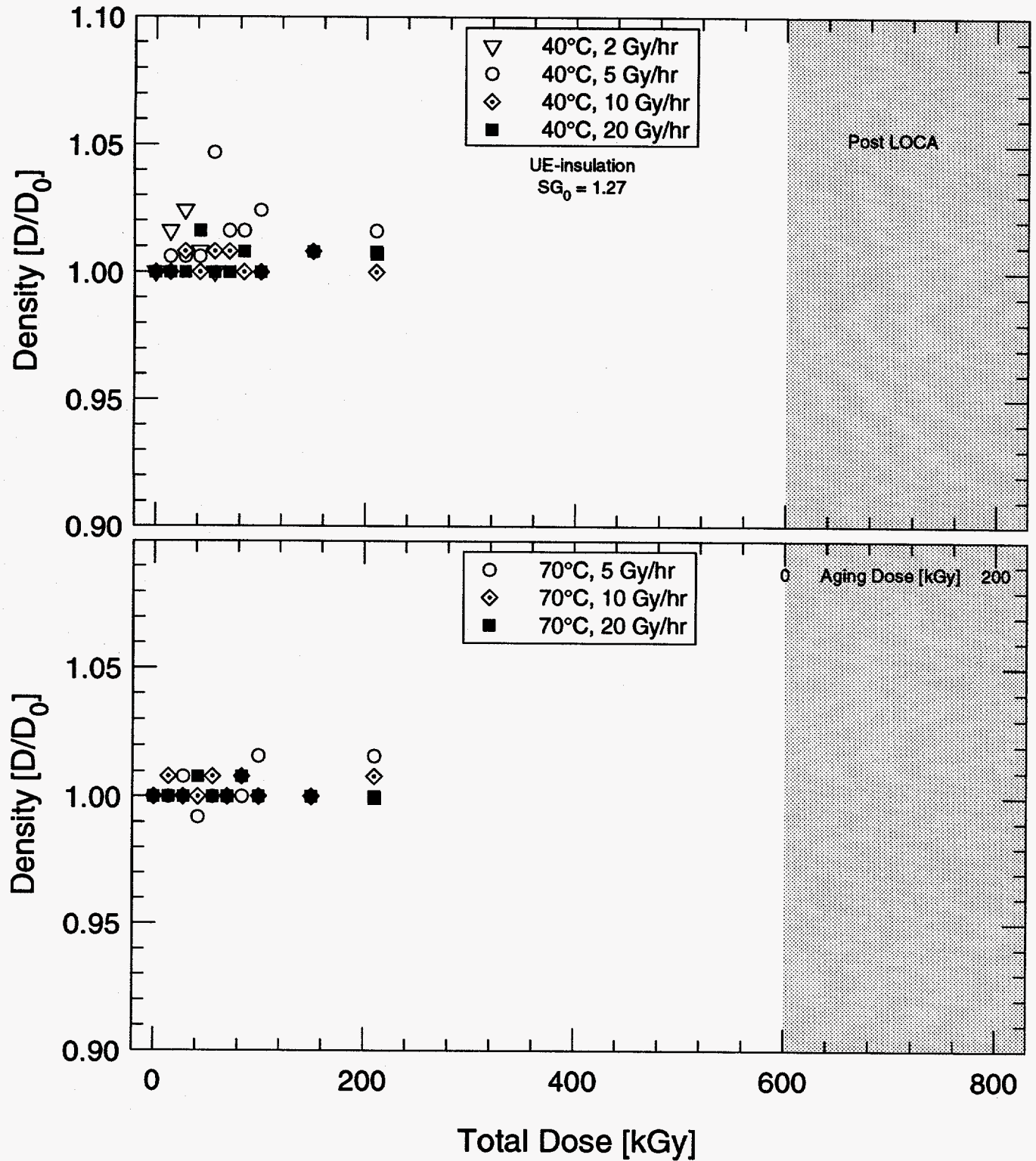
Figure 5.18: Density during aging versus total dose for U.S. EPR cable—FR-EPDM insulation.
