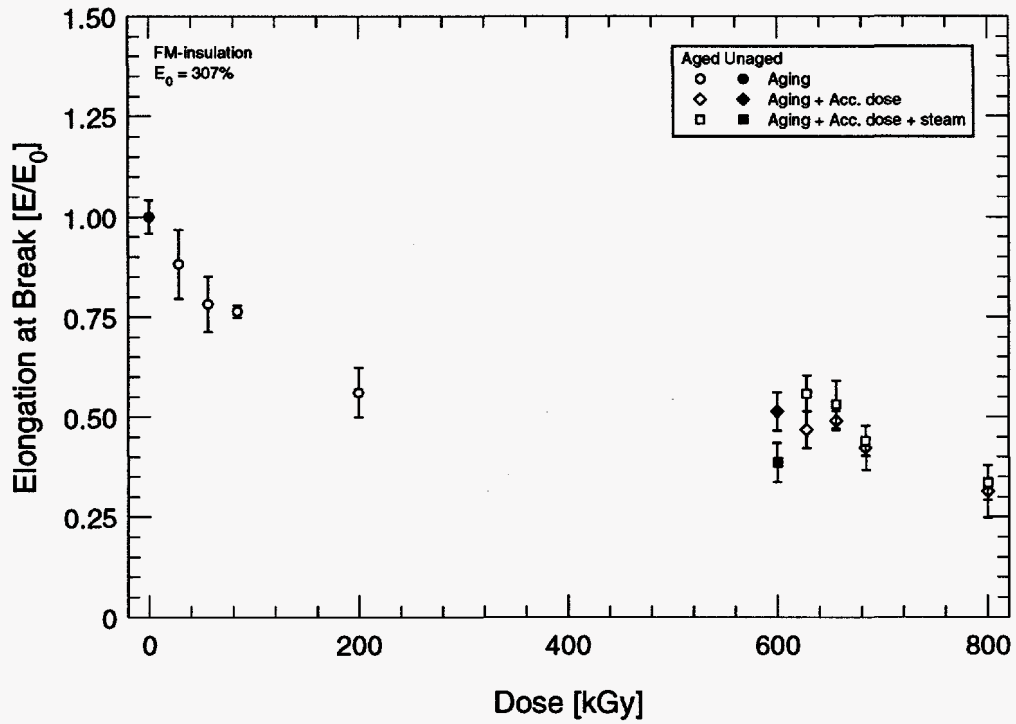
Figure 3.8: Elongation for French EPR cable—EPR insulation.
