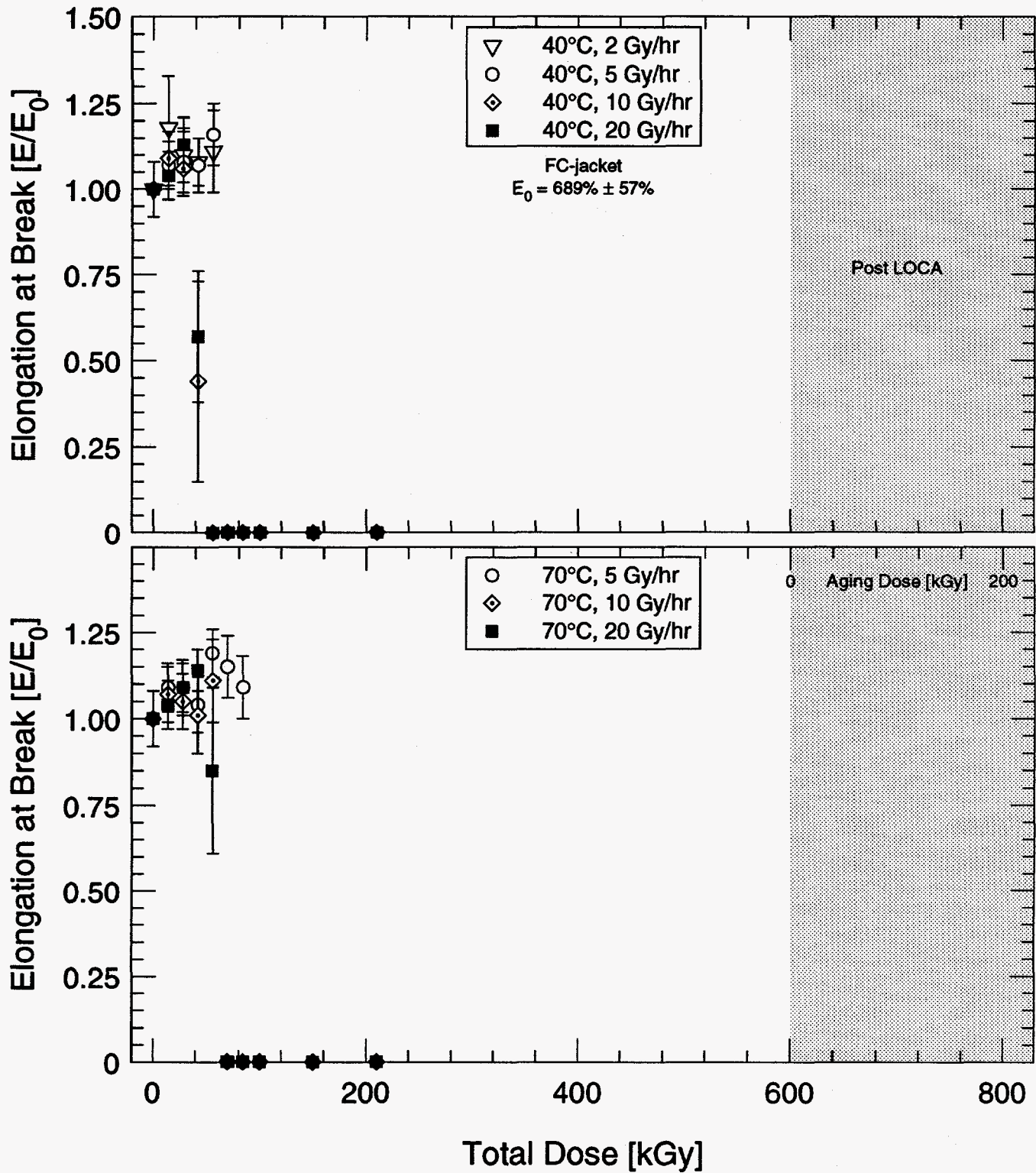
Figure 5.7: Elongation at break during aging versus total dose for French PE cable—PE jacket.
