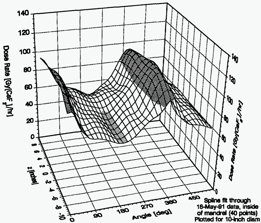
Figure A.8: Aging radiation dose rate for complete cable specimens—inside of cable wraps ( 0^\circ corresponds to x = 5 inches, y = 0 inches).
