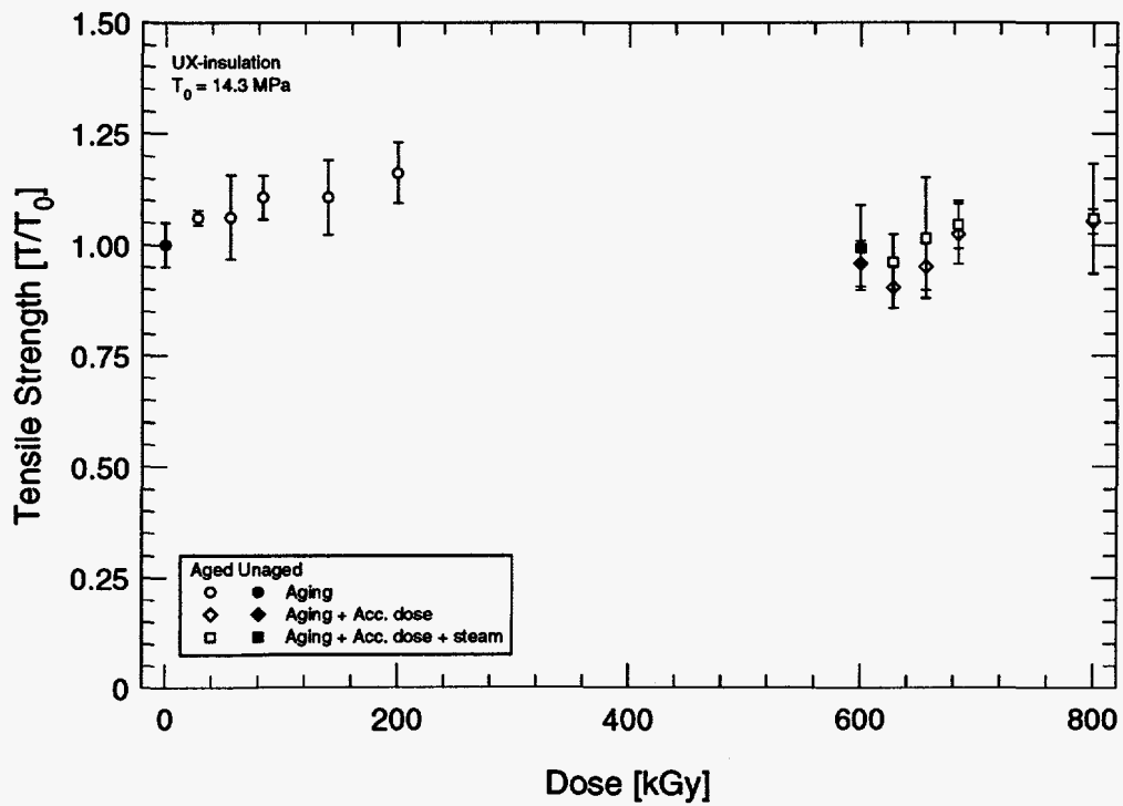
Figure 3.16: Tensile strength for U.S. XLPO cable—XLPE insulation.
