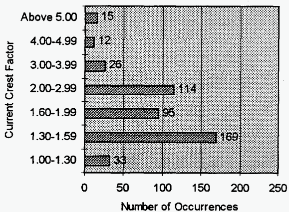
Fig. 4. Mathematical distribution of phase current crest factors.
