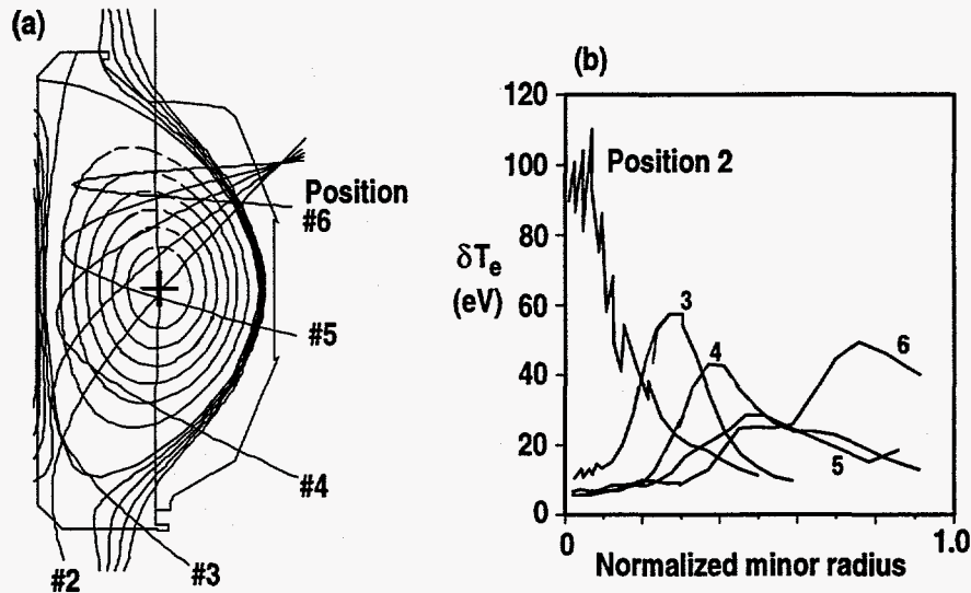
Fig. 3. The rf beam can be steered poloidally in the tokamak upper half plane to change the power deposition location without changing plasma parameters. Modulating the generated rf power allows the deposition profile to be determined from the time dependence of the ECE signals at different locations. The profiles in (b) for different wave trajectories shown projected to a single plane in (a) indicate the general location of the deposition, but due to low modulation frequencies used, transport effects comprise the measurement and broaden the apparent profile.
