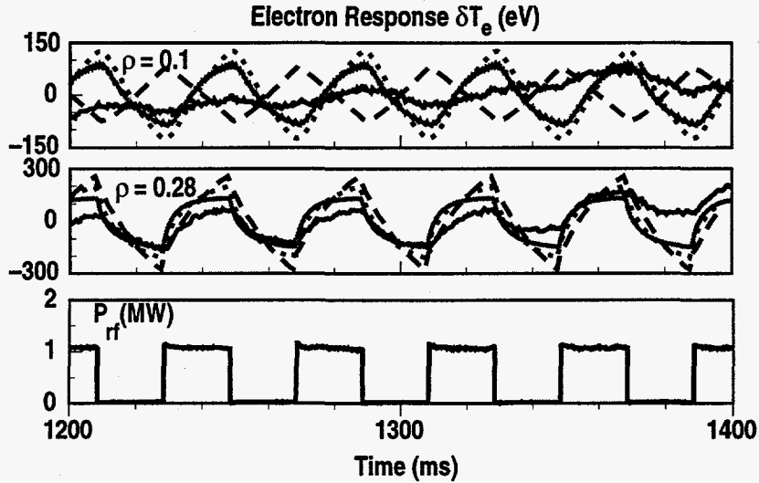
Fig. 4. The envelope of modulated rf is shown along with the response of the ECE diagnostic at two different values of the normalized flux. The phase of the resulting T_e(t) is compared with the measurements for three different transport theories at two different values of normalized flux. The phase of one of the transport model predictions is not consistent with the data at \rho = 0.1 , but two other models are not ruled out by the data. The experimental measurements are the solid black lines and the theoretical predictions are dotted, dashed, and gray lines. The data for \rho = 0.1 clearly show the T_e modulation, but are close to the limit of reliable detectability at presently available power levels.
