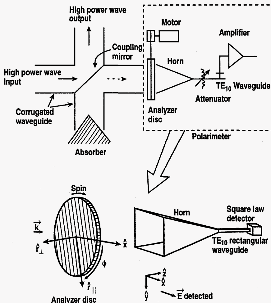
Fig. 6. The polarimeter consists of a rotating birefringent plate and a polarization sensitive detector. The leaky mirror couples a small fraction of the beam power, about -40 dB, to the polarimeter.
