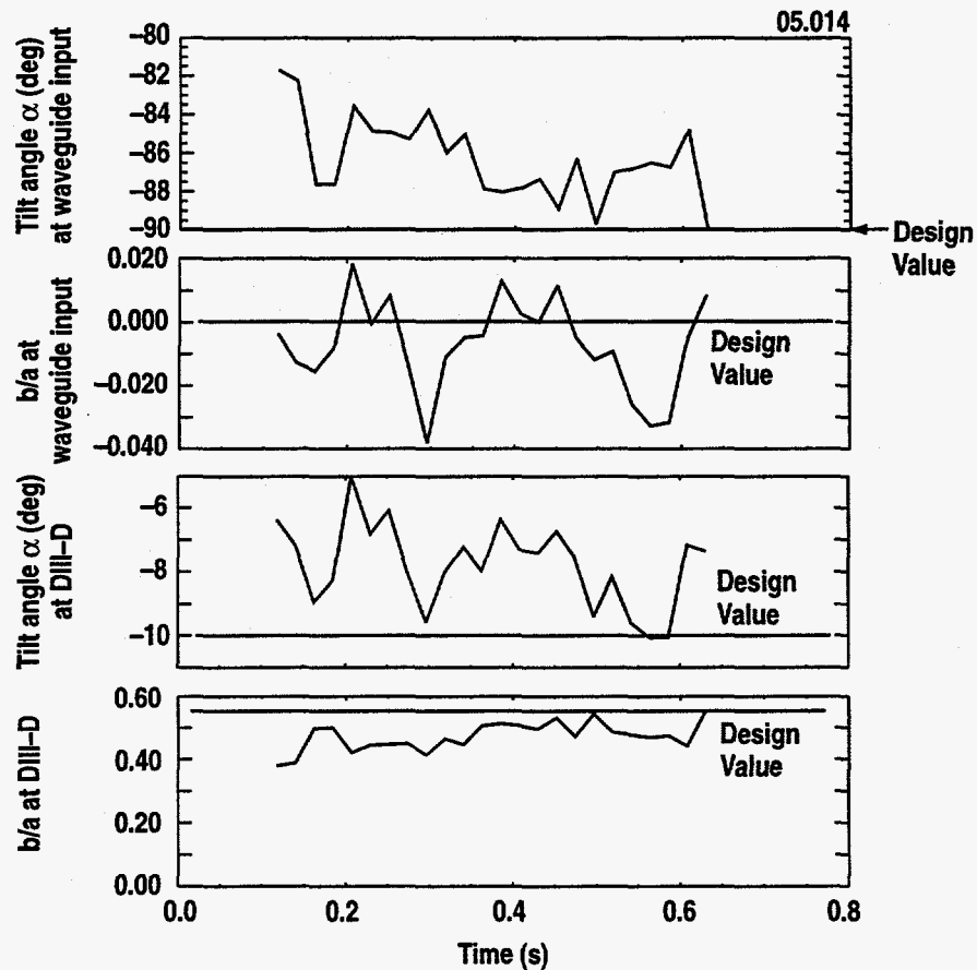
Fig 8. The performance of the entire Katya line was measured at the sixth miter and demonstrates that the polarizers produce close to the desired b/a = 0.55 and a = -10^\circ required to generate pure X-mode at the plasma. The scatter in the data indicates the accuracy of the polarization measurement.
