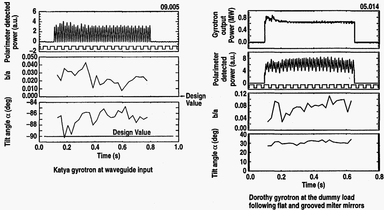
Fig 7. Polarization measurements at the input to the waveguide for the Gycom gyrotron, Katya, showed good linear polarization with about 3^\circ tilt from the horizontal. Similar measurements for the CPI gyrotron, Dorothy, made after reflection of the beam from one flat mirror and one grooved miter mirror showed linear polarization with the polarization axis rotated by about 30^\circ due to reflection from the grooved mirror.
