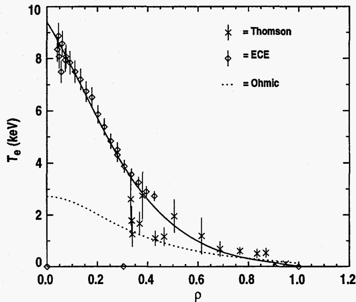
Fig. 2. Electron heating by electron cyclotron waves is extremely efficient. At moderately low density, 1 MW of rf power resonant in the discharge center yielded T_e(0) = 11 keV, the present record value for DIII-D. The profile above was for 0.4 MW at \bar{n}_e \sim 5 \times 10^{18}/\text{m}^3 .
