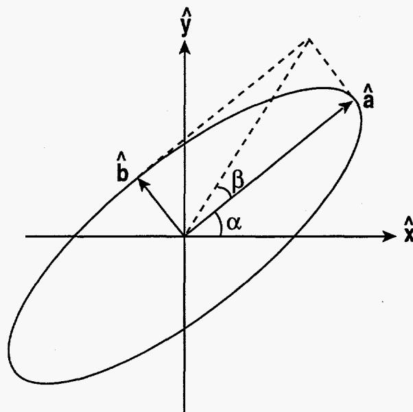
Fig. 5 The parameters of the elliptically polarized rf beam are described by specifying the ratio of the ellipse axes and the tilt angle of the longer axis, indicating the sign of the phase shift between the orthogonal components of the electric field.
