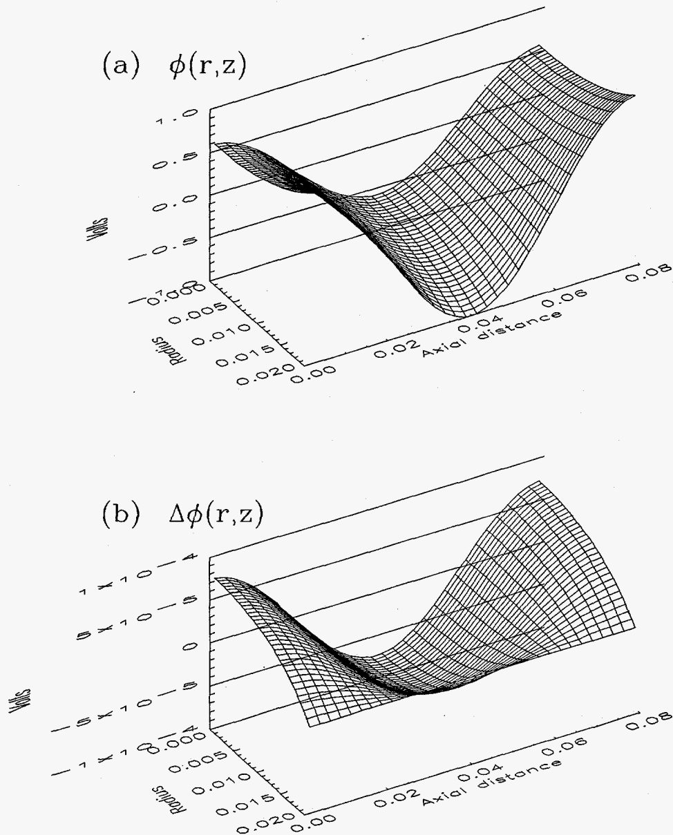
Figure 2: Figure 2(a) shows a plot of \phi(r,z) in Eq. (24) with V_0 = 1V , R_{wall} = 0.02m and L = 0.08m . Figure 2(b) shows the difference between the potential calculated using the Poisson solver and by using Eq. (24).
