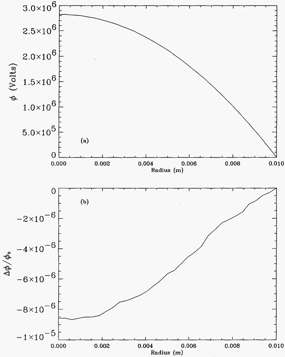
Figure 1: Figure 1(a) shows a plot of \phi(r) obtained from Eq. (23). Figure 1(b) shows the difference between the potential calculated using the Poisson solver and by using Eq. (23) normalized to the theoretical potential at r = 0 .
