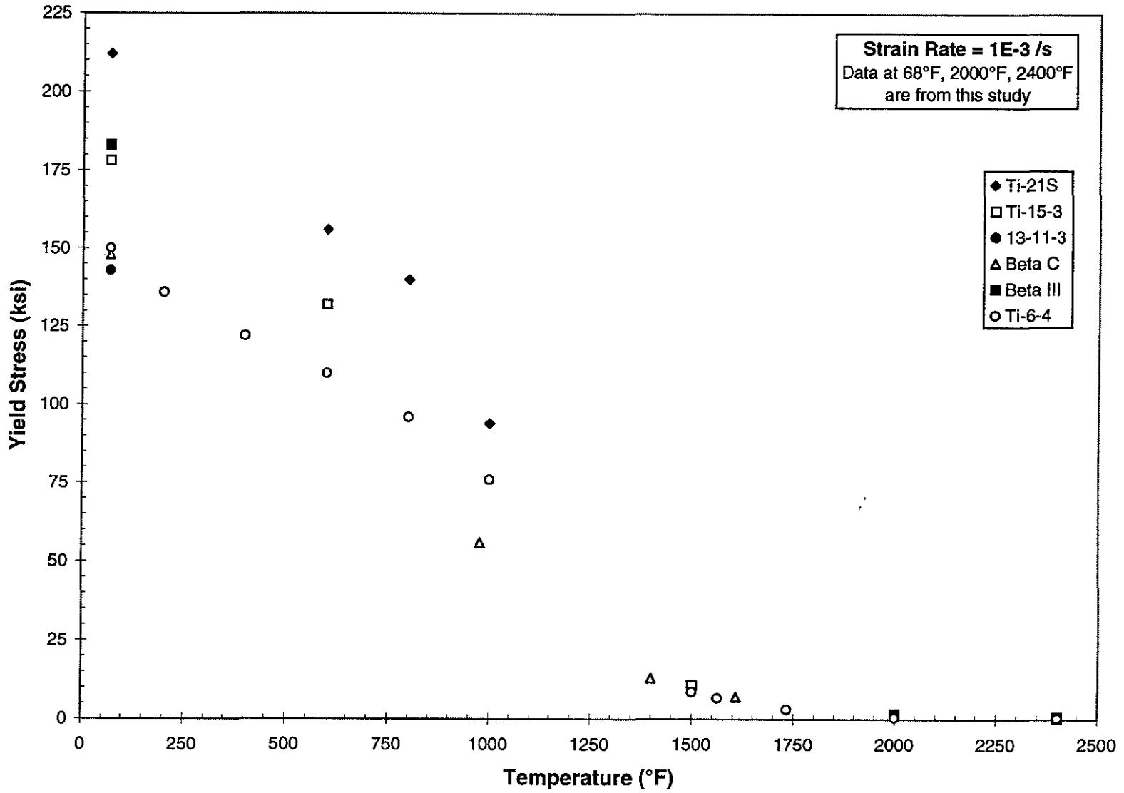
FIGURE 4a. VARIATION IN YIELD STRESS OF TITANIUM ALLOYS WITH TEMPERATURE
