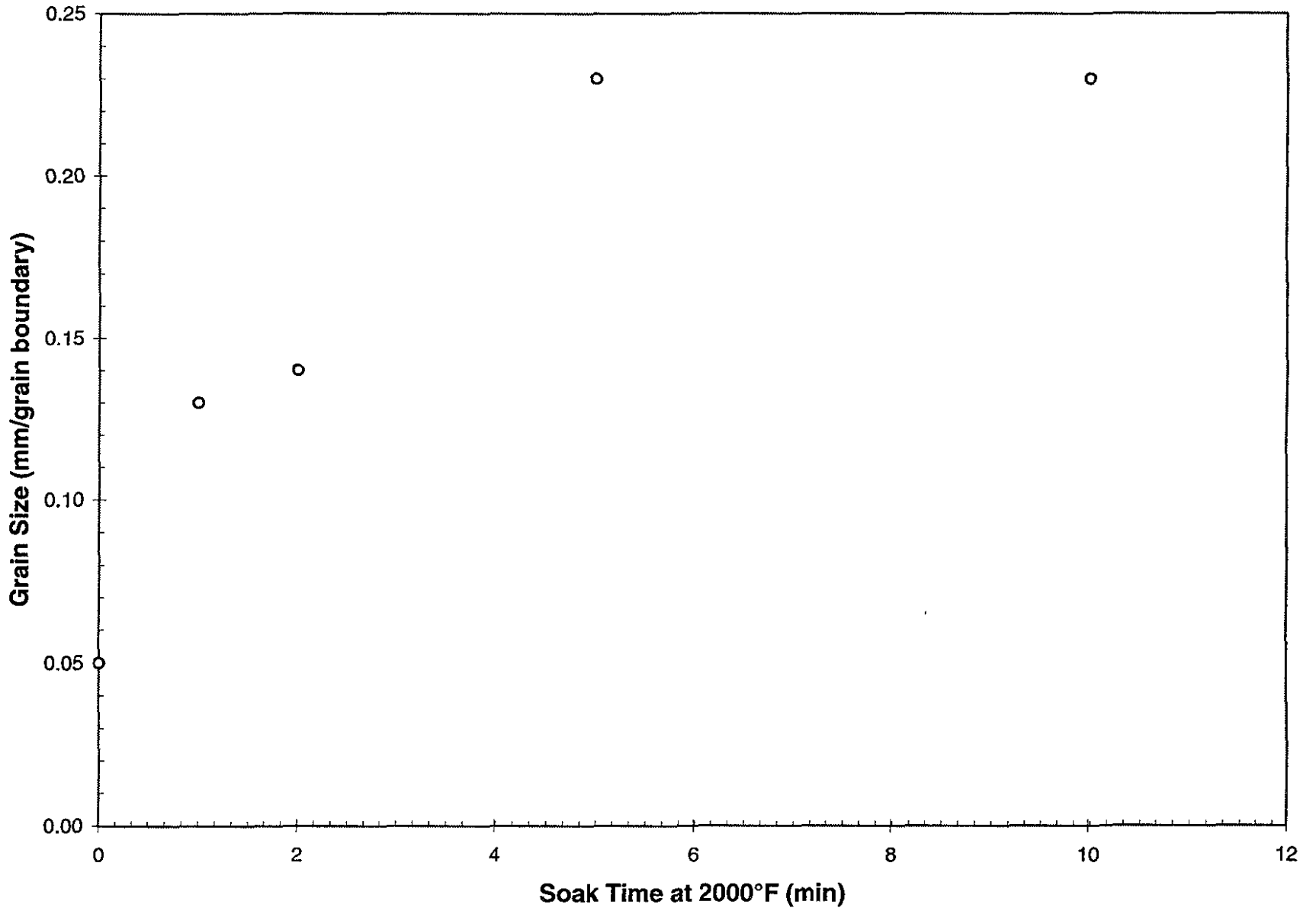
FIGURE 3. INCREASE IN GRAIN SIZE OF Ti-15-3 WITH SOAK TIME AT 2000°F
