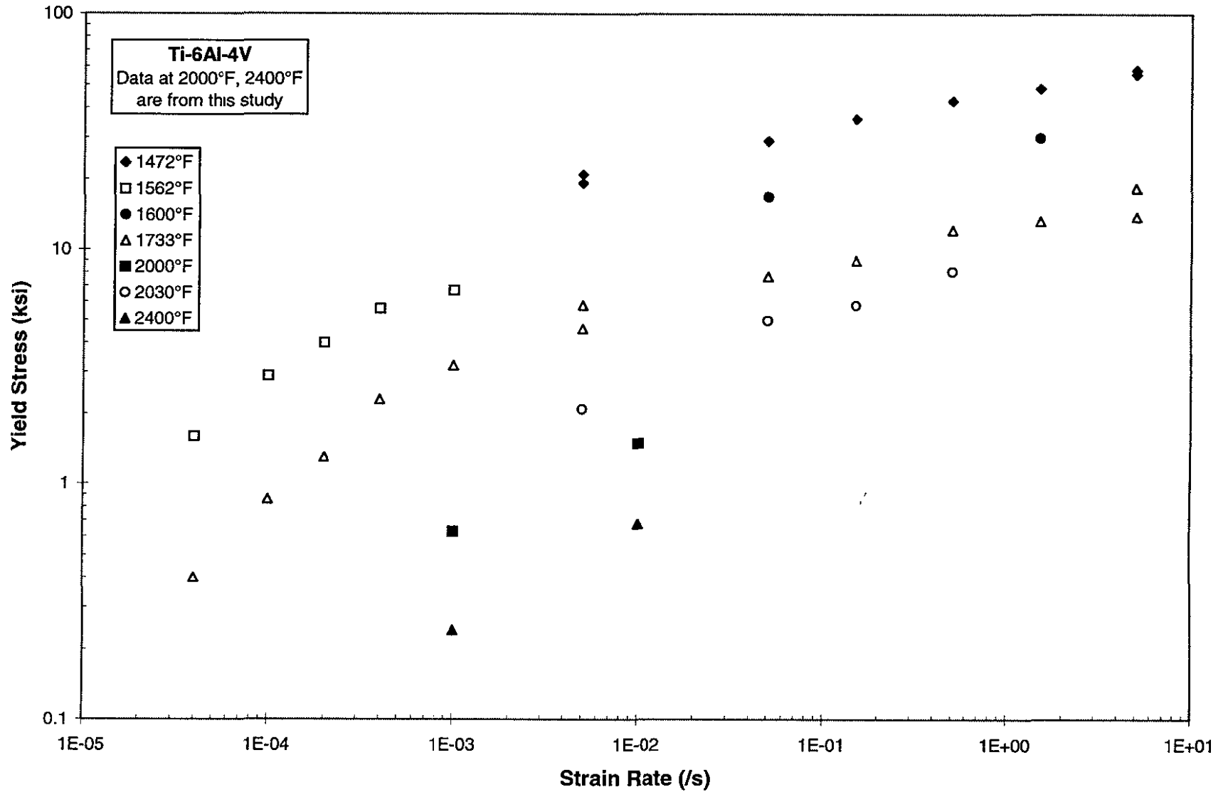
FIGURE 5. VARIATION IN YIELD STRESS OF Ti-6-4 WITH STRAIN RATE
