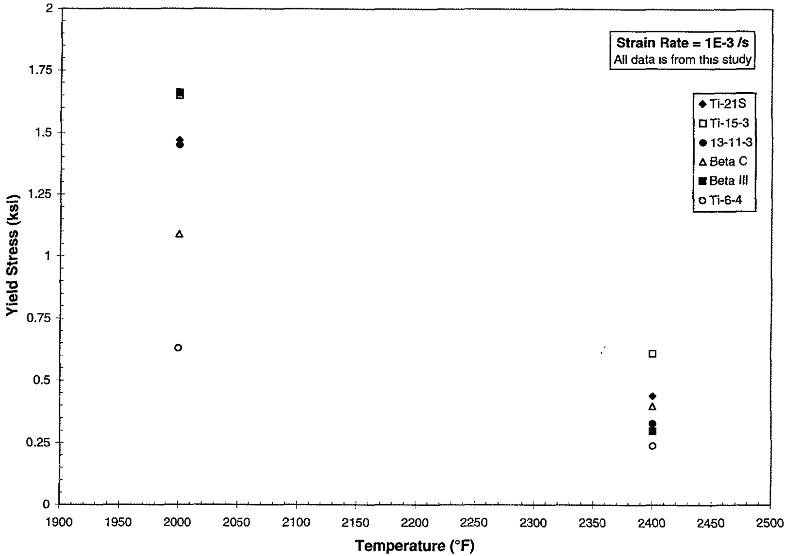
FIGURE 4b. YIELD STRESS OF TITANIUM ALLOYS AT VERY HIGH TEMPERATURES
