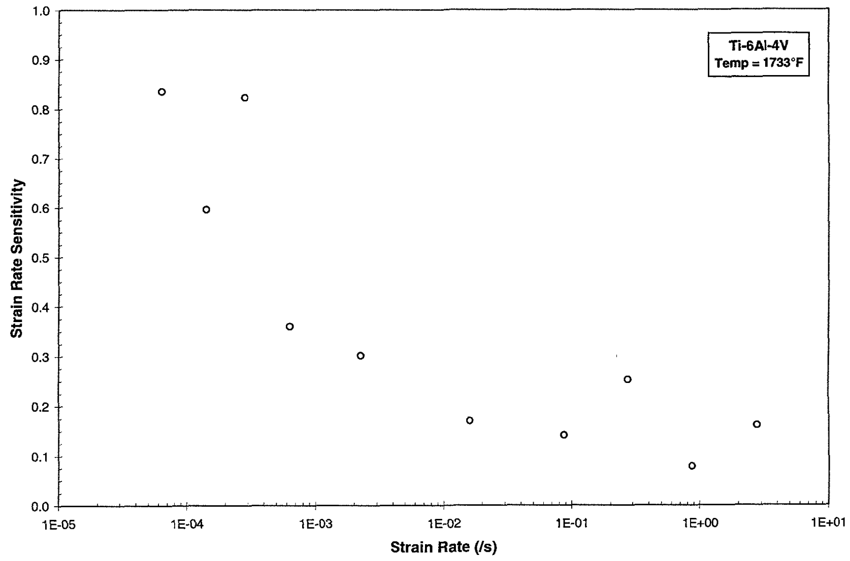
FIGURE 6a. VARIATION IN STRAIN RATE SENSITIVITY OF Ti-6-4 WITH STRAIN RATE
