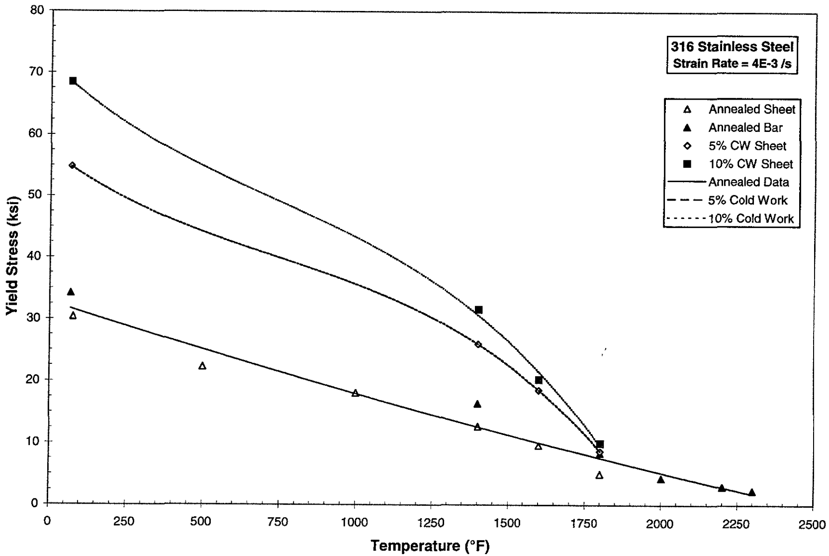
FIGURE 7 VARIATION IN YIELD STRESS OF 316 STAINLESS STEEL WITH TEMPERATURE
