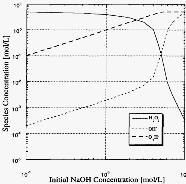
Figure 1. Variation in Equilibrium Concentrations of \text{O}_2\text{H}^- , \text{OH}^- , and \text{H}_2\text{O}_2 for an Initial 5.0\text{M H}_2\text{O}_2 and Variable Initial NaOH Concentrations
