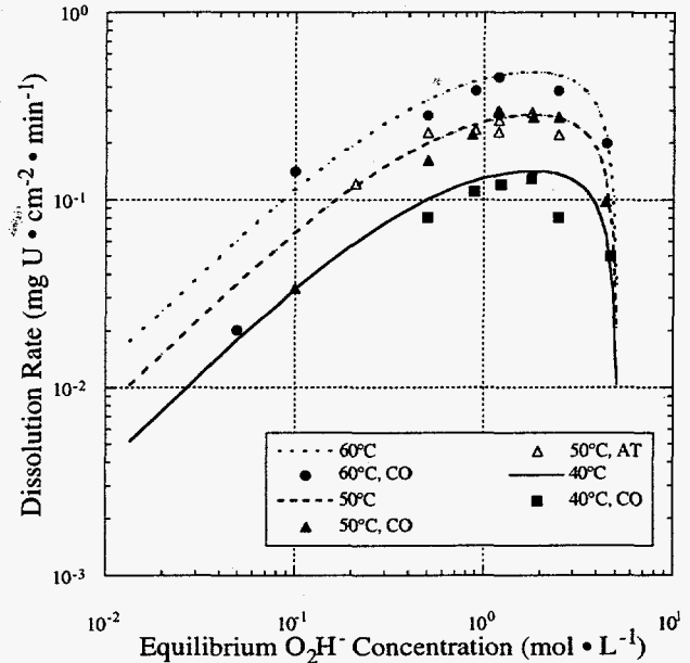
Figure 2. Variation of Uranium Dissolution Rate with Equilibrium Peroxy Ion Concentration. Data points are denoted by dissolution temperature and particle type, (CO or AT); empirical model curves are denoted by temperature only.
