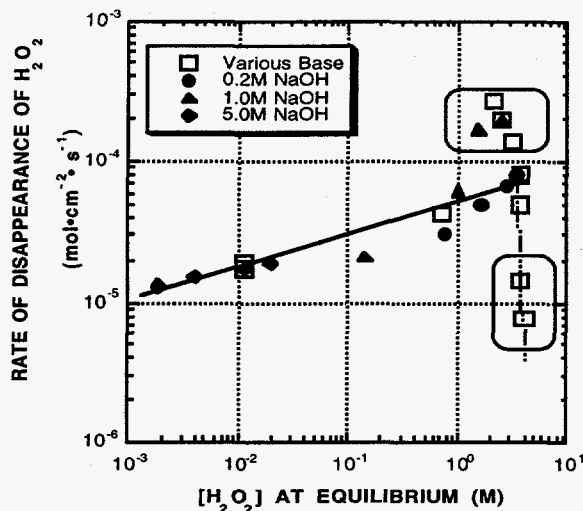
Figure 3. Effect of Equilibrium \text{H}_2\text{O}_2 Concentration on its Depletion Rate at 60^\circ\text{C}
