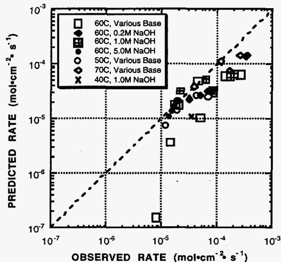
Figure 4. Predicted Rates versus Observed Rates for Depletion of \text{H}_2\text{O}_2
