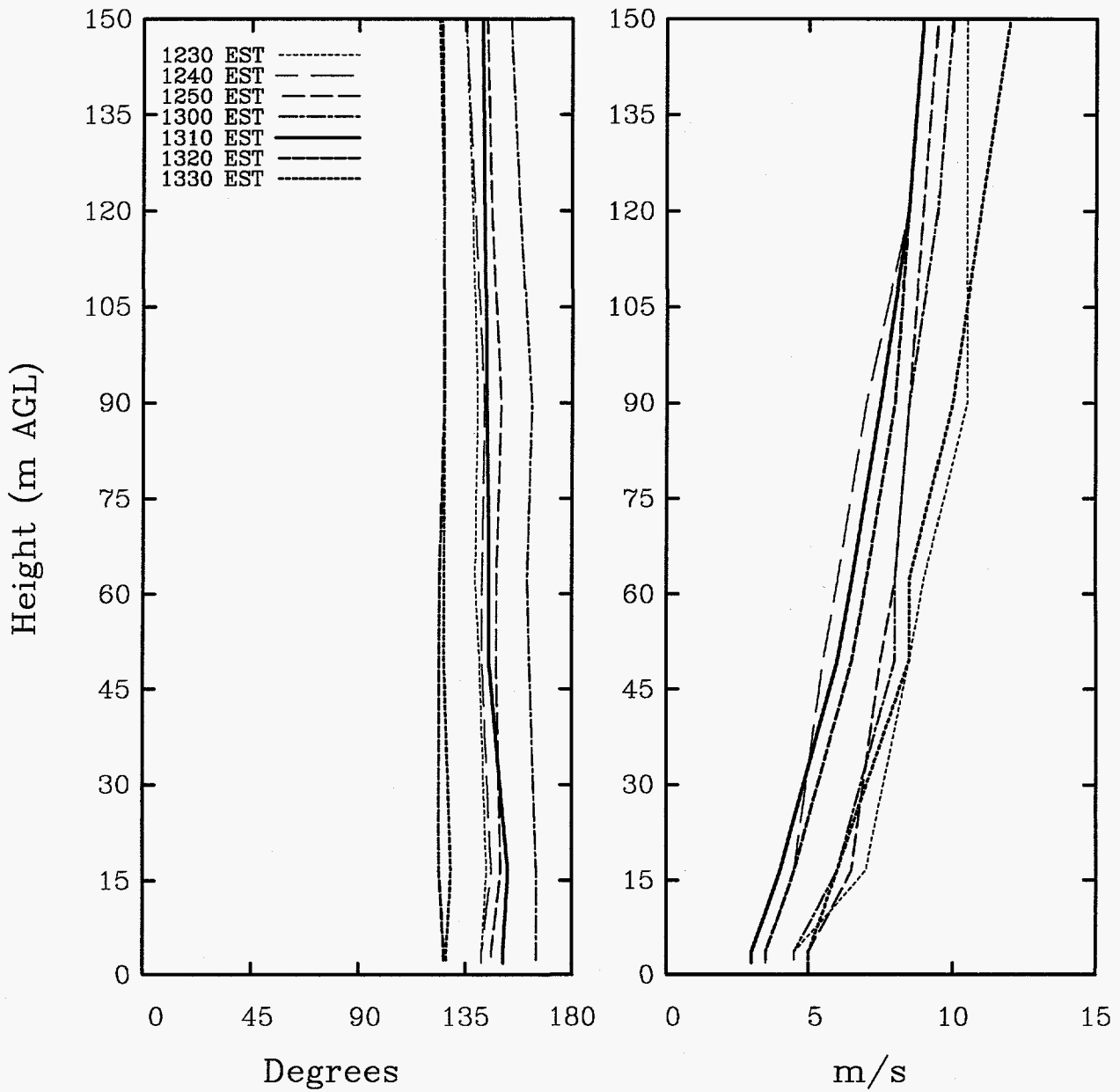
(a) CCAFS/KSC WIND TOWER DATA 4/11/97
