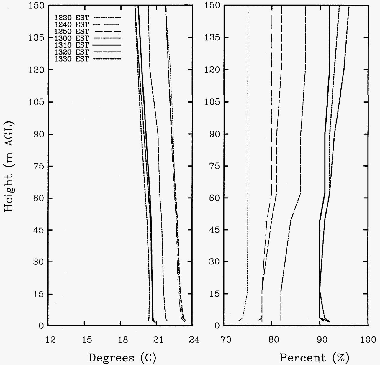
(b) CCAFS/KSC WIND TOWER DATA 4/11/97
