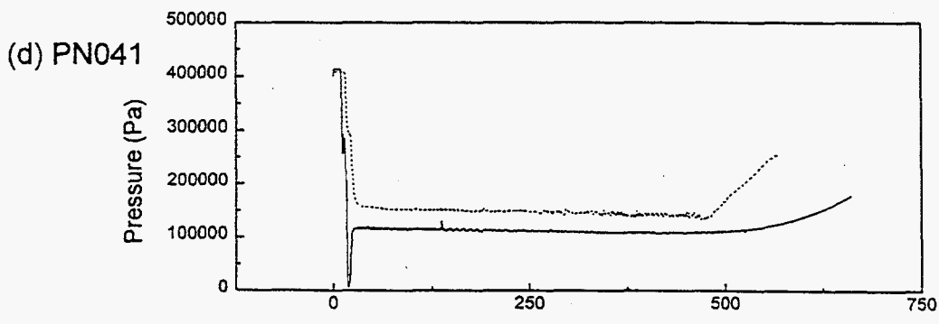
Figure 3.3: Comparison of the test section pressure between experiments and calculation
