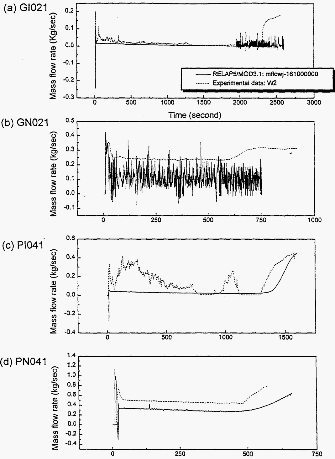
Figure 3.6: Comparison of the injection flow rate between experiments and calculation
