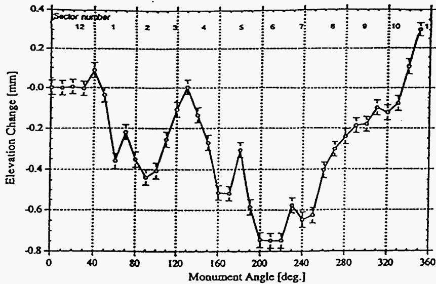
Figure 6a Storage ring monument elevation changes from Feb.1993 to Oct. 1993.
