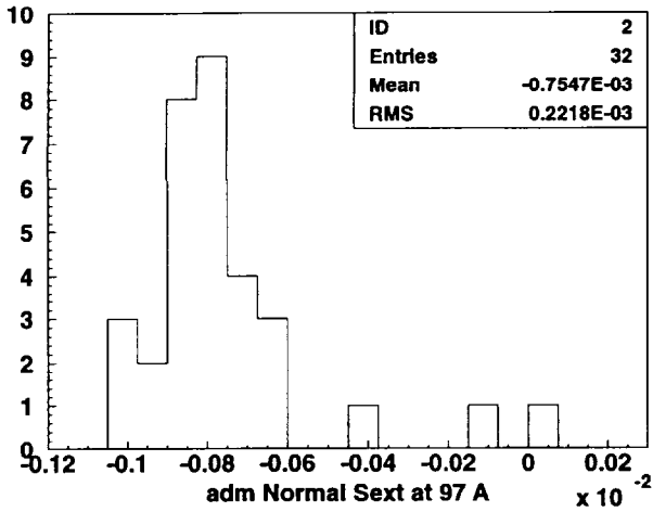
Main Ring Dipole - Sextupole Harmonics
