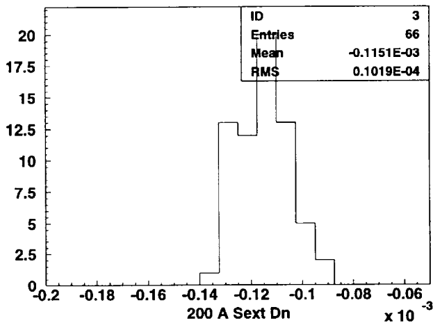
IDC Sextupole Harmonics
