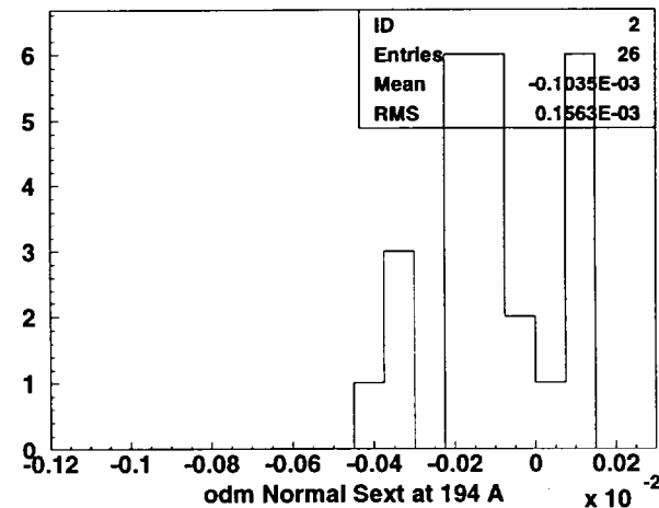
Main Ring Dipole - Sextupole Harmonics
