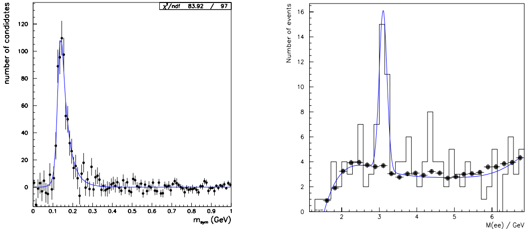
Figure 2: Background-subtracted \pi^0 \rightarrow \gamma\gamma \rightarrow eeee peak, with fit. We measure m_{\pi^0} = 134.5 \pm 10.2 MeV/ c^2 (left). Low- E_T ( E_T^e < 3 GeV/ c ) dielectron invariant mass, showing the J/\psi peak and a fit to the distribution (including background). The measured J/\psi mass is m_{J/\psi} = 3.032 \pm 0.193 GeV/ c^2 (right). (Errors quoted represent both the statistical and systematic contributions added in quadrature.)
