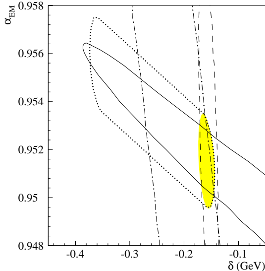
Figure 3: Constraints on the scale factor \alpha and intercept \delta from observed J/\psi \rightarrow ee (dashed-dotted line), \pi^0 \rightarrow \gamma\gamma (dashed line), and Z \rightarrow ee decays (solid line). The shaded inner contour shows the combined result. The dotted line indicates the allowed area when nonlinear terms, constrained from test beam measurements, are included.
