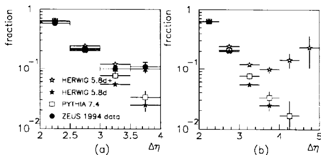
Figure 6: Gap fractions for ZEUS 1994 data, compared with Monte Carlo model predictions: (a) is for a standard detector, compared to the ZEUS data; (b) is for an extended detector at HERA. Similar results might be expected for a detector at higher center of mass energies.
