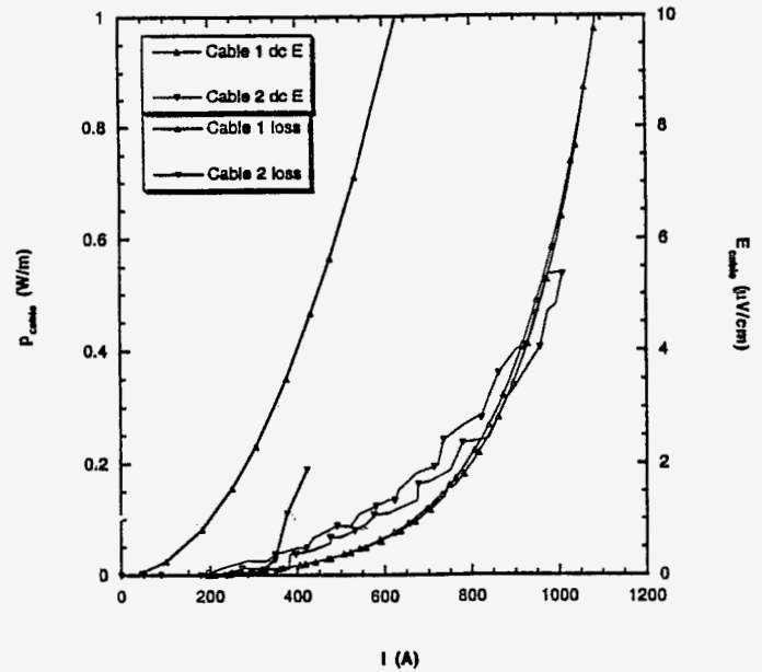
Fig. 7 AC losses of both cable#1 and #2 in reference to their DC I-E curve. RMS current is plotted for the AC current.
