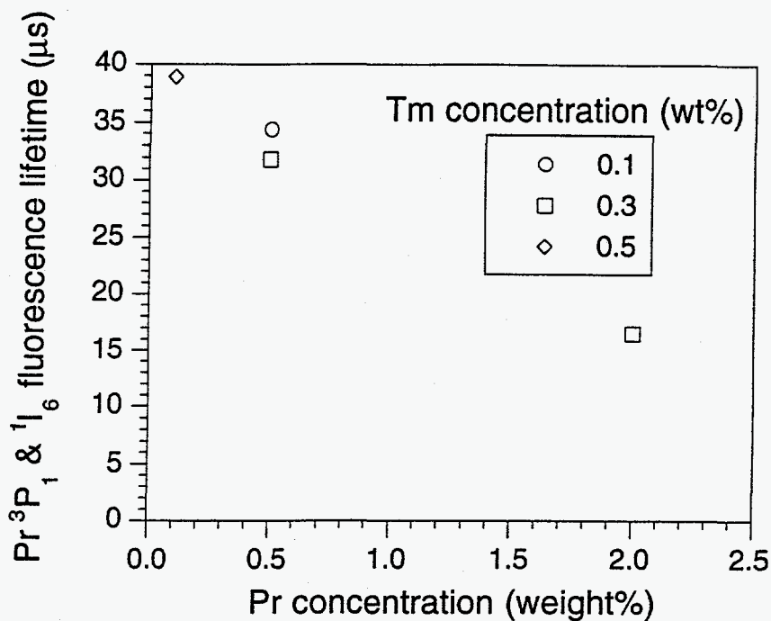
Figure 5. The Pr 3+ ³P 1 and ¹I 6 levels were excited at 468 nm and emission was monitored at 520 nm (³P 1 → ³H 5 ). The data shown is an average of five data points taken for each sample.
