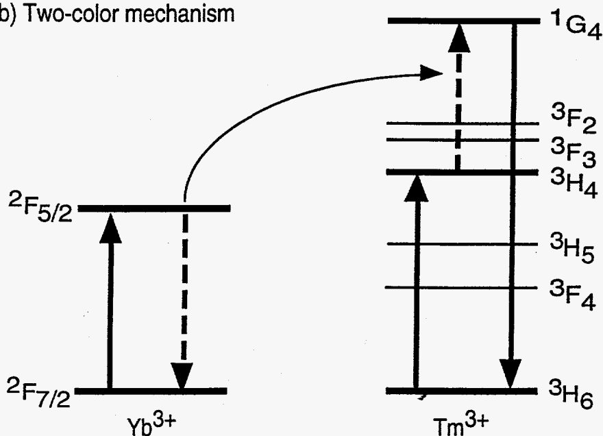
Figure 9. The top drawing (a) shows a sequential three-step energy transfer from \text{Yb}^{3+} to \text{Tm}^{3+} resulting in population of the \text{Tm}^{3+} 1G_4 level (the one-color mechanism). The \text{Yb} ions can be pumped anywhere in the 915-982 nm range. The lower drawing (b) shows a one-step energy transfer from \text{Yb}^{3+} to \text{Tm}^{3+} that also results in population of the \text{Tm}^{3+} level. This (two-color) mechanism requires direct excitation of both \text{Yb}^{3+} and \text{Tm}^{3+} at approximately 975 nm and 785 nm respectively.
