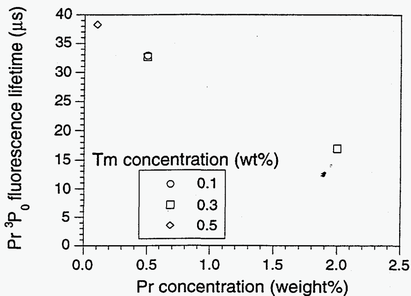
Figure 6. The Pr 3+ ³P 0 level was excited at 468 nm (presumably indirectly by energy transfer from the Pr 3+ ³P 1 and ¹I 6 levels or by energy transfer from the Tm 3+ ¹G 4 state) and emission monitored at 715 nm (³P 0 → ³F 4 ). The data shown is an average of five data points taken for each sample.
