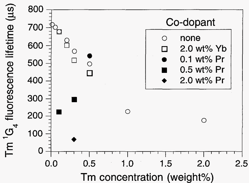
Figure 3. The Tm^{3+} \ ^1G_4 level was excited at 468 nm. Emission from the Tm only and Yb co-doped samples was monitored at 642 nm ( ^1G_4 \rightarrow ^3F_4 ), while emission from the Pr co-doped samples was monitored at 788 nm ( ^1G_4 \rightarrow ^3H_5 ). The data shown is an average of five data points taken for each sample.
