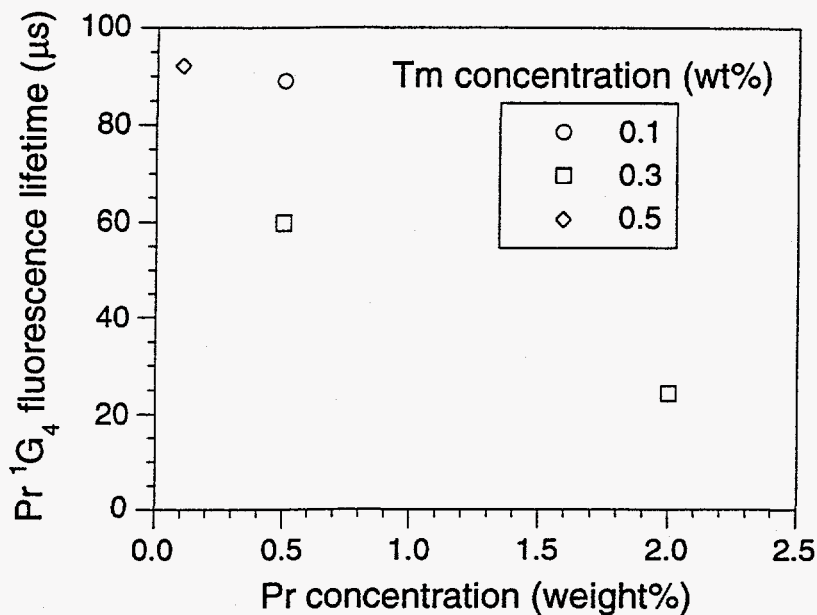
Figure 7. The Pr 3+ 1 G 4 level was excited at 1010 nm and emission was monitored at 1313 nm ( 1 G 4 → 3 H 5 ). The data shown is an average of five data points taken for each sample.
