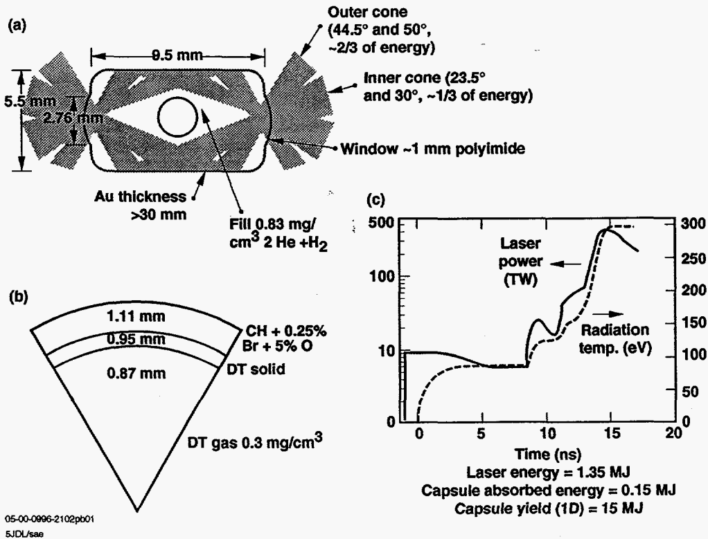
Fig. 2 Most of the LASNEX integrated modeling and detailed analysis of Rayleigh-Taylor instability has concentrated on a target, called the PT, which absorbs about 1.3 MJ of 0.35 μm laser light.
