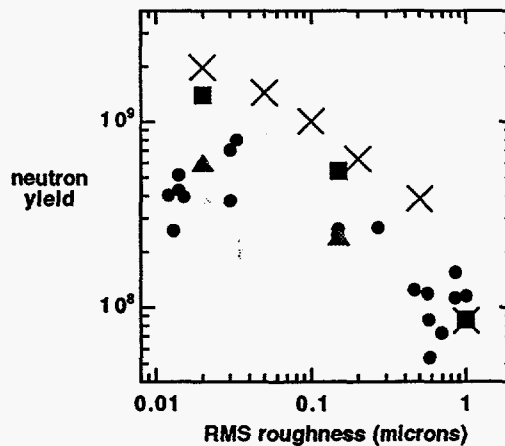
Fig. 11 Solid circles show experimental yields of Nova capsules having multimode perturbations of various amplitudes. The crosses indicate yields from the 1-D mix model. The solid squares are from 3-D HYDRA simulations, including drive asymmetry. The triangles represent simulations which also include low mode thickness variations.
