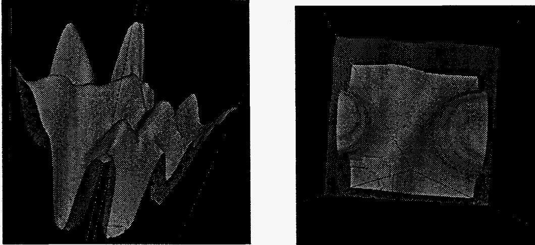
Fig. 9 Iso-density contour surfaces near ignition time for a PT capsule simulation containing modes with l=15-120 . (a) 130 \text{ g/cm}^3 surface just inside the DT-ablator interface (b) 650 \text{ g/cm}^3 surface at pusher-hot spot interface seen from the inside.
